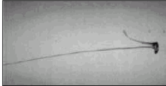
Figure 5. Liquid breakup using 3.8%PSBMA (M.W. 2,270,000)+TBP, d=1.9 mm, We=30 .
