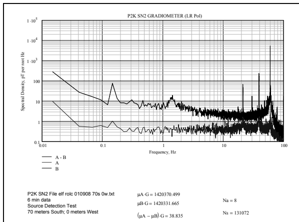
Figure 6. Upper left plot is background environmental noise. Upper right plot is magnet rotation measurement 30 meters to South of sensor. Lower left is 70 meters and lower right plot is 100 meters South of P-2000 gradiometer.
