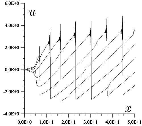
Figure 4. Speed distributions over height for several times for one-dimensional heating (units are dimensionless).
