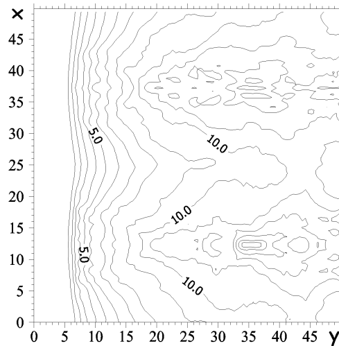
Figure 8. Maximal over period temperature for atmosphere, heated by non-uniform wave's source (units are dimensionless).
