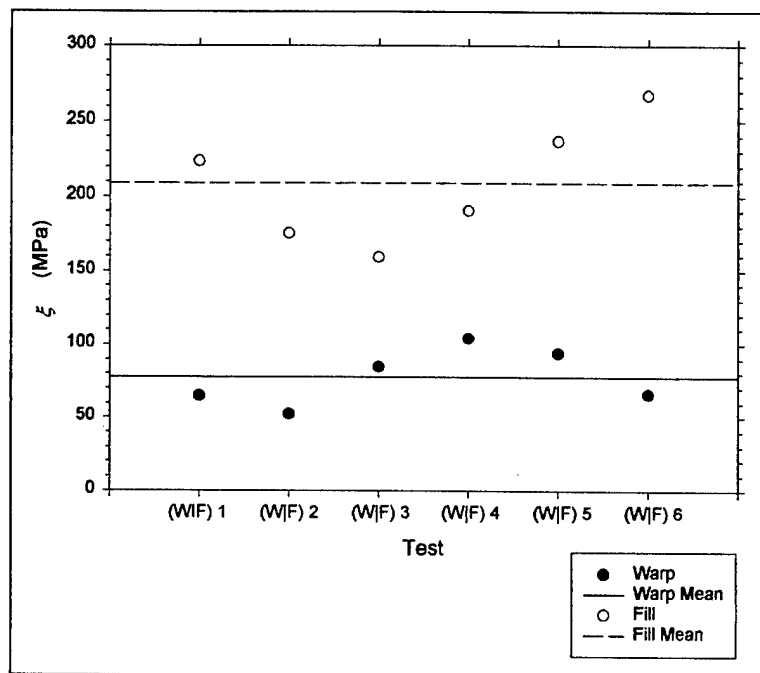
Figure 24. Characteristic-stress parameter of the exponential fit to the fabric stress-crosshead displacement results from each of the 12 tests.
