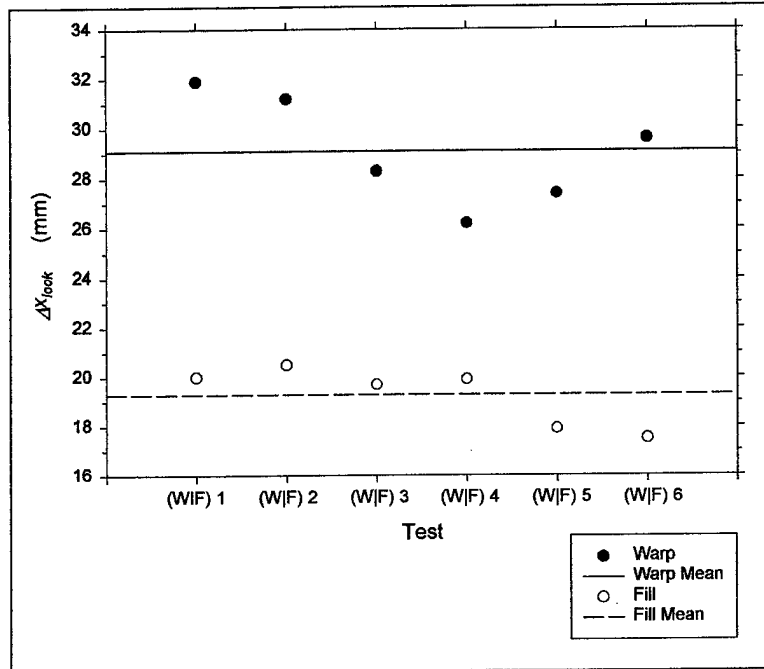
Figure 20. The locking displacement of the bilinear fit to the fabric stress-crosshead displacement results from each of the 12 tests.
