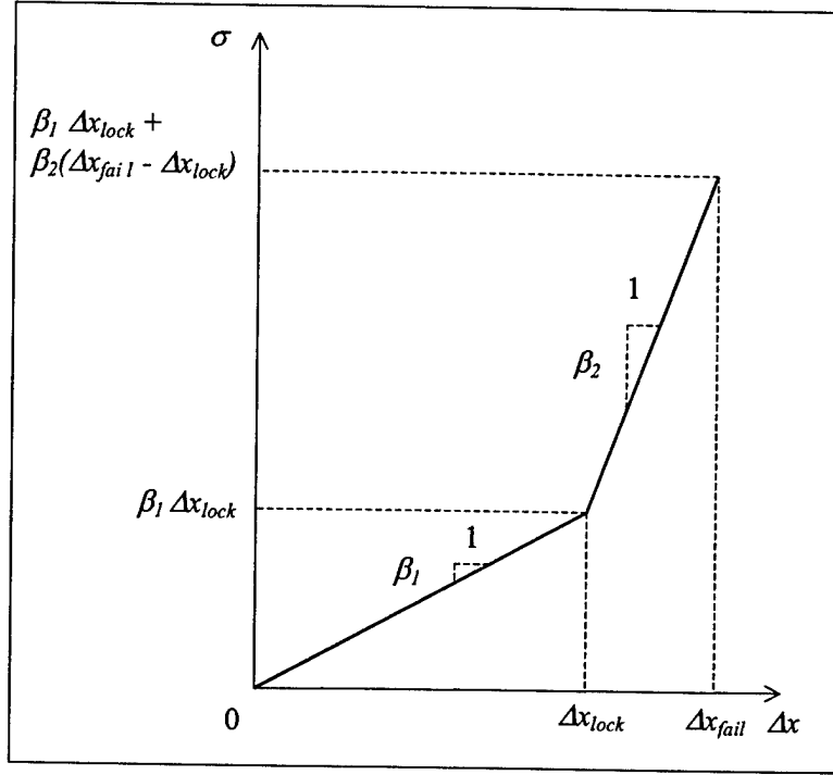
Figure 16. The bilinear fabric stress-crosshead displacement curve of equation 3.
