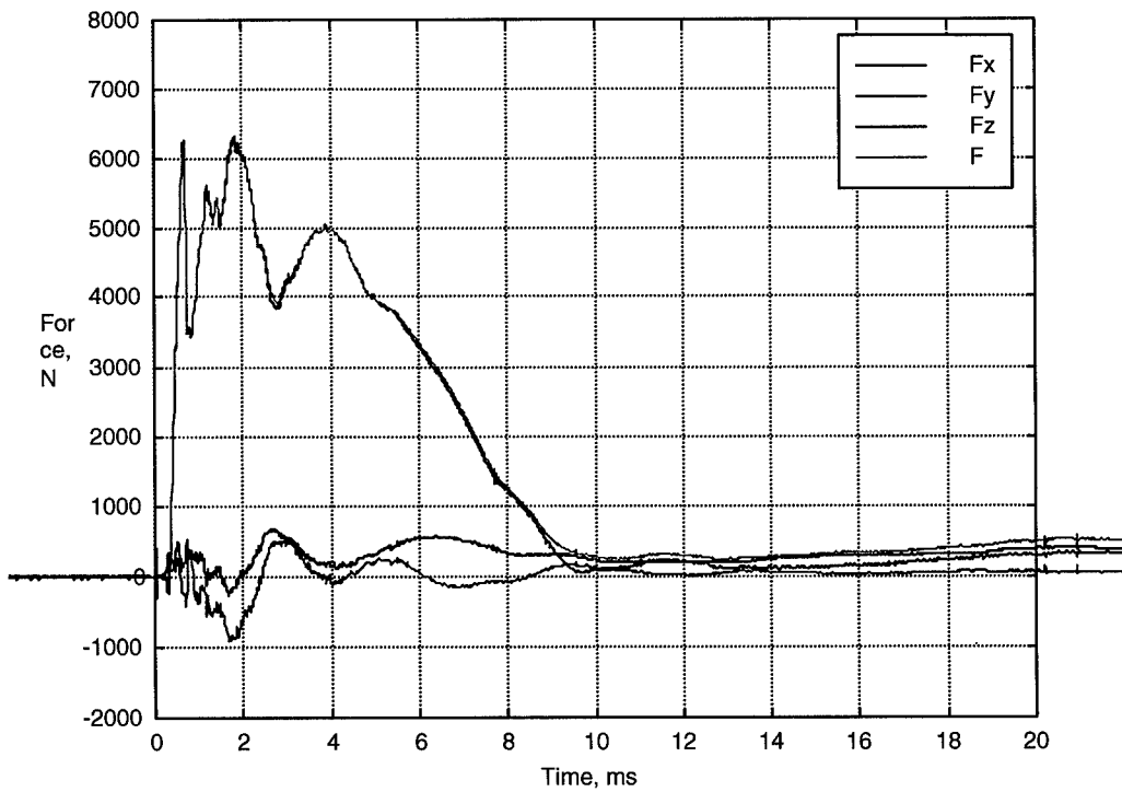
Figure 2: Force data for experiment 5.
