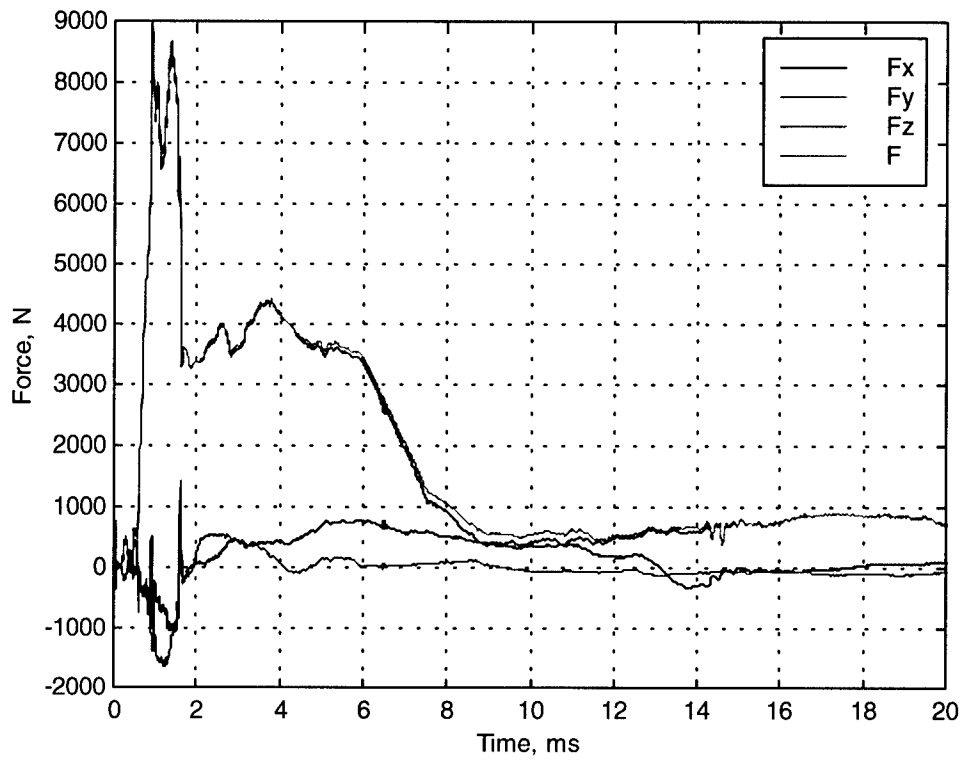
Figure 3: Force data for experiment 6.
