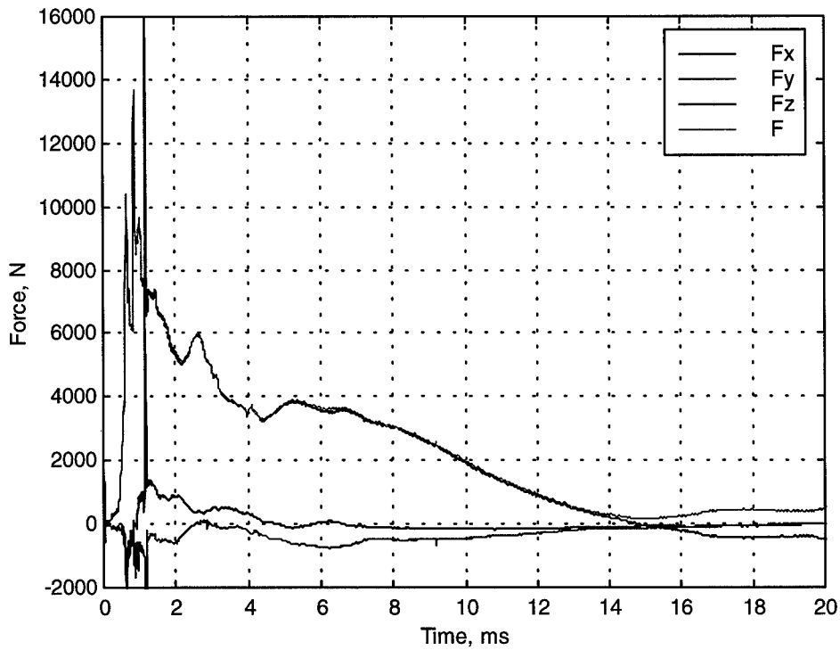
Figure 6: Force data for experiment 10.
