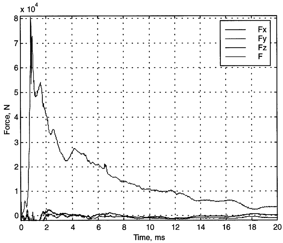
Figure 5: Force data for experiment 8.
