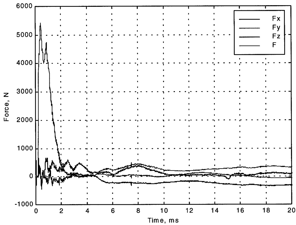
Figure 1: Force data for experiment 1.
