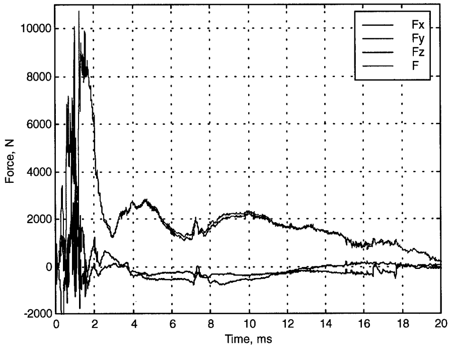
Figure 13: Force data for experiment 25.
