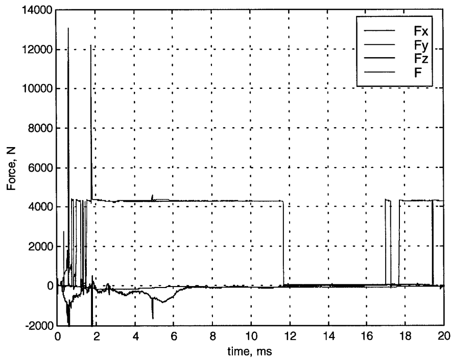
Figure 14: Force data for experiment 26.
