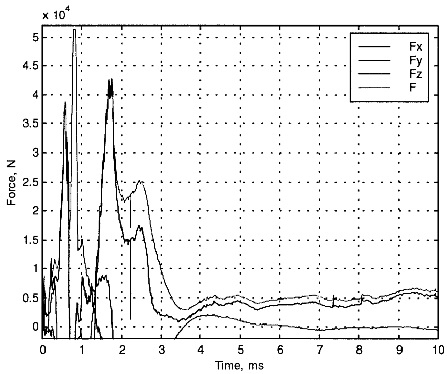
Figure 8: Force data for experiment 15.
