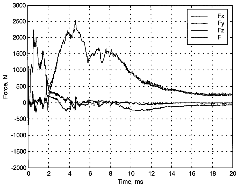
Figure 10: Force data for experiment 19.
