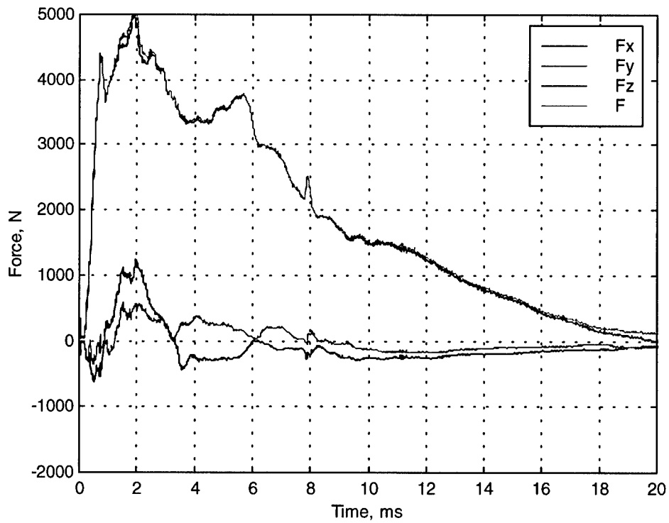
Figure 4: Force data for experiment 7.
