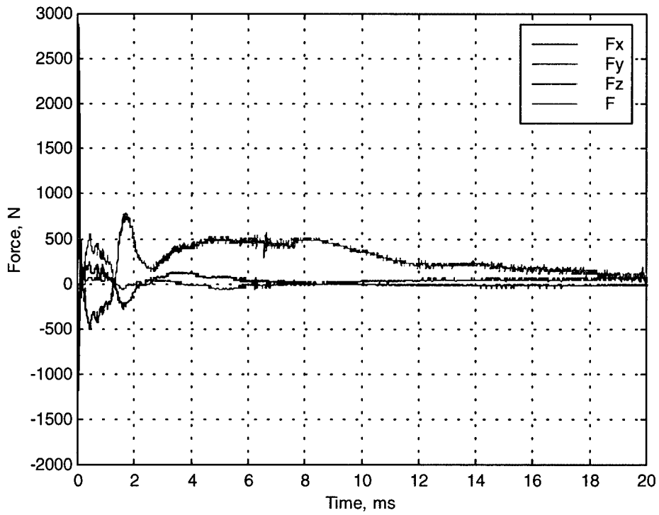
Figure 12: Force data for experiment 21.
