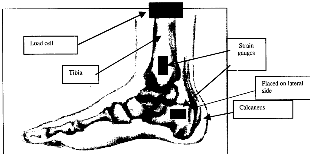
Figure 4: Instrumentation Placement
