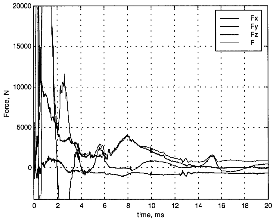
Figure 9: Force data from experiment 18.
