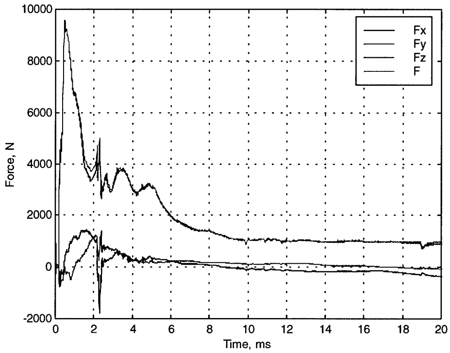
Figure 11: Force data for experiment 20.
