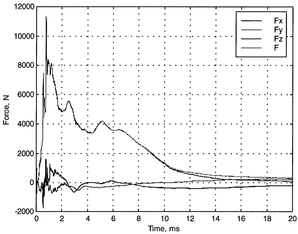
Figure 7: Force data for experiment 12.
