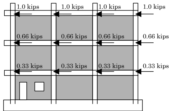
Figure A.7. Pushover Case II.
