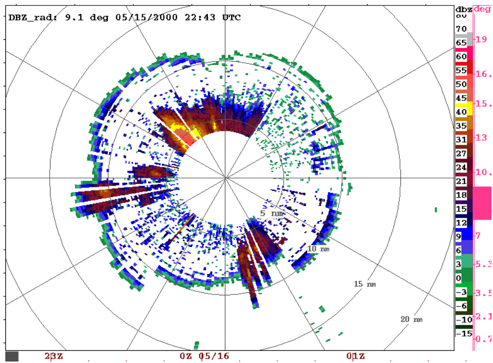
Figure 4-15: TEP Reflectivity Plot (9.1° elevation) for 22:43Z on 15 May 2000 (notice upper level of intense storm at 315°, body of storm within first range gate)
