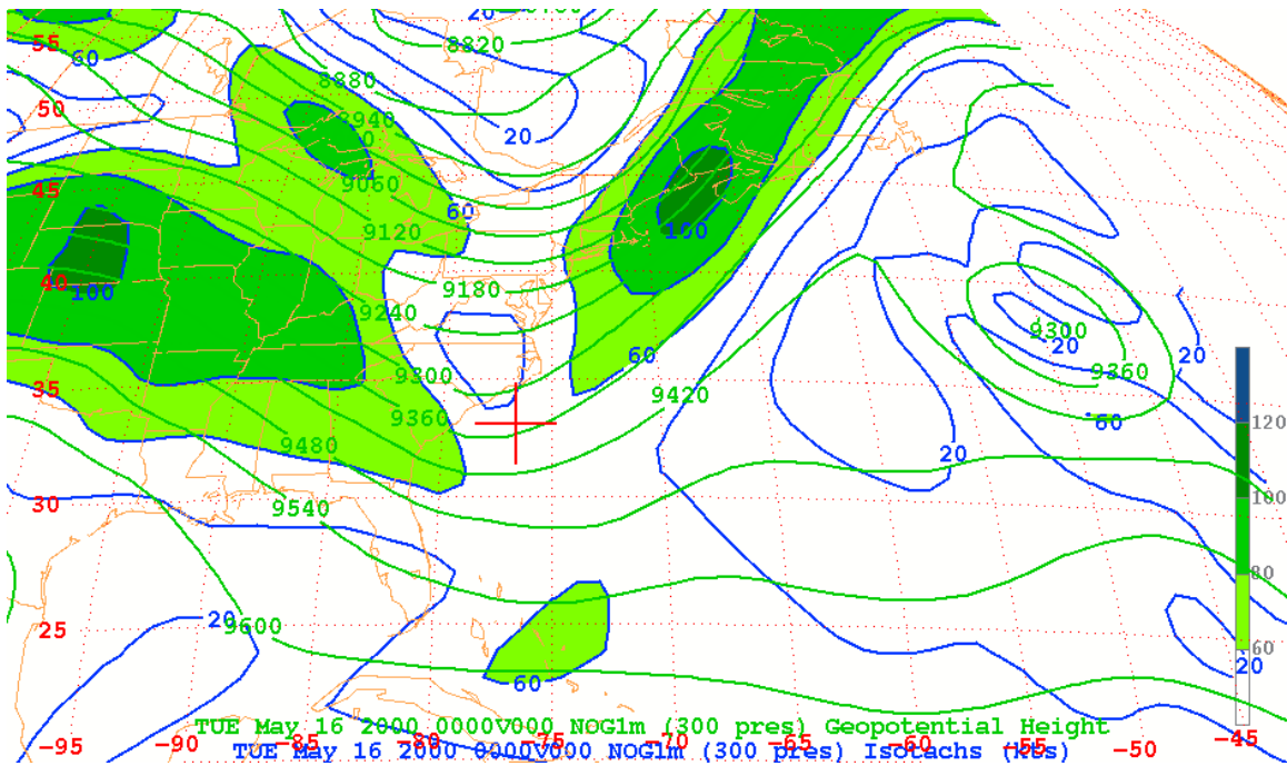
Figure 4-2: 16/00 300mb Heights and Isotachs (red cross-hair represents center of JTFEX OPAREA)
