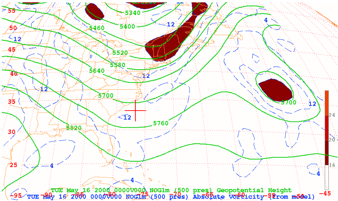
Figure 4-3: 16/00 500mb Heights and Absolute Vorticity (red cross-hair represents center of JTFEX OPAREA)
