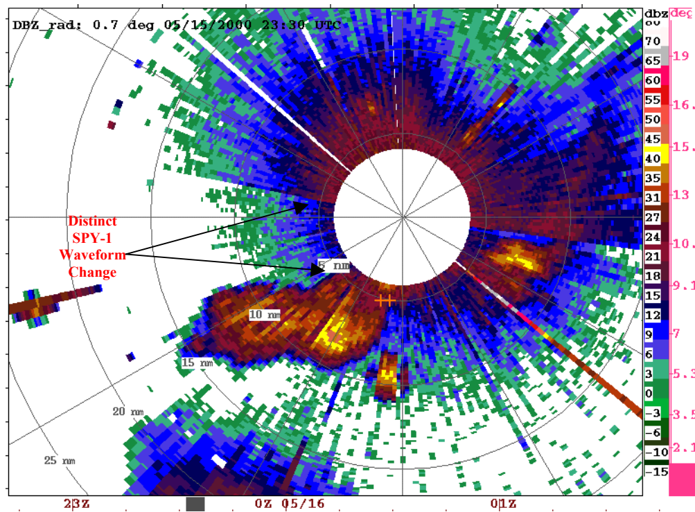
Figure 4-19: TEP Reflectivity Plot for 23:30Z on 15 May 2000 (distinct SPY-1 waveform or power change between 240^{\circ} and 280^{\circ} )
