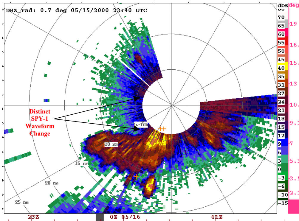
Figure 4-20: TEP Reflectivity Plot for 23:40Z on 15 May 2000 (SPY-1 waveform between 240^{\circ} and 280^{\circ} is still de-sensitized)
