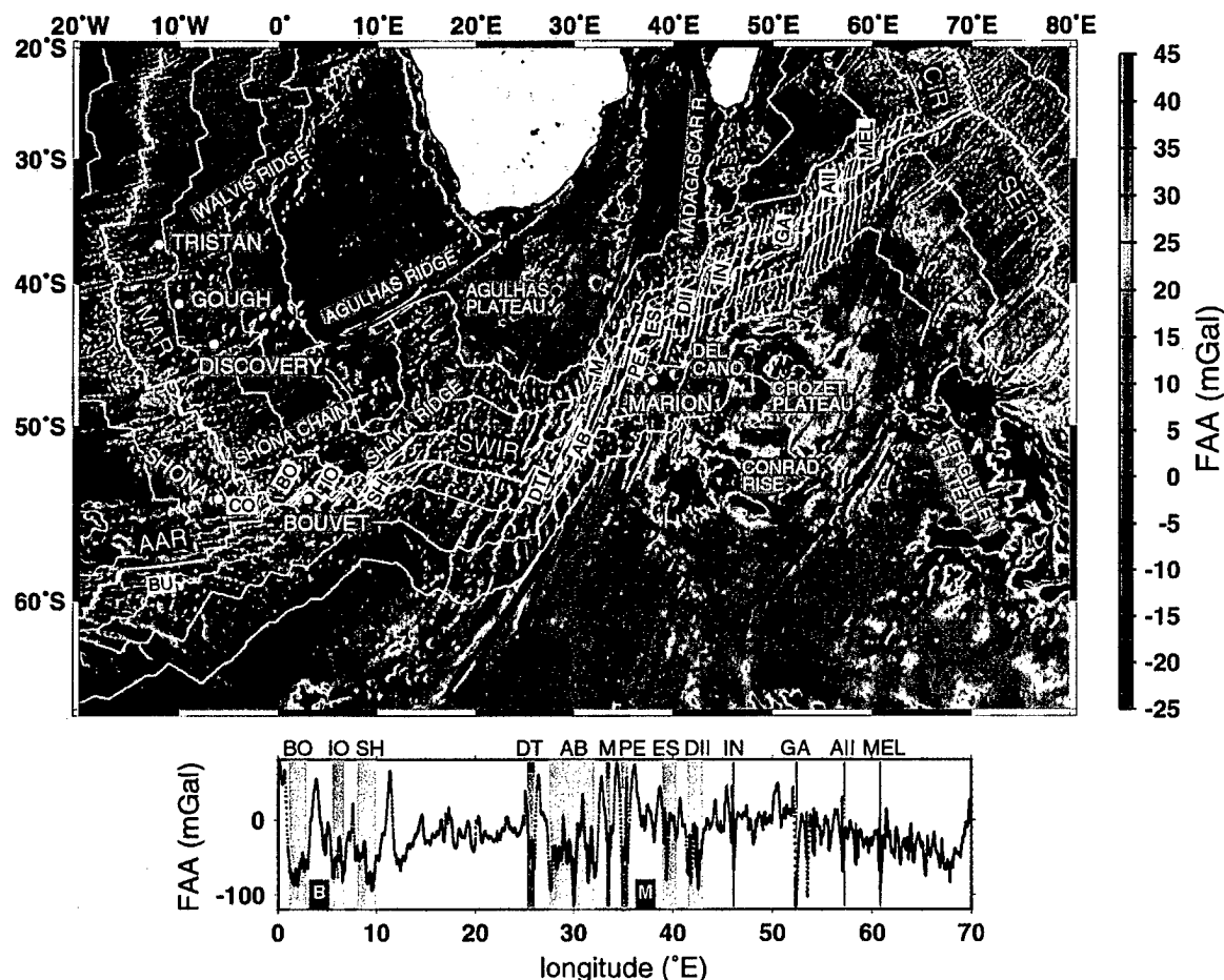
Fig. 1. Regional FAA map for the SWIR and part of the Southern Atlantic Ocean (data from [1]). Thick white lines mark the location of ridge axes: SWIR = Southwest Indian Ridge, SEIR = Southeast Indian Ridge, CIR = Central Indian Ridge, MAR = Mid-Atlantic Ridge, AAR = American–Antarctic Ridge. Locations of significant seafloor features are labeled in white lettering; positions of hotspots are marked with filled white circles. The names of prominent fracture zones are labeled as BU = Bullard FZ, CO = Conrad FZ, BO = Bouvet FZ, IO = Islas Orcadas FZ, SH = Shaka FZ, DT = Du Toit FZ, AB = Andrew Bain FZ, M = Marion FZ, PE = Prince Edward FZ, ES = Eric Simpson FZ, DII = Discovery II FZ, IN = Indomed FZ, GA = Gallieni FZ, AII = Atlantis II FZ, and MEL = Melville FZ. Thin white lines are 25, 50, and 75 Ma isochrons [3]. Gravity data are plotted at 5' spacing and an artificial illumination has been imposed on the grid from the NW. Lower panel shows FAA along the axis of the SWIR. Regions covering fracture zones are shaded, and the positions of the Marion and Bouvet hotspots are indicated with M and B, respectively.
