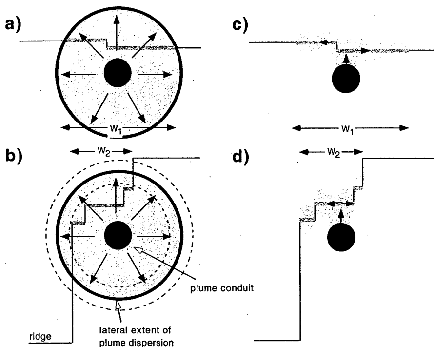
Fig. 11. Schematic cartoons of plume-ridge interaction with a segmented ridge. (a) Broad dispersion of plume material at a depth below the onset of melting, for a ridge with only a single, small transform offset. Dark gray circle represents the plume conduit, light gray shading depicts dispersal of plume material, arrows indicate plume dispersal direction, and thin black lines denote ridge geometry. Ridge segments with a plume signature are emphasized with thick, medium gray shading. The length of ridge affected by plume 1, or waist width, is W_1 . (b) As in (a), but for a highly segmented ridge. Although the plume's lateral extent is the same as in (a), the resulting waist width W_2 is less than W_1 . Note ambiguity in inferring plume dispersion from W_2 , since both smaller (dashed) and larger (dash-dot) circles will produce the same W_2 . (c) Schematic illustration of the channelized along-axis plume dispersion model for the same ridge geometry as in (a). Arrows indicate flow directed from plume to ridge, and subsequent dispersion along-axis, at depths within the partial melting zone. The resulting waist width is W_1 . (d) As for (c), but for a highly segmented ridge. Note that long-offset transforms act as thermal and mechanical barriers and prevent along-axis dispersion, resulting in a W_2 that is less than W_1 .
