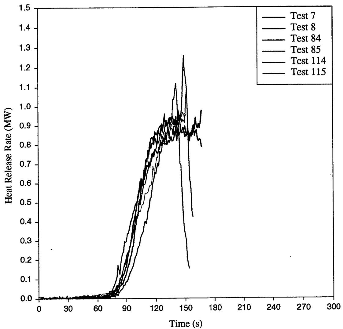
Comparison of heat release rates for Scenario 1, 1.7 Lpm unconfined JP-8 spill fires.
