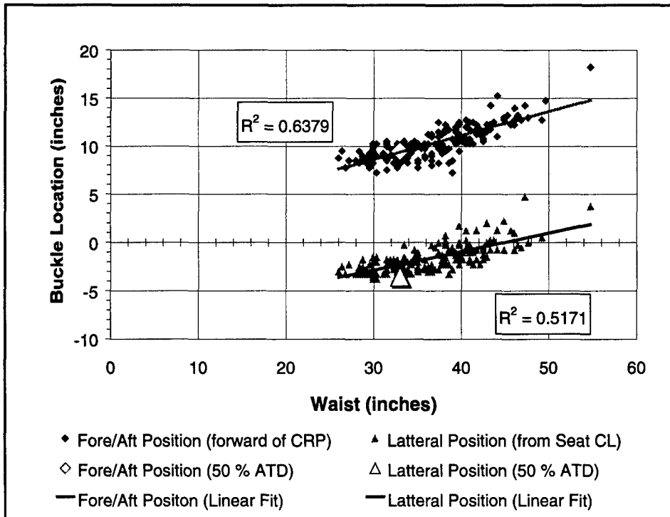
Figure 13. Belt Buckle Location vs. Occupant Girth
