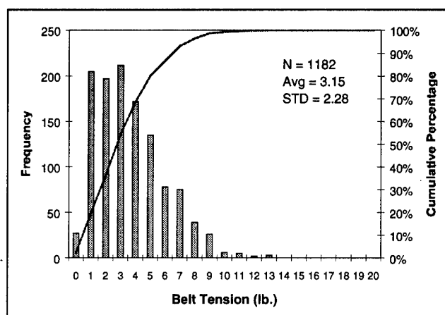
Figure 6. Normal Lap Belt Tension
