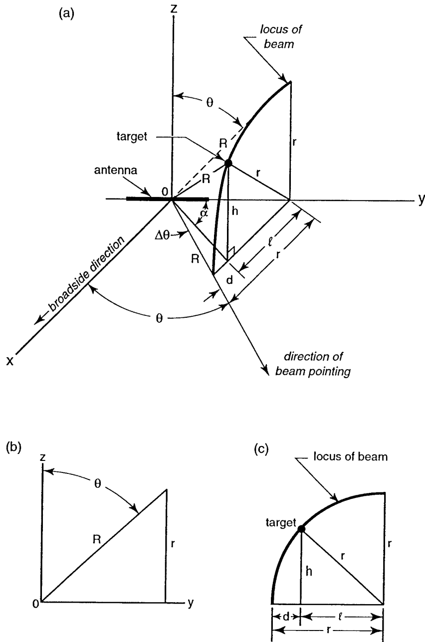
Fig. III-1(a) — Geometry of scanning a beam in azimuth with a linear array antenna. (b) Cut in the y - z plane. (c) Cut in the target plane.
