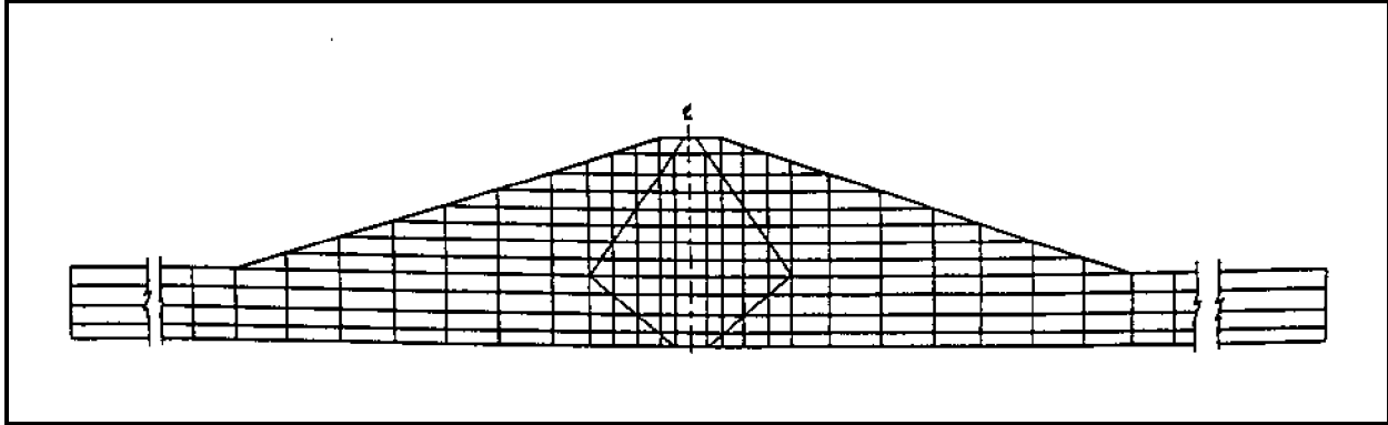
Figure 17. Finite element mesh of Birch Dam
