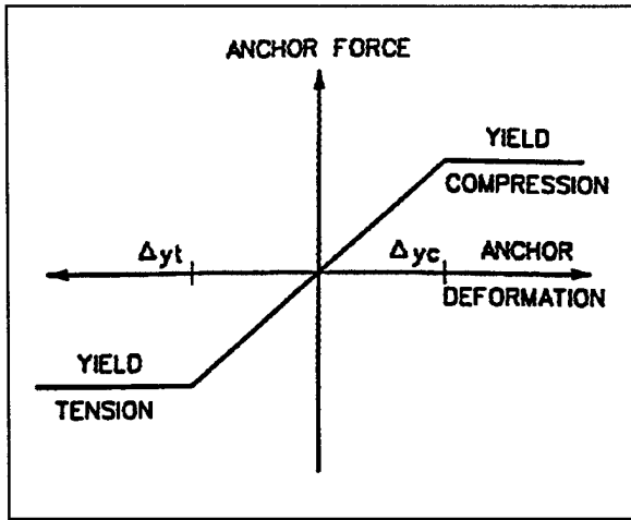
Figure 7-3. Anchor spring
