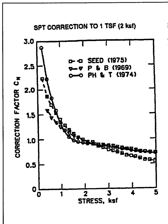
Figure 3-5. SPT correction to 1 tsf
