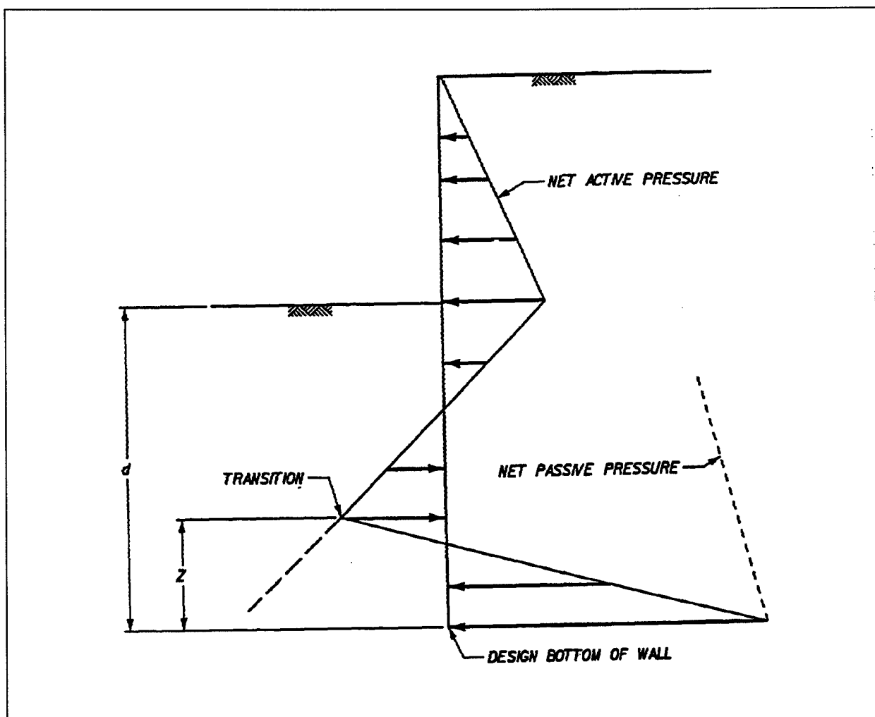
Figure 5-6. Design pressure distribution for cantilever wall
