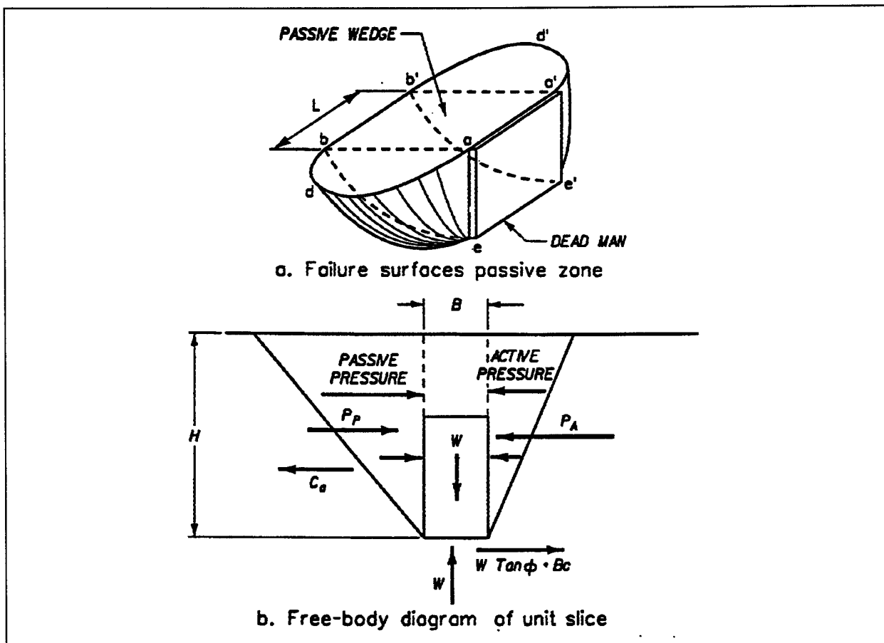
Figure 5-10. Resistance of discontinuous anchor (dead man)
