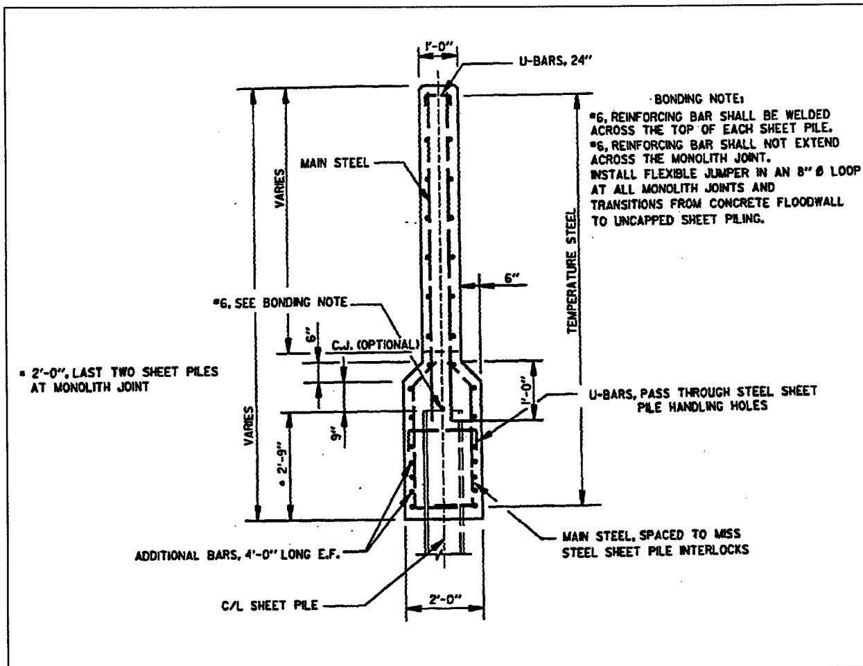
Figure 9-1. Typical section through I-wall of varying thickness
