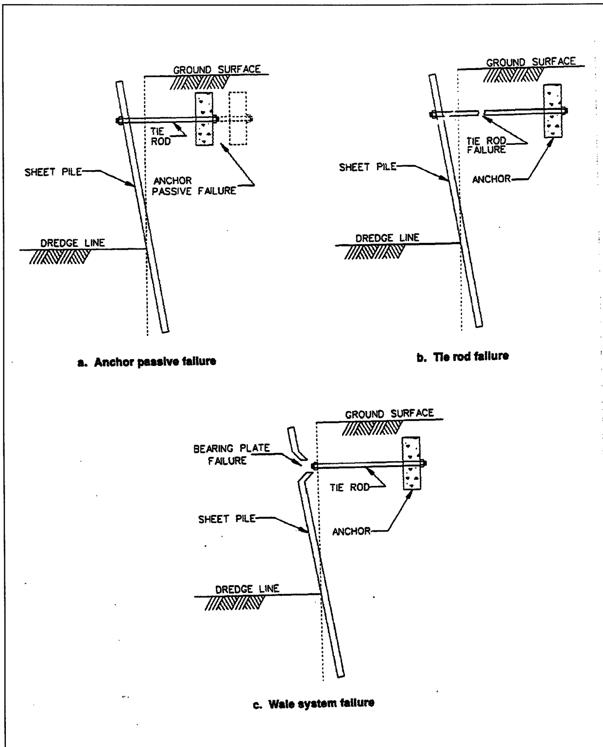
Figure 5-4. Anchorage failures
