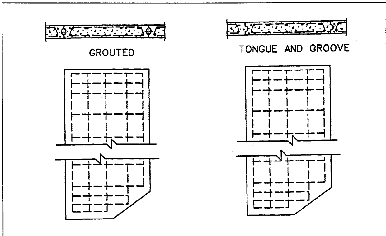
Figure 2-6. Typical concrete sections
