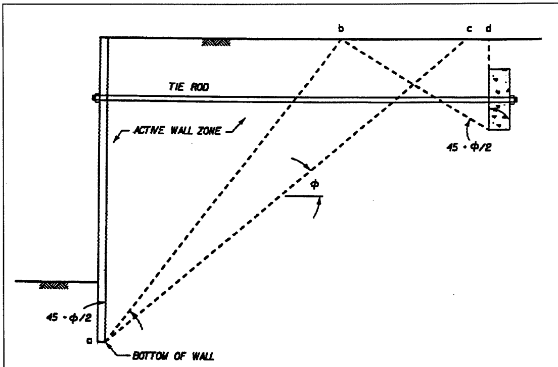
Figure 5-8. Minimum anchor - wall spacing for full passive anchor resistance in homogeneous soil
