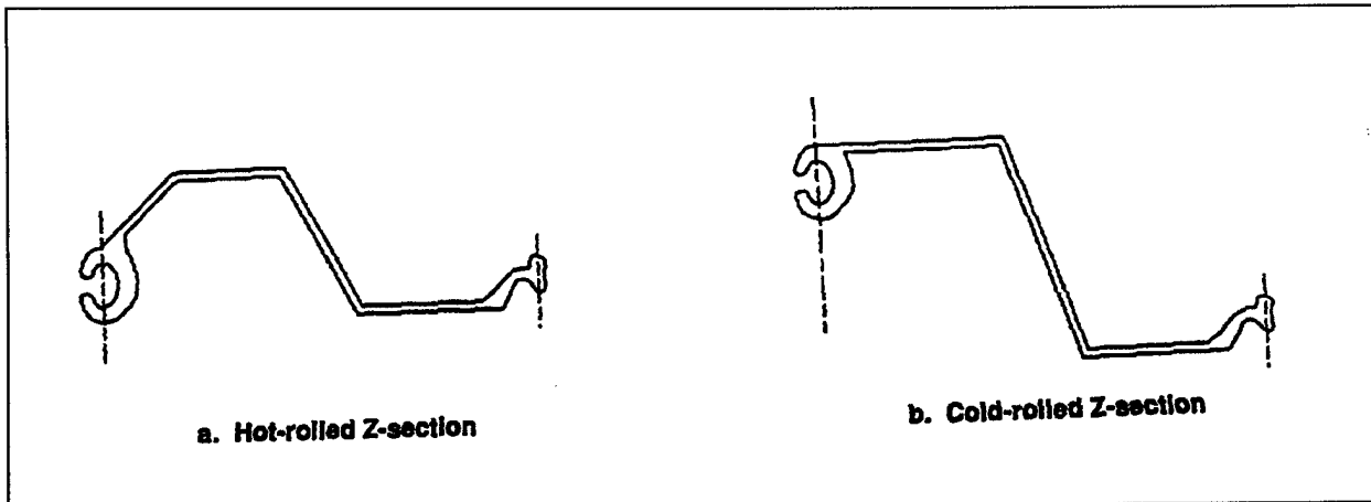
Figure 2-7. Typical aluminum sheet piling
