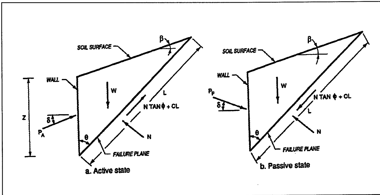
Figure 4-4. Soil wedges for Coulomb earth pressure theory
