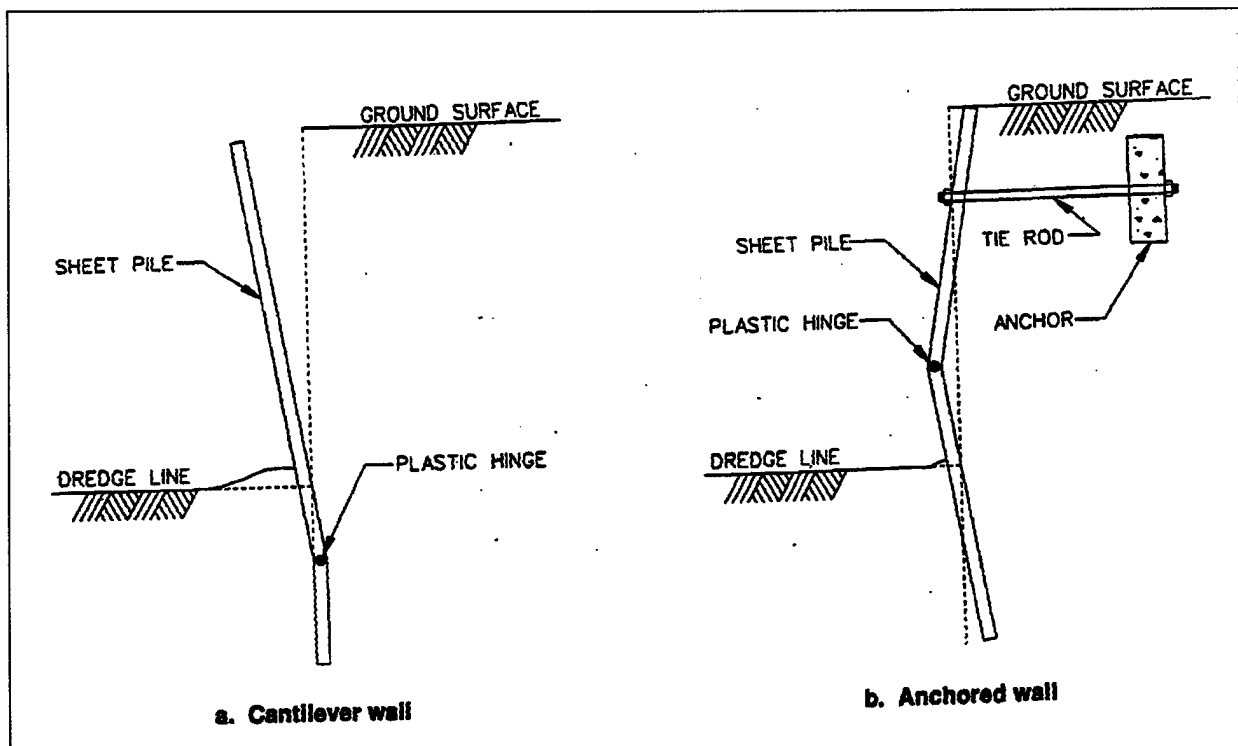
Figure 5-3. Flexural failure of sheet piling
