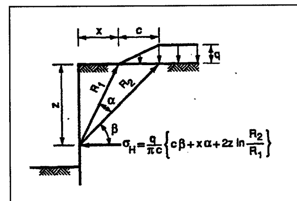
Figure 4-7. Ramp load
