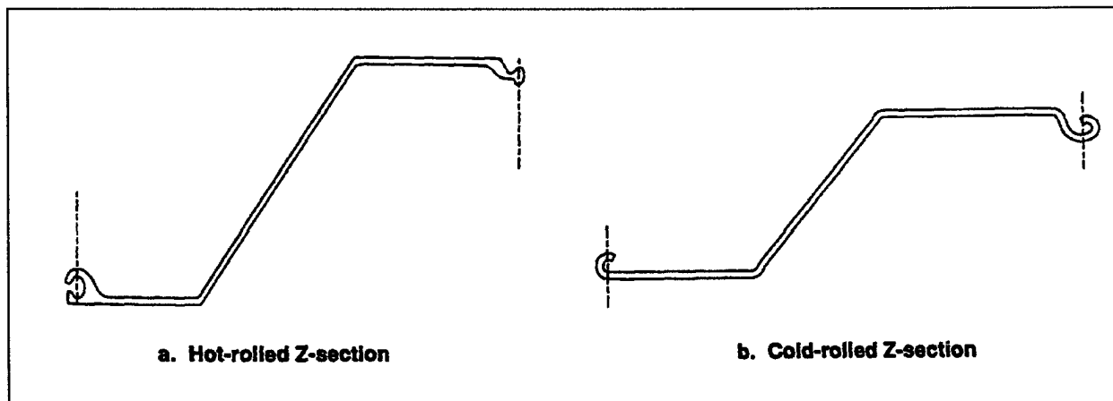
Figure 2-4. Typical light-gauge steel piling
