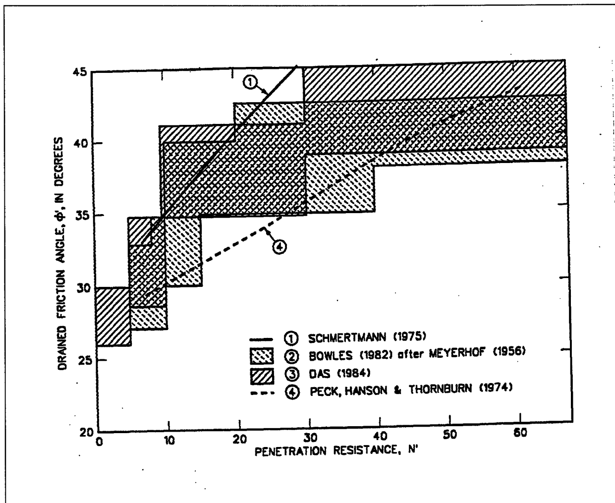
Figure 3-6. Correlations between SPT results and shear strength of granular materials
