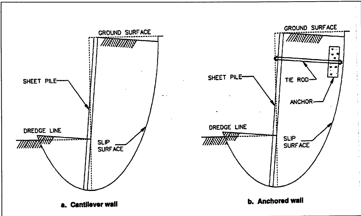
Figure 5-1. Deep-seated failure
