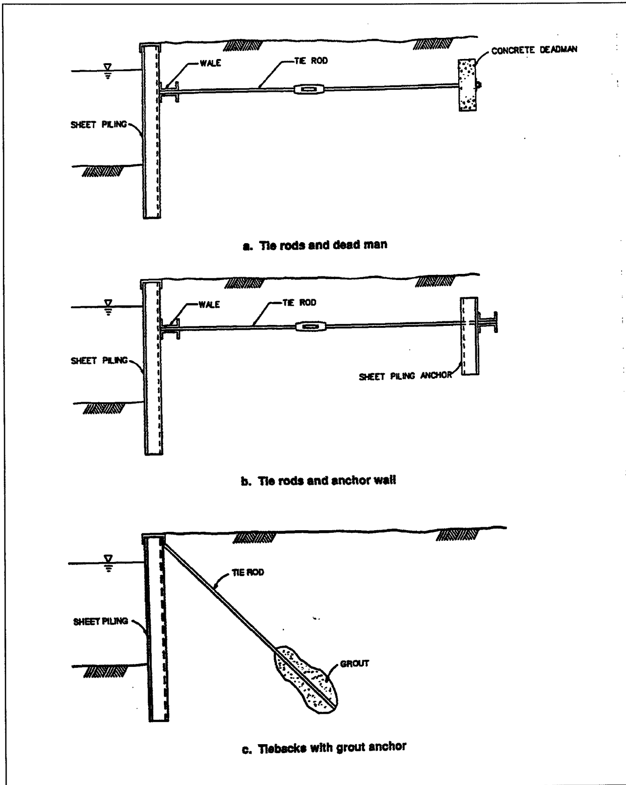
Figure 2-2. Anchored walls (Continued)
