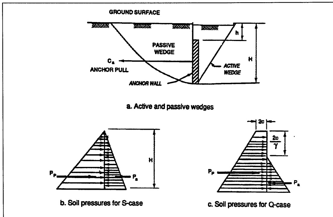
Figure 5-9. Resistance of continuous anchor wall
