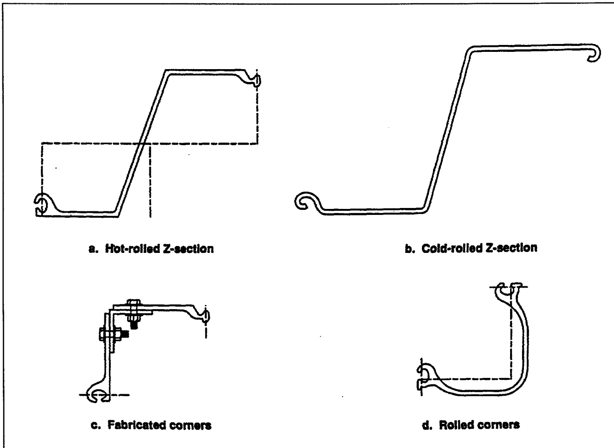
Figure 2-3. Typical heavy-gauge steel piling
