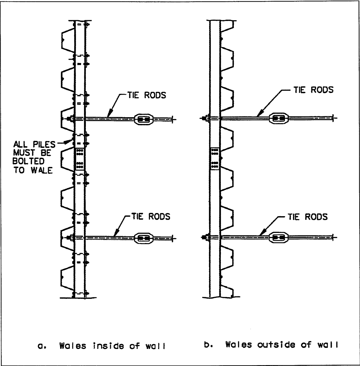
Figure 6-5. Typical wale configurations
