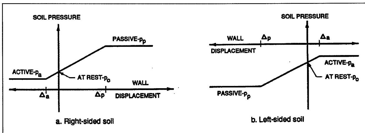
Figure 7-2. Distributed soil springs
