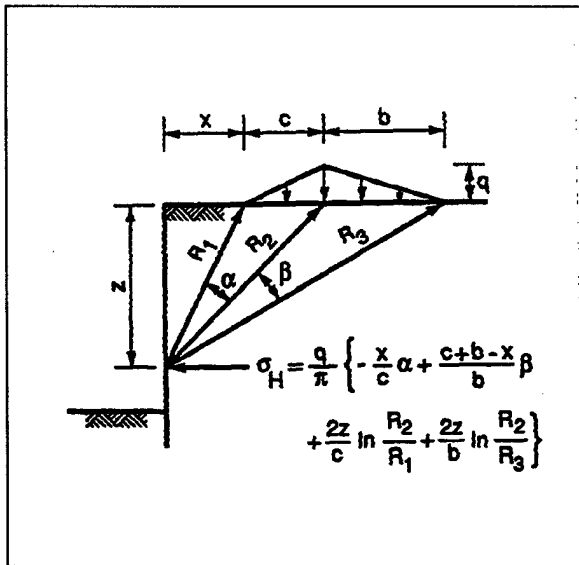
Figure 4-8. Triangular load
