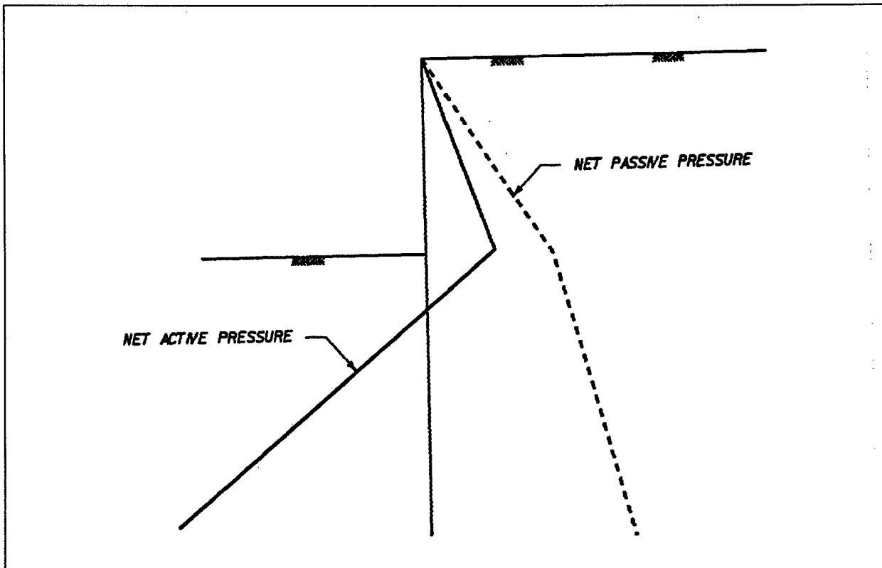
Figure 5-5. Typical net pressure distributions
