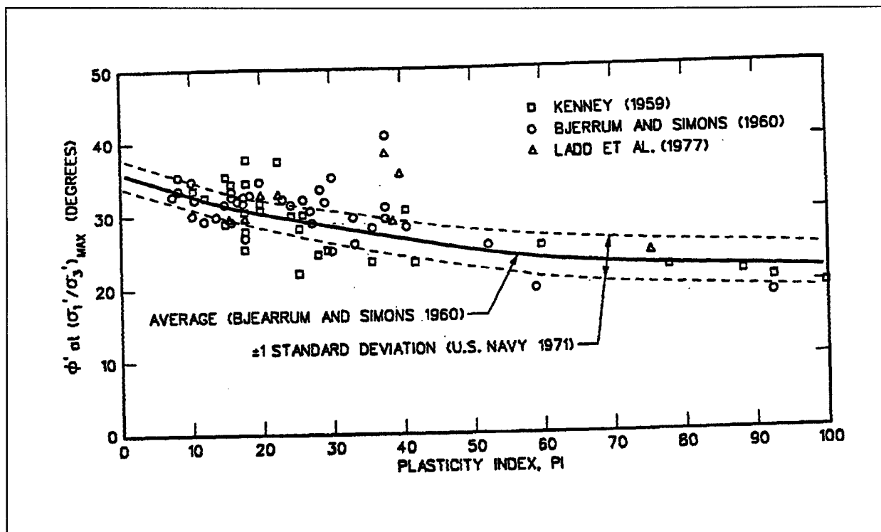
Figure 3-4. Empirical correlation between friction angle and PI from triaxial tests on normally consolidated clays
