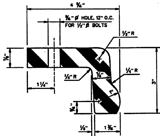
L-TYPE WATERSTOP
