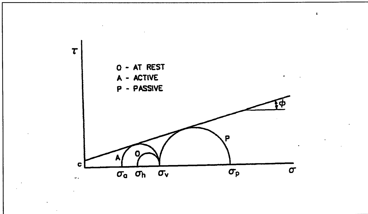
Figure 4-2. Definition of active and passive earth pressures
