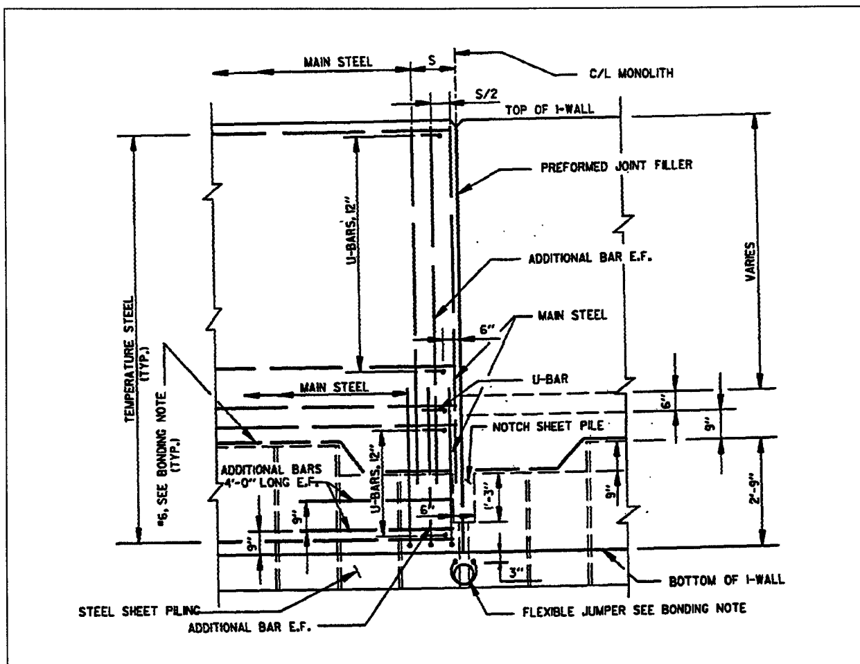
Figure 9-2. Detail of I-wall of varying thickness
