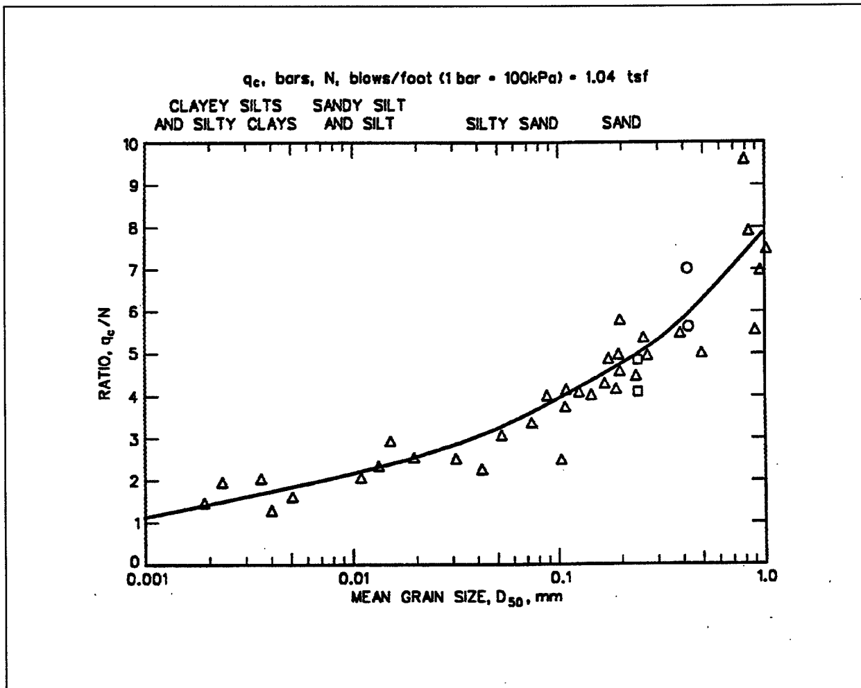
Figure 3-7. Correlation between grain size and the ratio of cone bearing and STP resistance (after Robertson and Campanella 1983)
