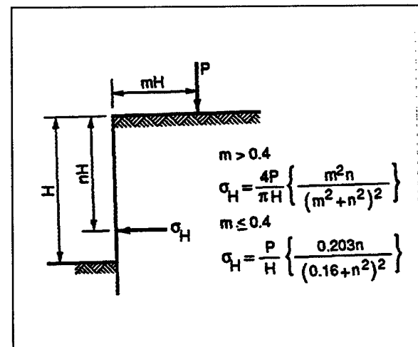
Figure 4-6. Line load
