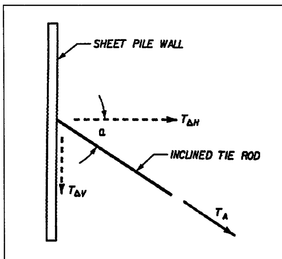
Figure 6-3. Anchor force components for inclined anchors
