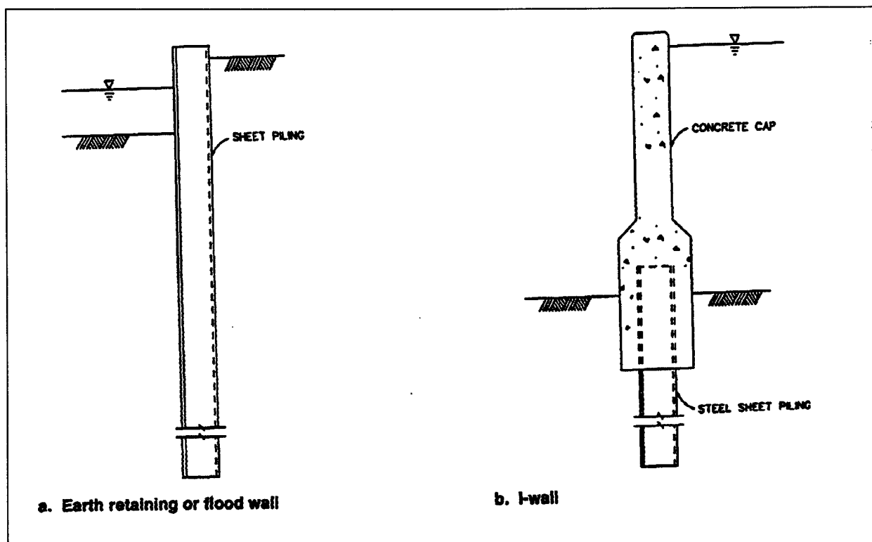
Figure 2-1. Typical cantilevered walls
