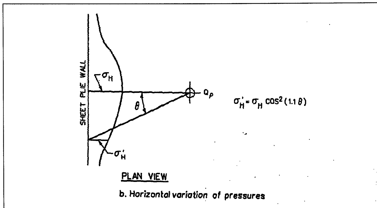
Figure 4-9. Point load (after Terzaghi 1954)
