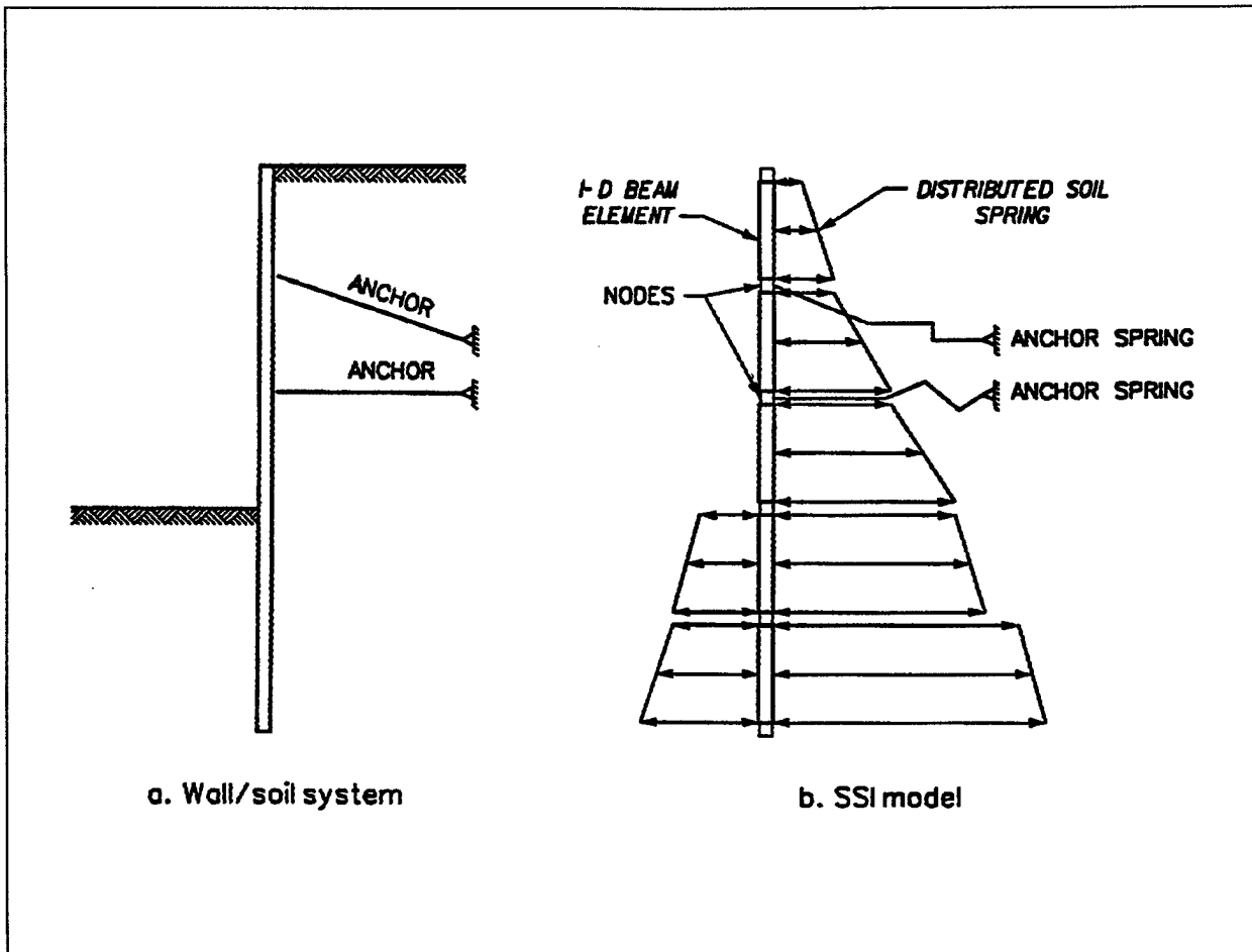
Figure 7-1. System for SSI analysis
