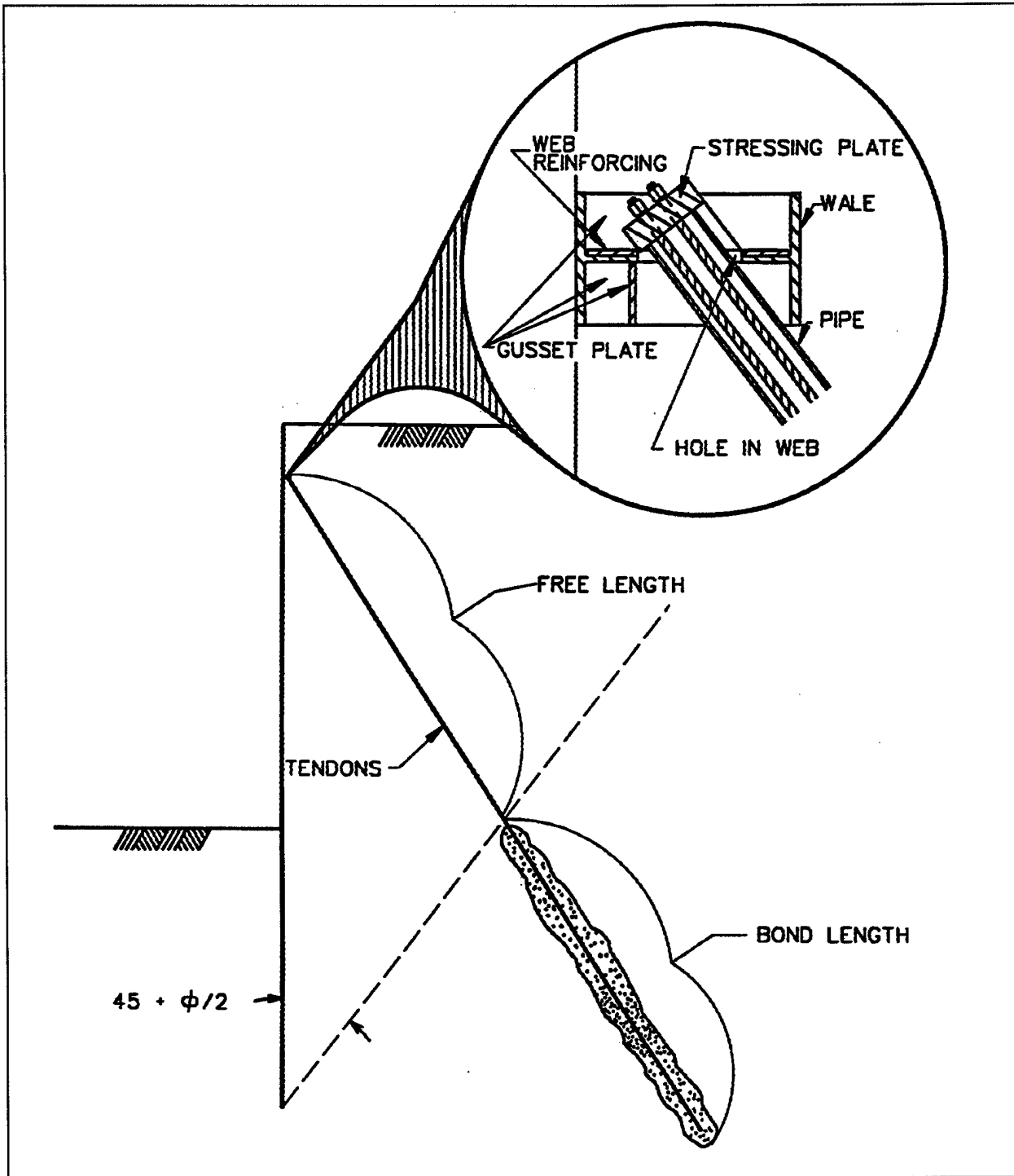
Figure 5-11. Grouted anchors
