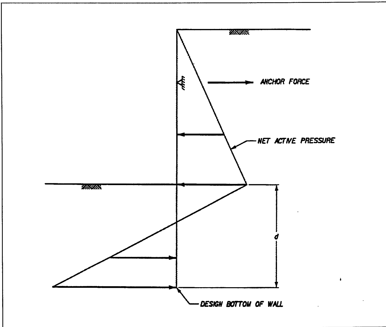
Figure 5-7. Design pressure distribution for free earth design of anchored walls
