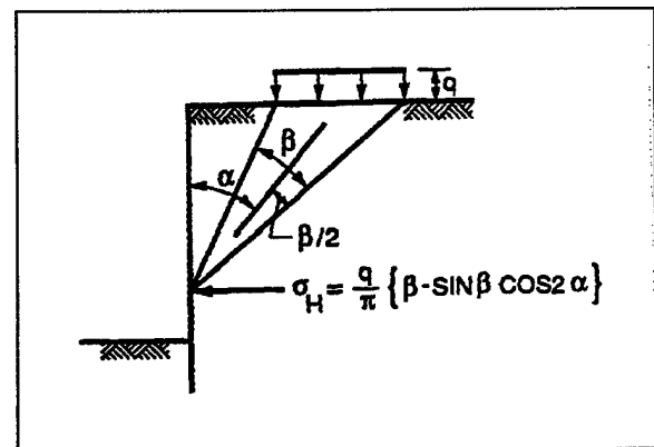
Figure 4-5. Strip load
