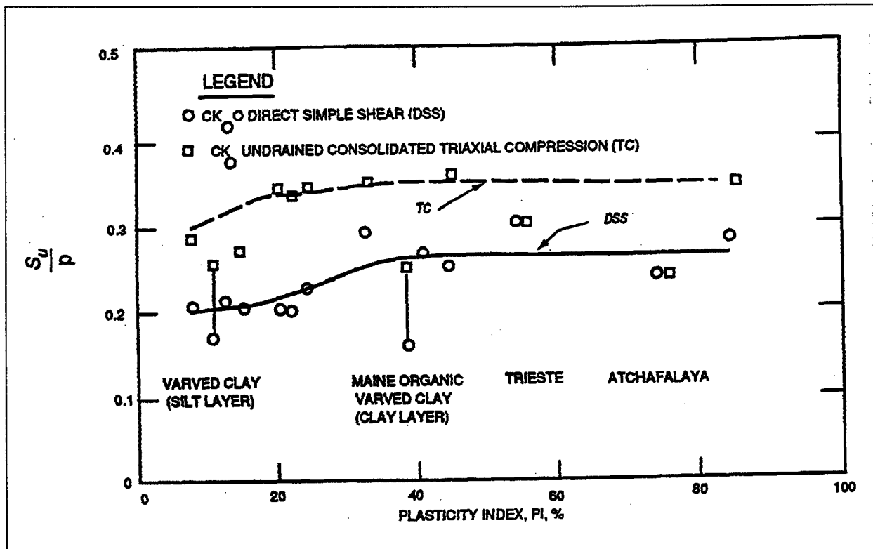
Figure 3-2. Relationship between the ratio S_u/p and plasticity index for normally consolidated clays (after Gardner 1977)
