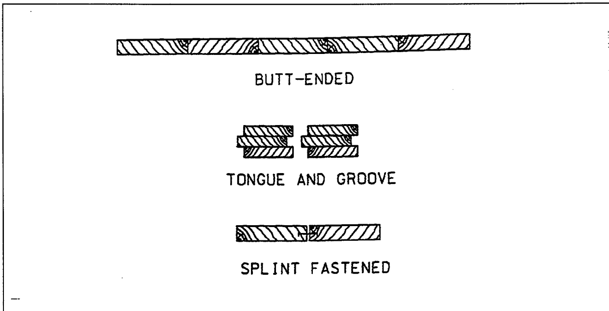
Figure 2-5. Typical wood sections
