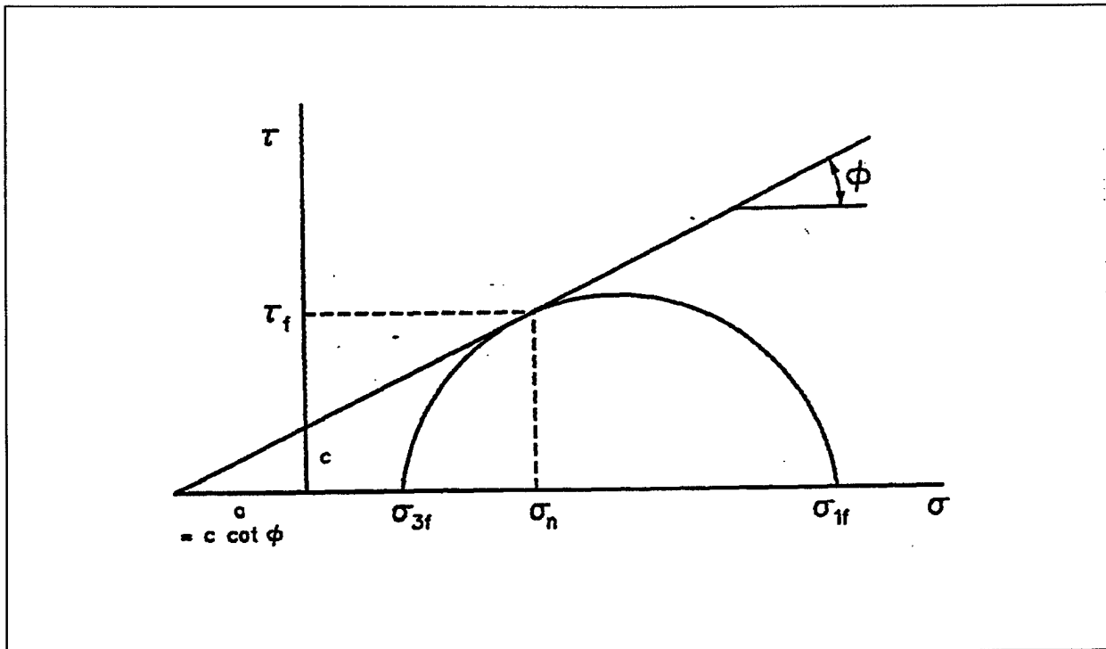
Figure 4-1. Shear strength parameters
