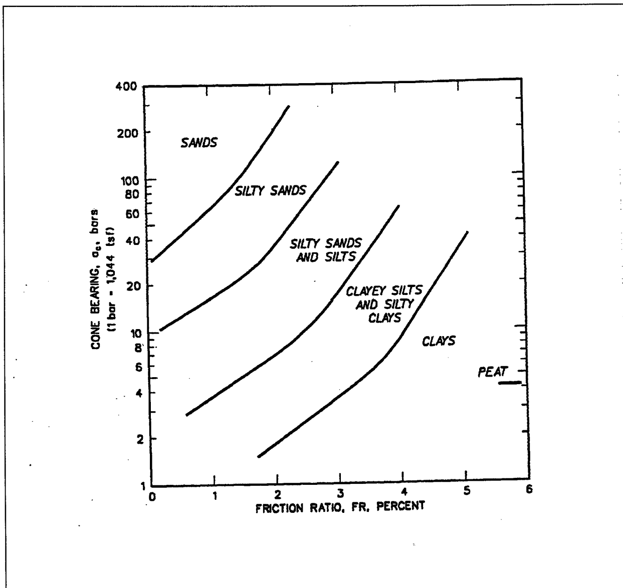
Figure 3-8. Soil classification from cone penetrometer (after Robertson and Campanella 1983)
