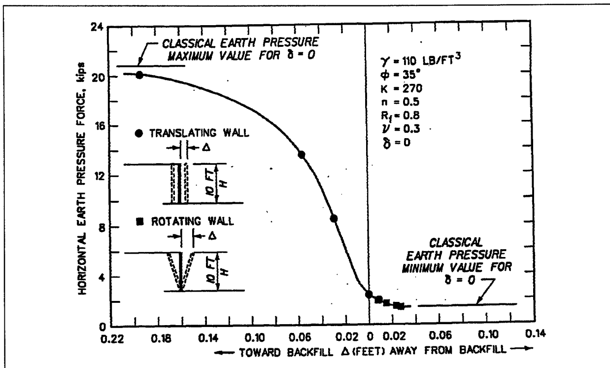
Figure 4-3. Variations of earth pressure force with wall movement calculated by finite element analyses (after Clough and Duncan 1971)
