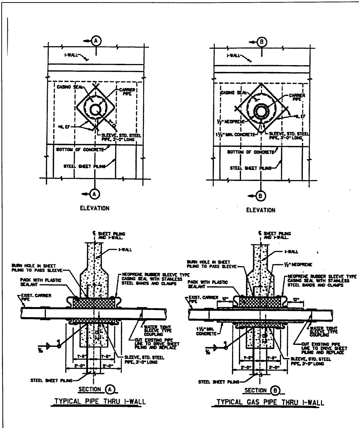
Figure 9-3. Typical utility crossings (Sheet 1 of 4)
