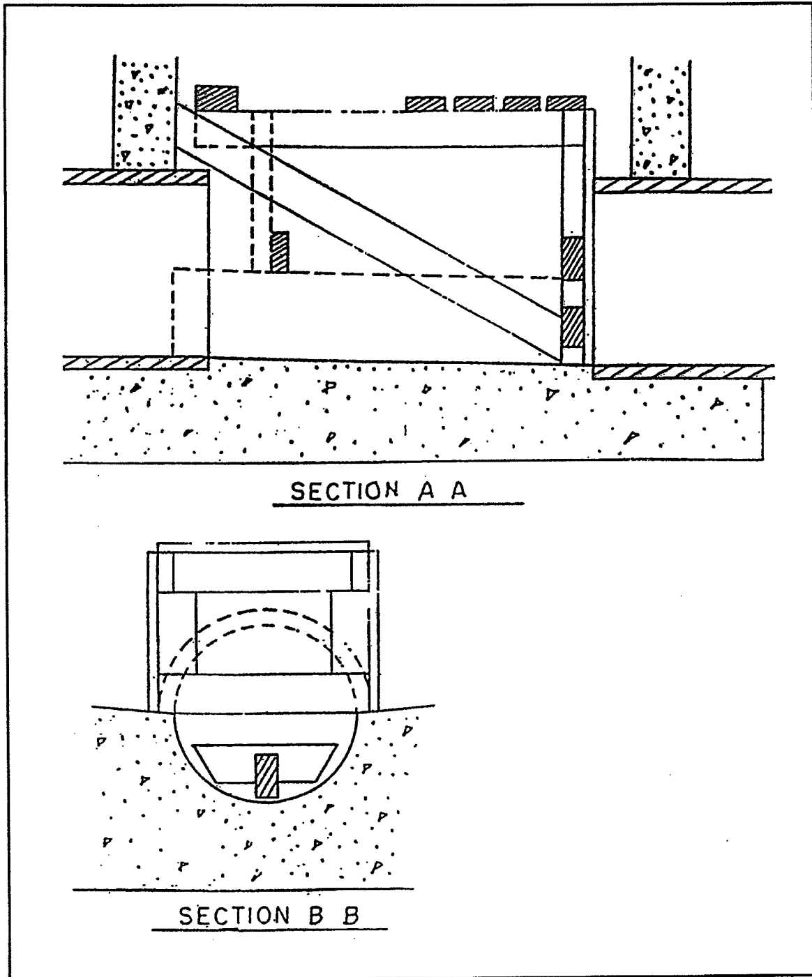
Figure F-10. Treatment of bottom of manhole
