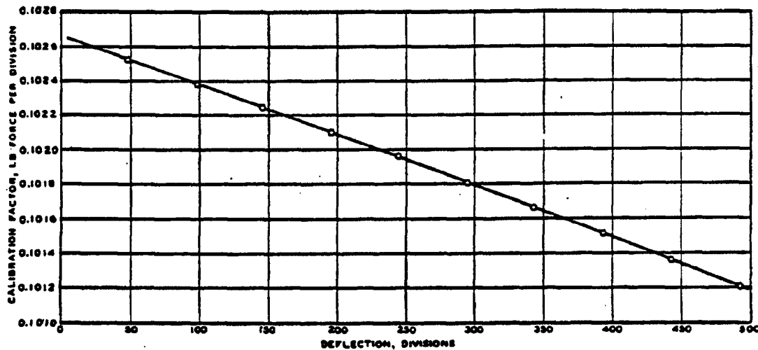
Fig. 12. Calibration factors for a 50-lb compression load ring
