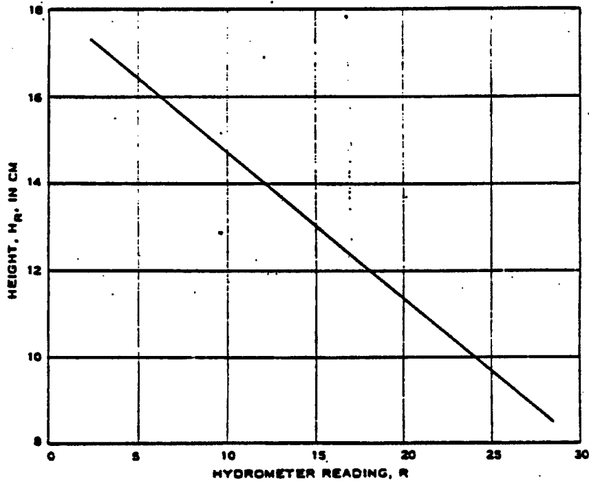
b. TYPICAL HYDROMETER CALIBRATION CURVE
