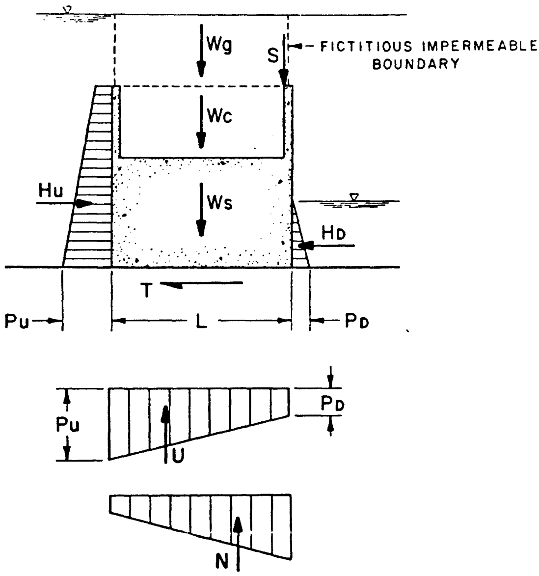
Figure B-1. Generic Geometry and Loading Conditions
