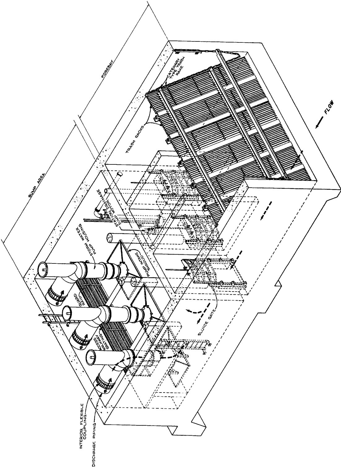
EN 1115-100 STRUCTURAL AND ARCHITECTURAL DESIGN OF PUMPING STATIONS TYPICAL OPEN PUMPING STATION SUBSTRUCTURE
