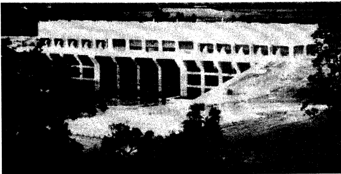
Photograph 1 W.G. Huxtable Pumping Station -- Exterior View
