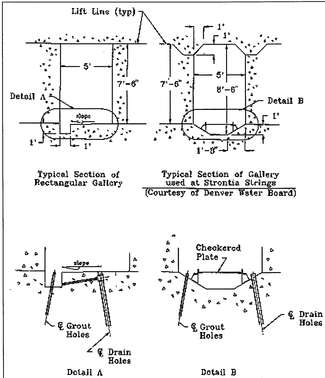
Figure 13-16. Typical gallery details
