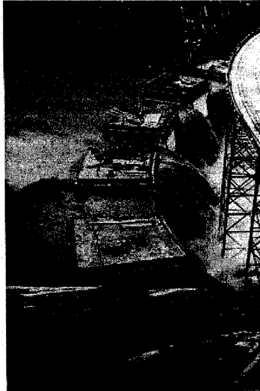
Figure 13-1. View from right abutment of partially complete Monticello Dam in California showing water flowing over low blocks (USBR)
