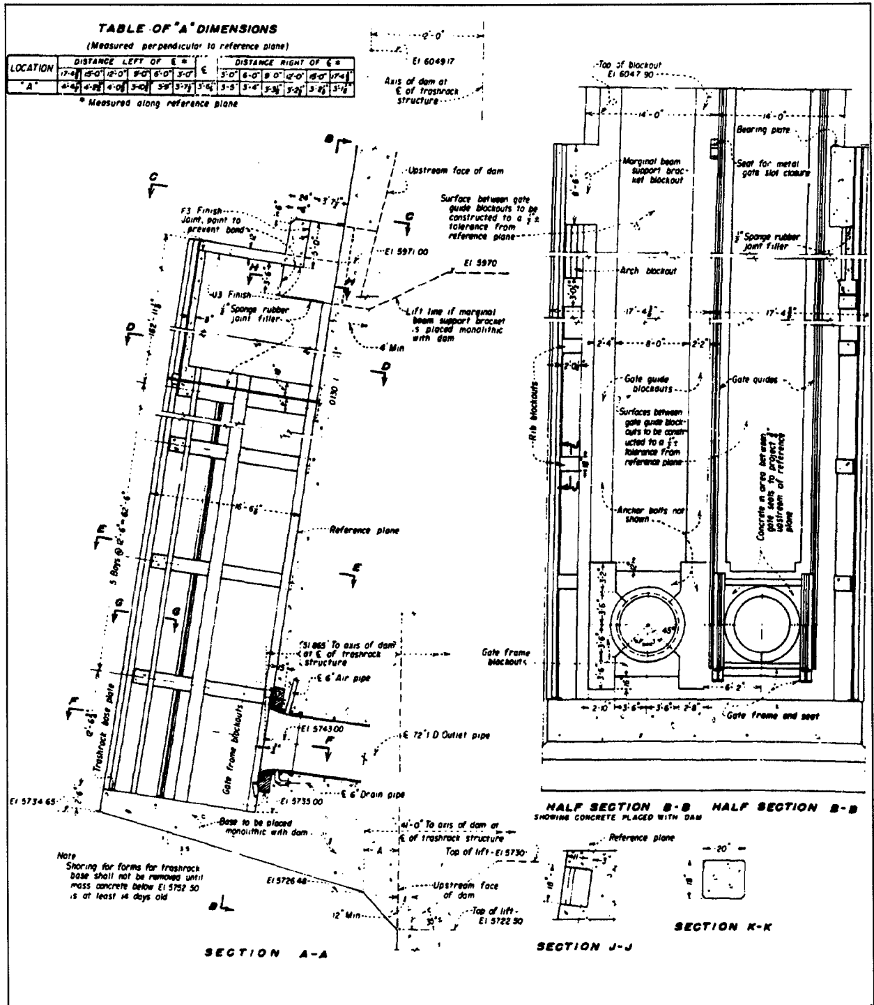
Figure 3-8. Typical river outlets trashrack structure (USBR)
