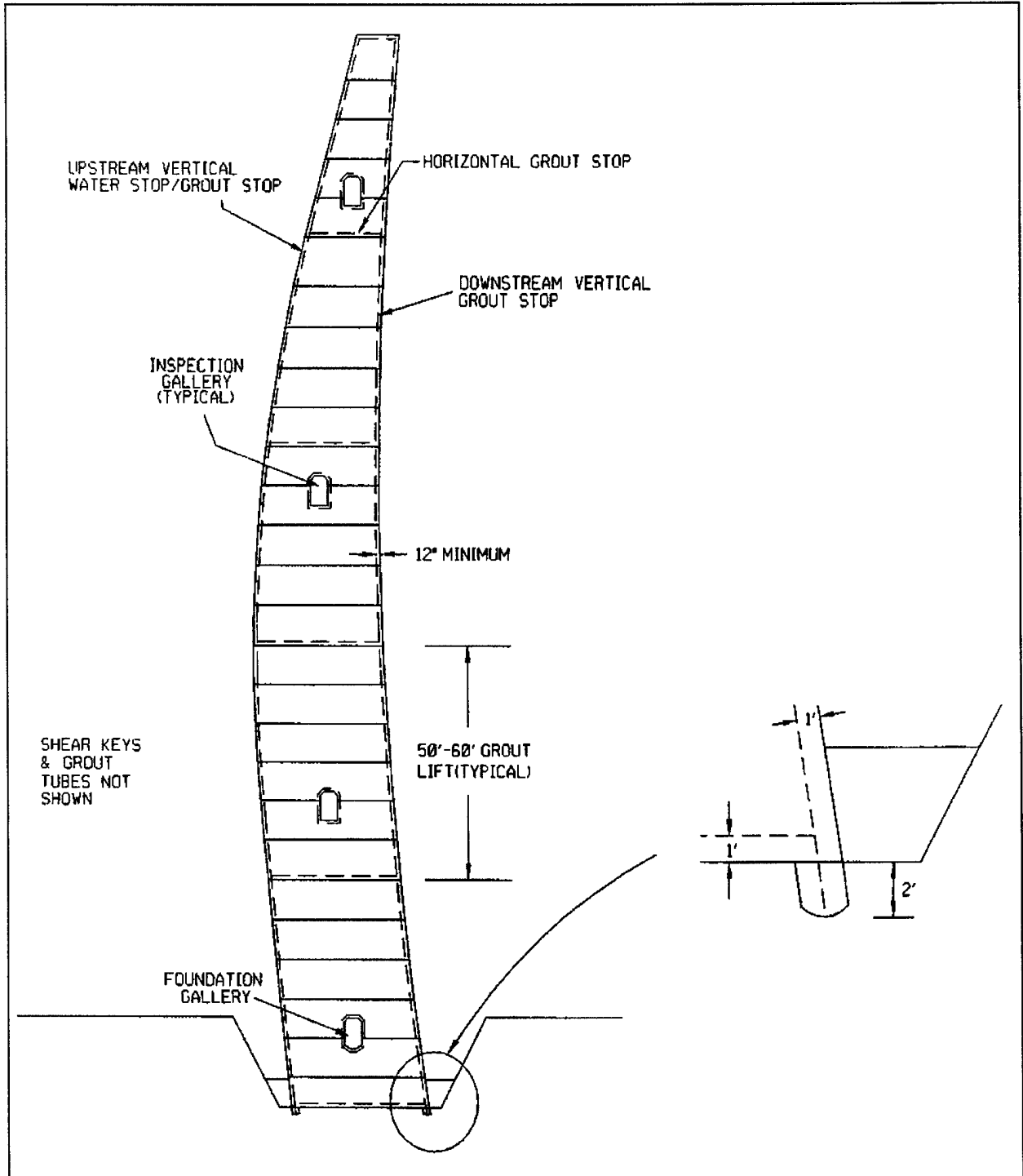
Figure 13-10. Water stop and grout stop details
