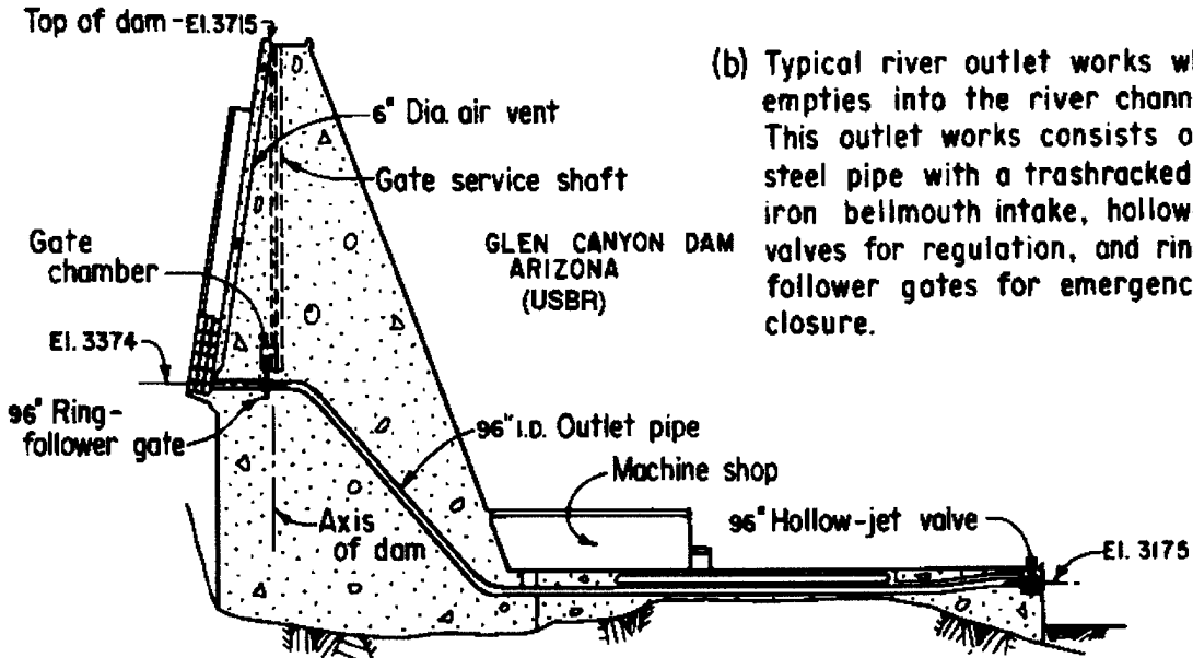
SECTION THRU RIVER OUTLETS (b)
