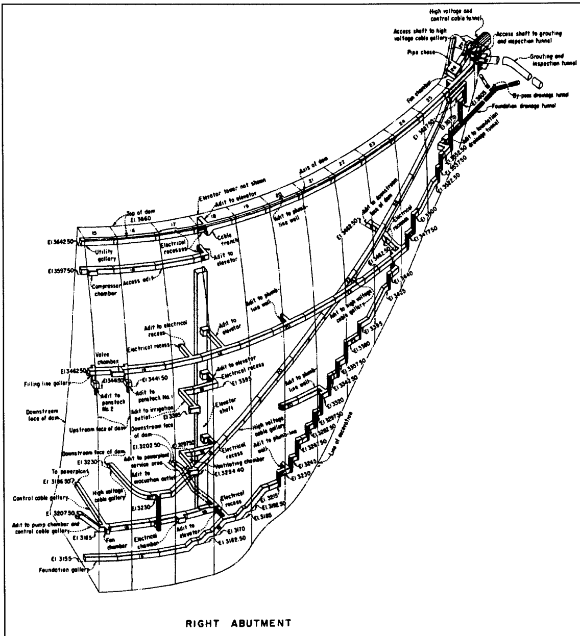
Figure 3-15. Gallery system in right side of Yellowtail Dam (USBR)
