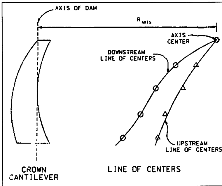
Figure 5-9. Development of the lines of centers
