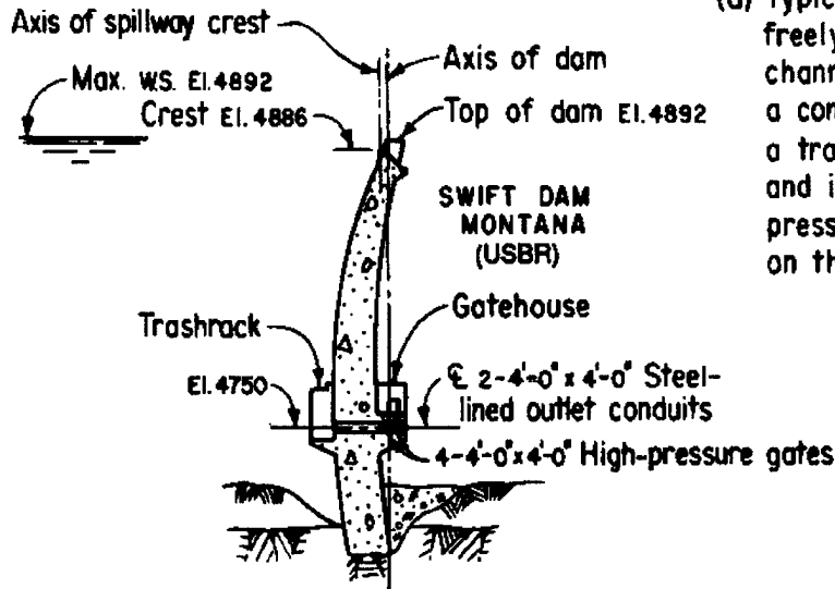
SECTION THRU RIVER OUTLETS (a)
