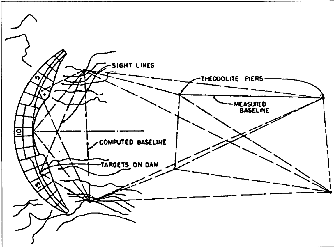
Figure 12-6. Layout for triangular or trilateration network
