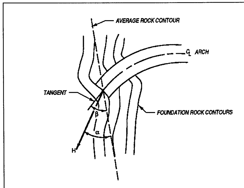
Figure 2-1. Angle between arch thrust and rock contours
