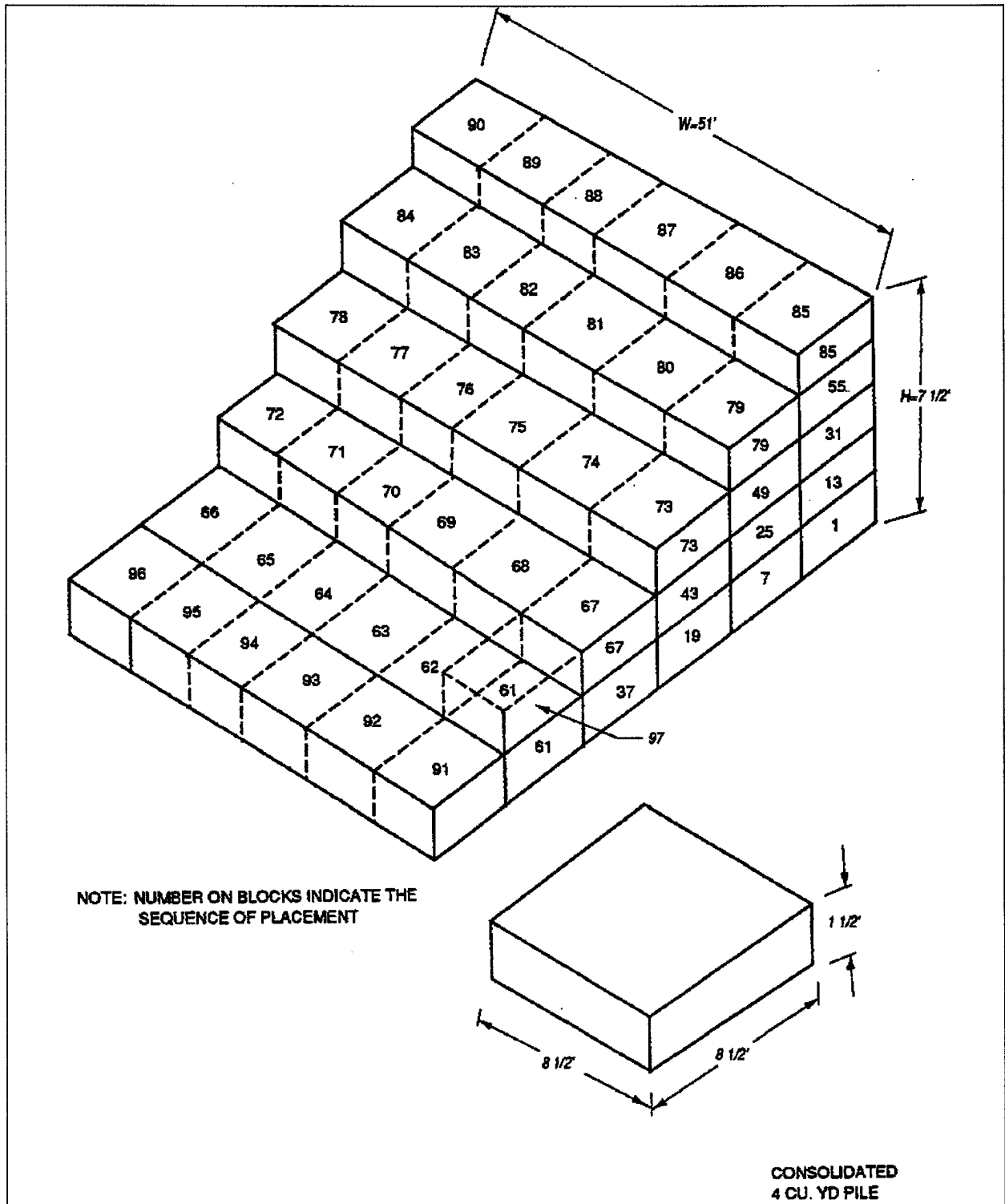
Figure 3-1. Stepped placement sequence and plant capacity, 7-1/2-ft lift height
