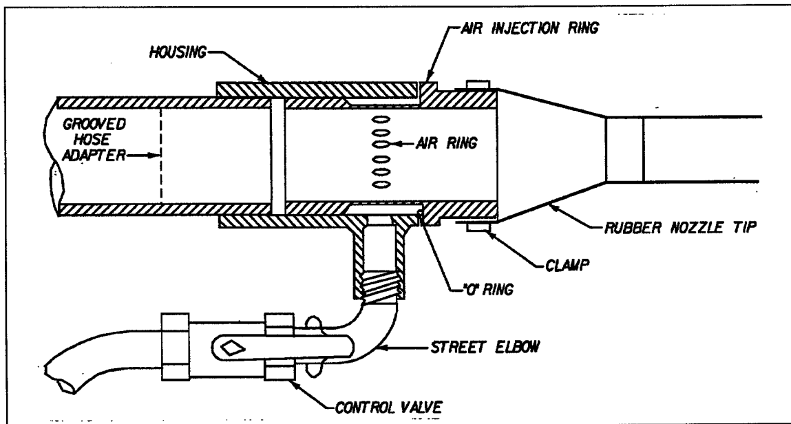
Figure 4-9. Typical wet-mix nozzle (paragraph A-2, ACI 1991c; copyright permission granted by ACI)
