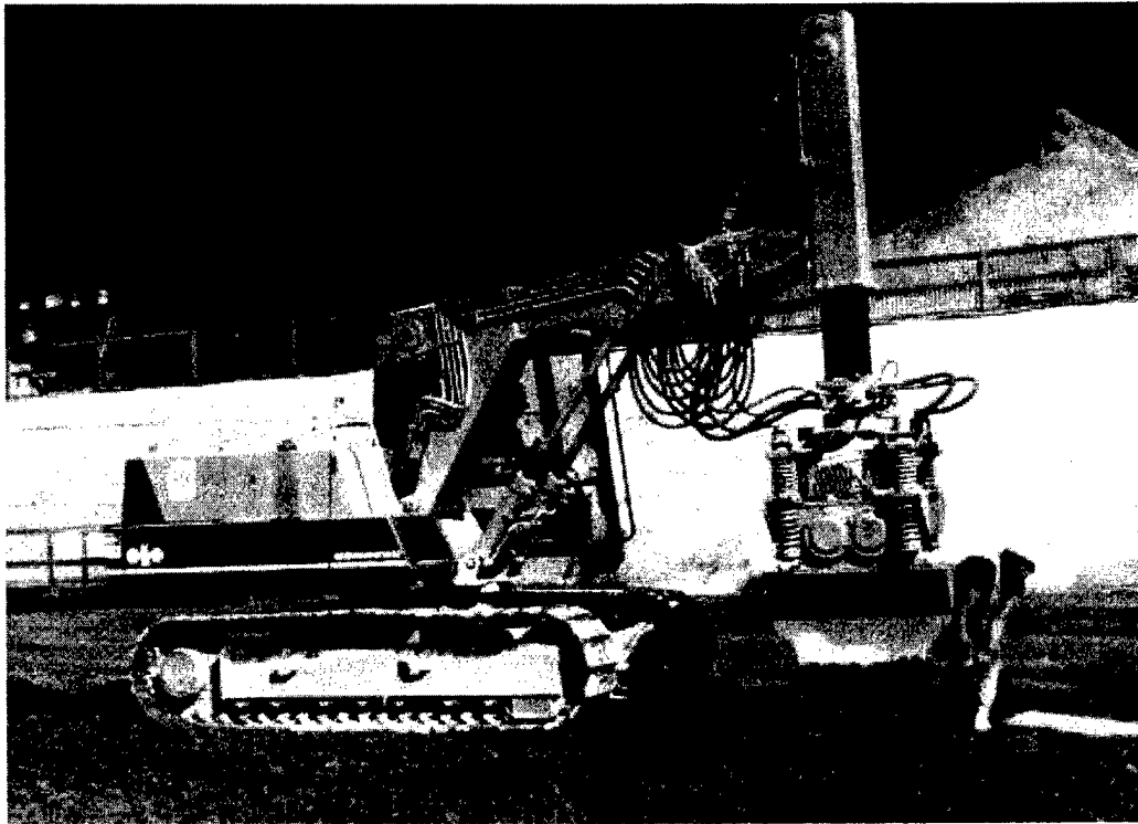
Figure 6-3. Installation of sheet metal joints with vibrating blade
