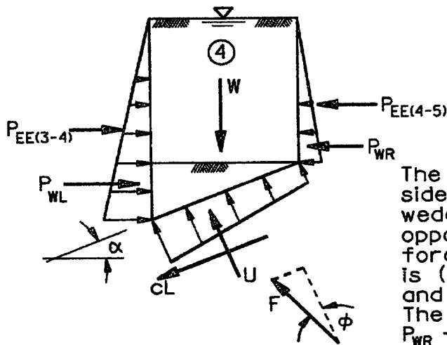
b. Free-body diagram of slice 4
