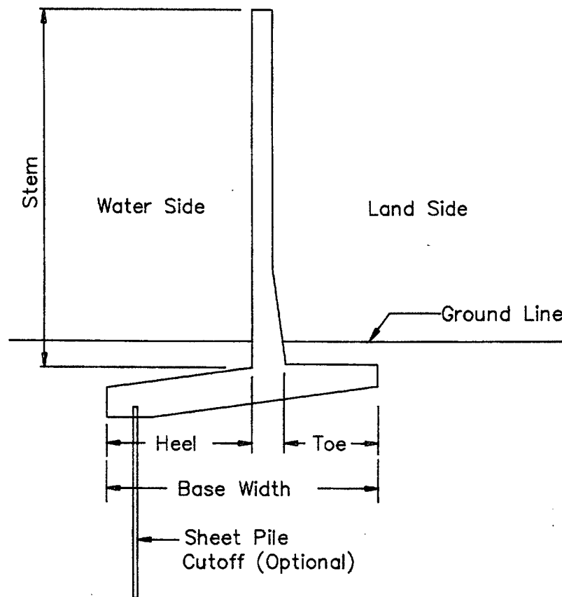
Figure 7-4. T-type flood wall--sloped base
