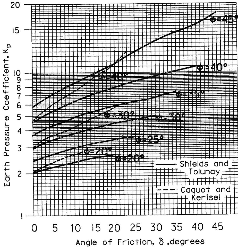
Figure 3-18. Passive earth pressure coefficients
