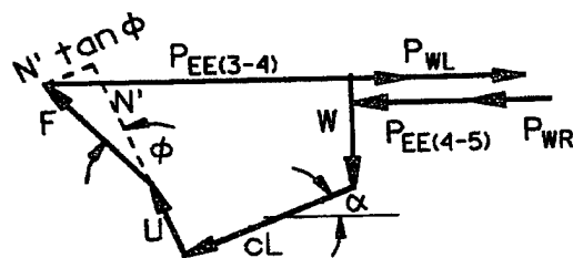
c. Force polygon for slice 4
