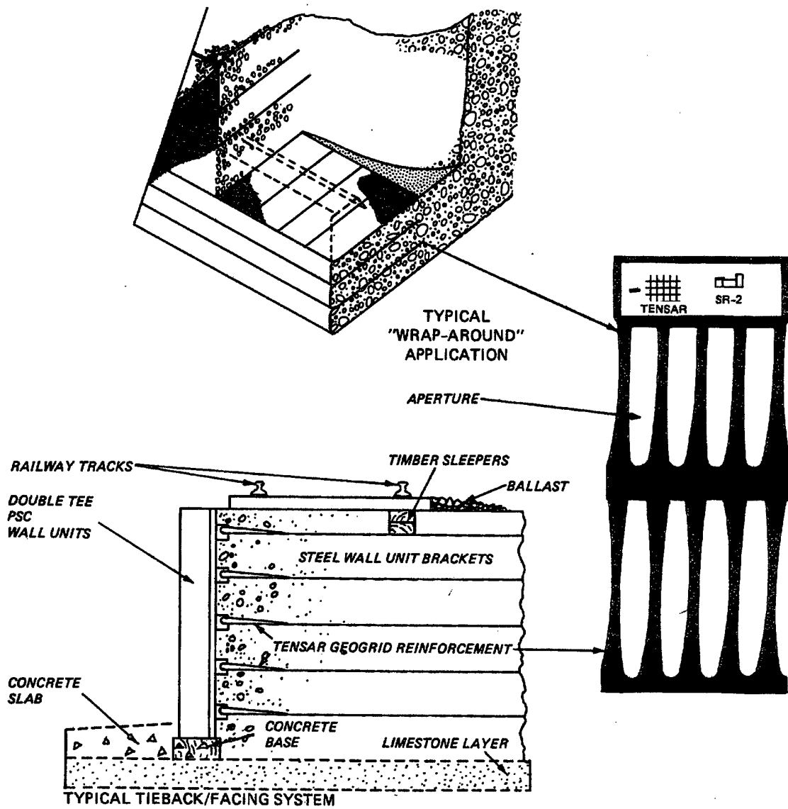
Figure 10-4. Tensar geogrid retaining wall (adapted from Tensar Corporation 1984)
