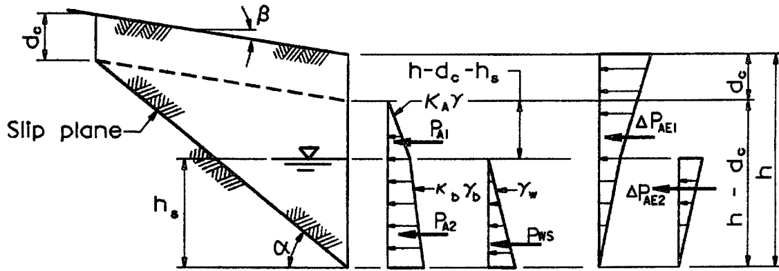
a. Driving wedge
