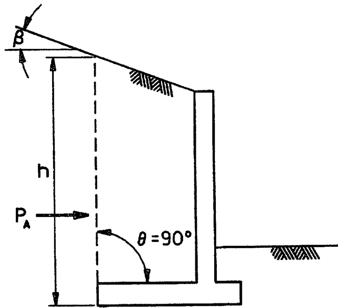
Figure 3-10. Variables used in Coulomb equation
