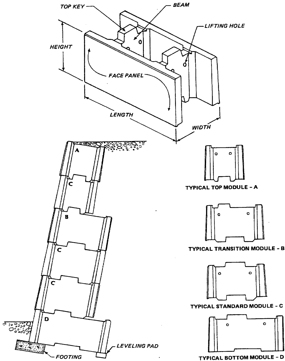
Figure 10-5. Schematic diagram of Doublewal retaining wall (after Doublewal Corporation 1984)
