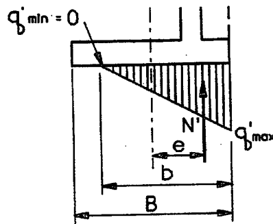
c. Pressure for resultant outside middle one-third
