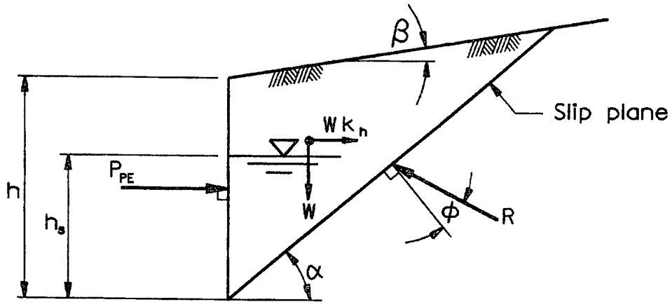
b. Resisting wedge
