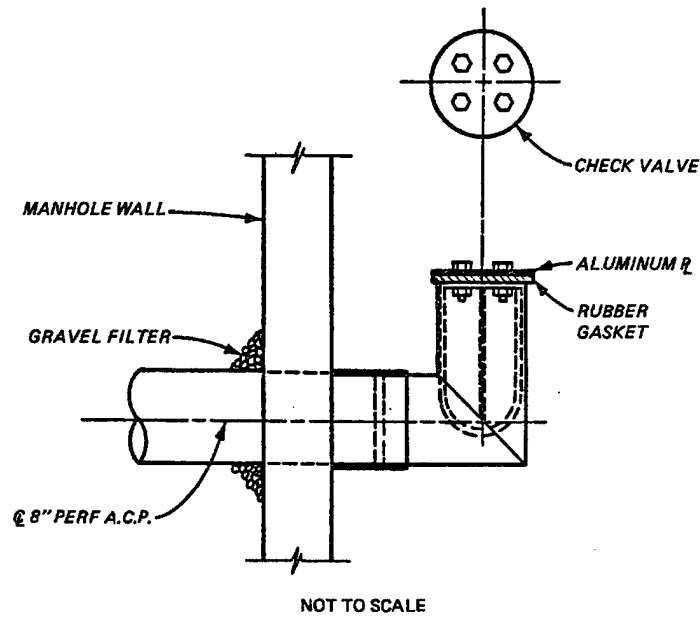
Figure 6-8. Vertical check valve at end of longitudinal drain
