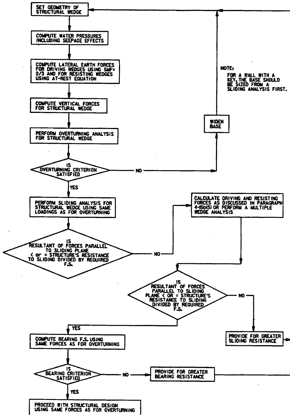
Figure 4-12. Wall design flowchart
