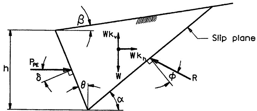
b. Passive wedge
