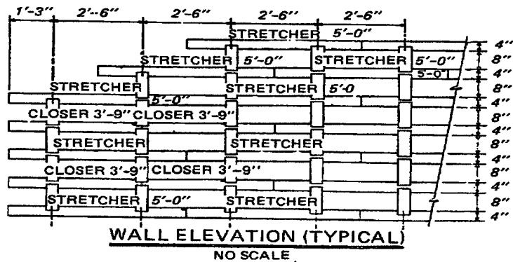
Figure 10-7. Schematic diagram of Criblock retaining wall (after Criblock Retaining Walls of America)
