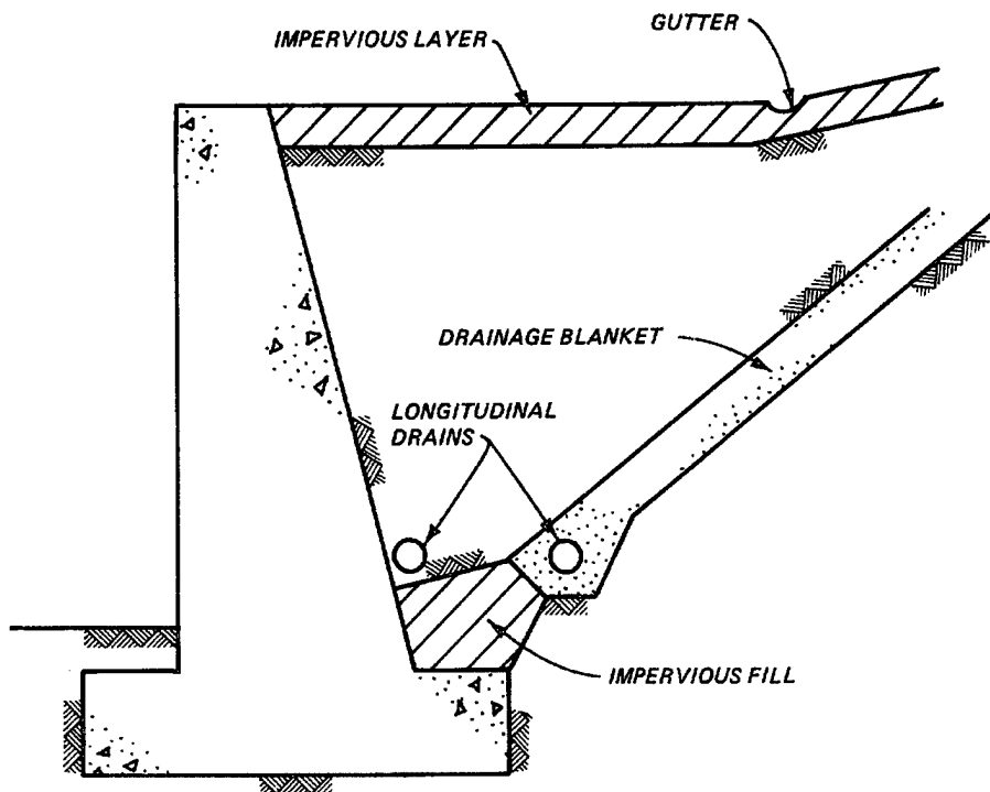
Figure 6-1. Inclined drainage blanket (after Department of the Navy 1982a)
