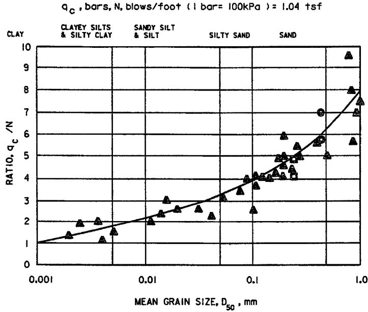
Figure 2-7. q_c/N versus D_{50} (after Robertson and Campanella 1983)
