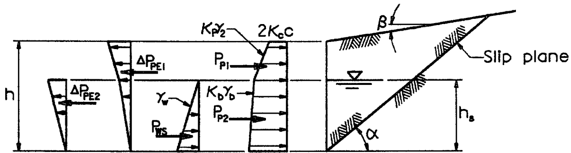
b. Resisting wedge
