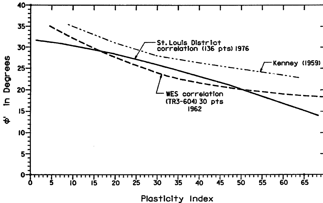
Figure 2-4. Drained friction angle versus plasticity index
