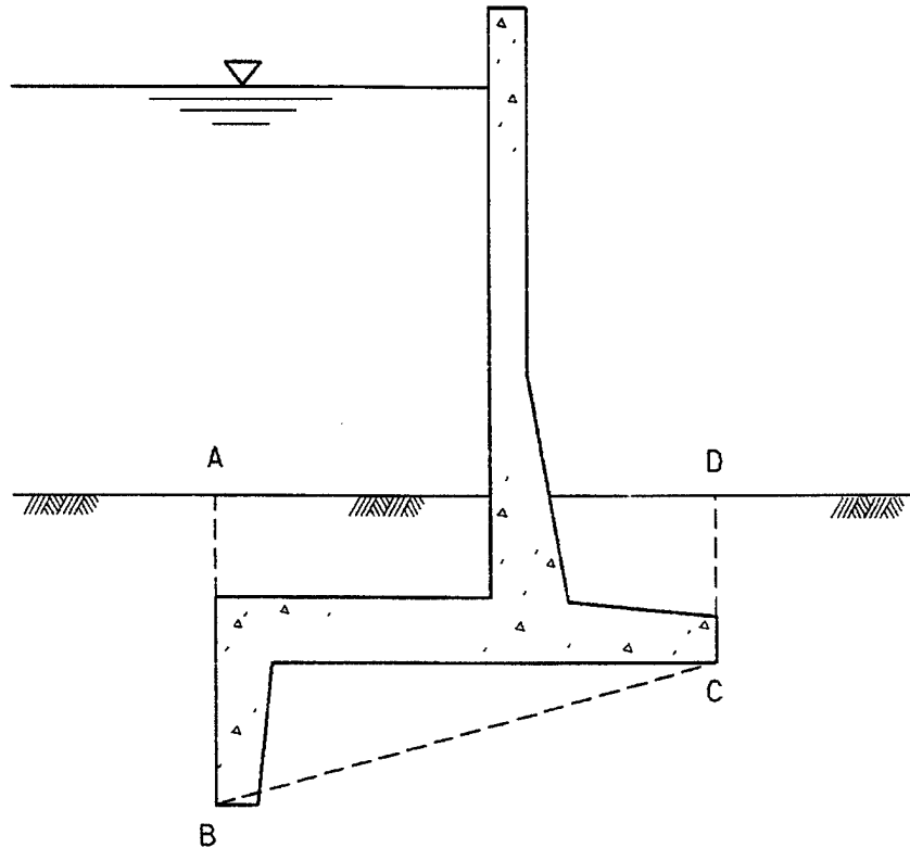
Figure 3-33. Seepage path for line of creep
