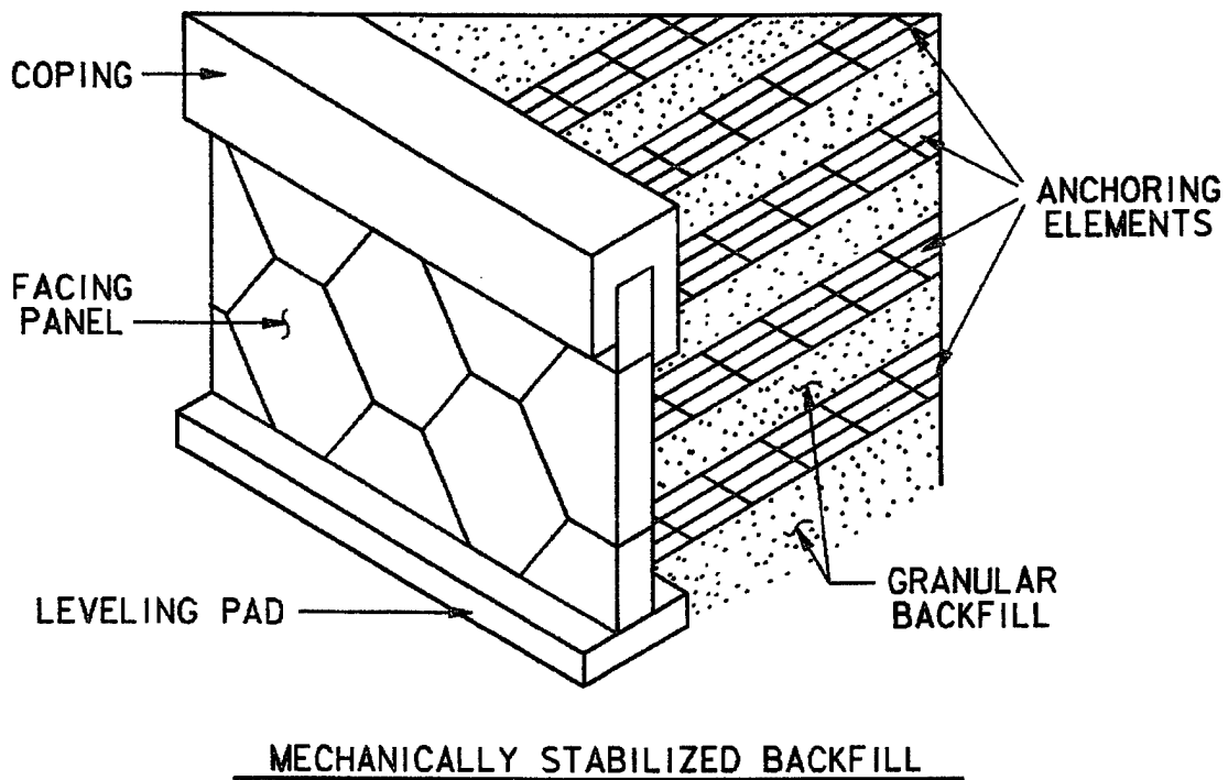
Figure 2-1. Types of retaining walls
