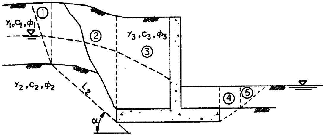
a. Estimation of forces using slices
