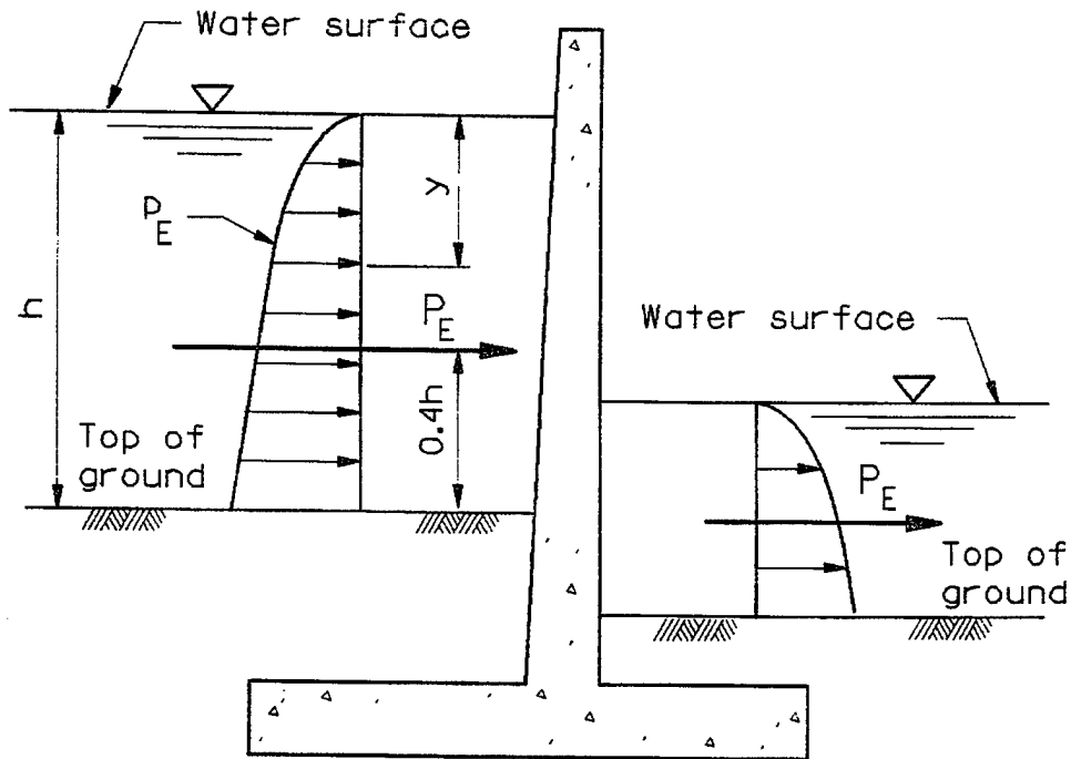
Figure 3-39. Hydrodynamic forces for freestanding water
