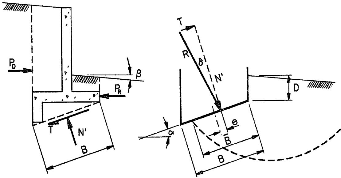
b. Keyed base, sloping ground
