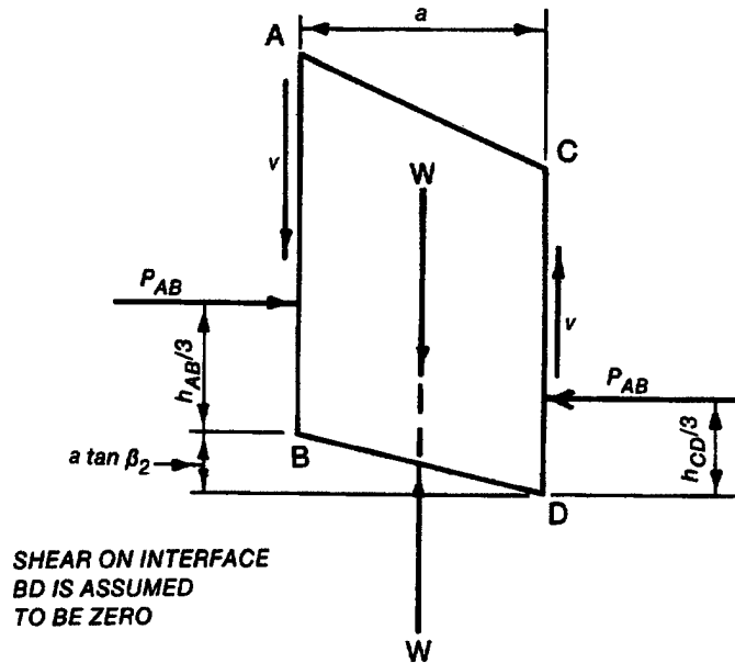
Figure K-2. Free body of Block ABCD.
