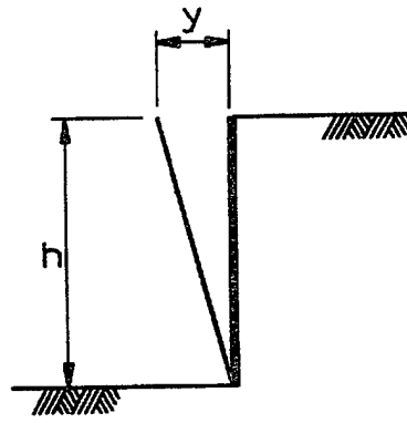
ACTIVE CASE
