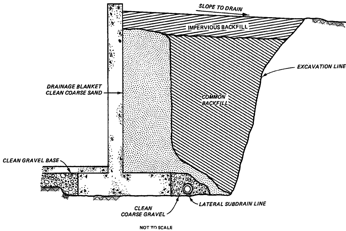
Figure 6-3. Drainage blanket located adjacent to retaining wall (after Sibley 1967)
