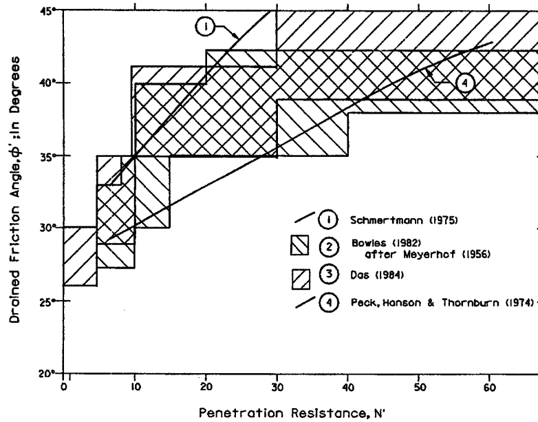
Figure 2-6. \phi' versus N' for granular materials
