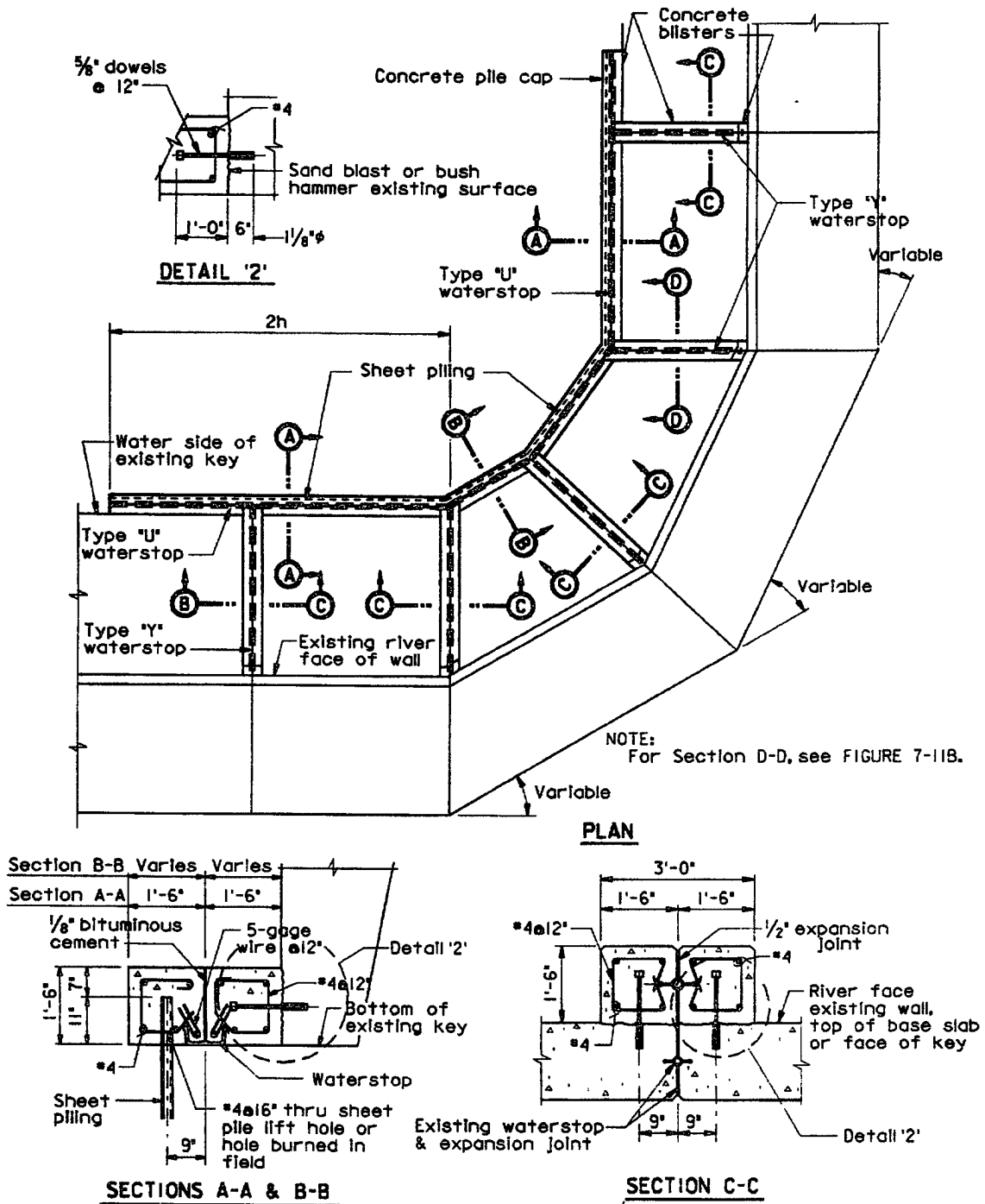
Figure 7-11. Permanent water stop repair measures (Continued)
