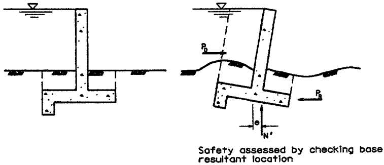
b. Overturning
