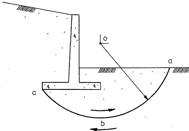
Figure 5-4. Shallow shear surface
