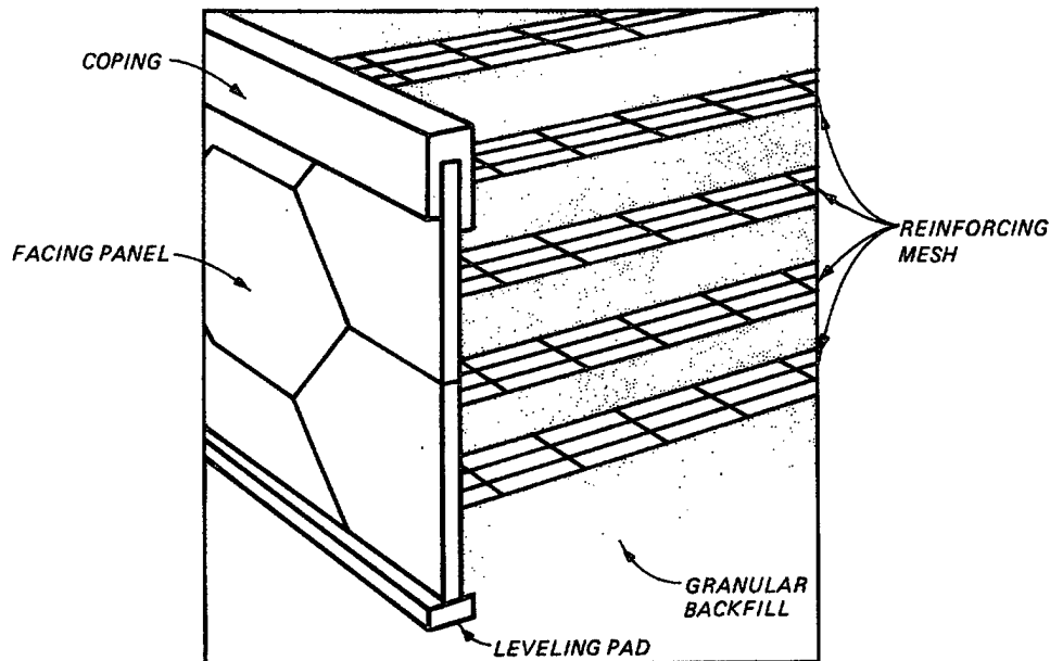
Figure 10-3. VSL retained earth retaining wall (adapted from VSL Corporation 1984)
