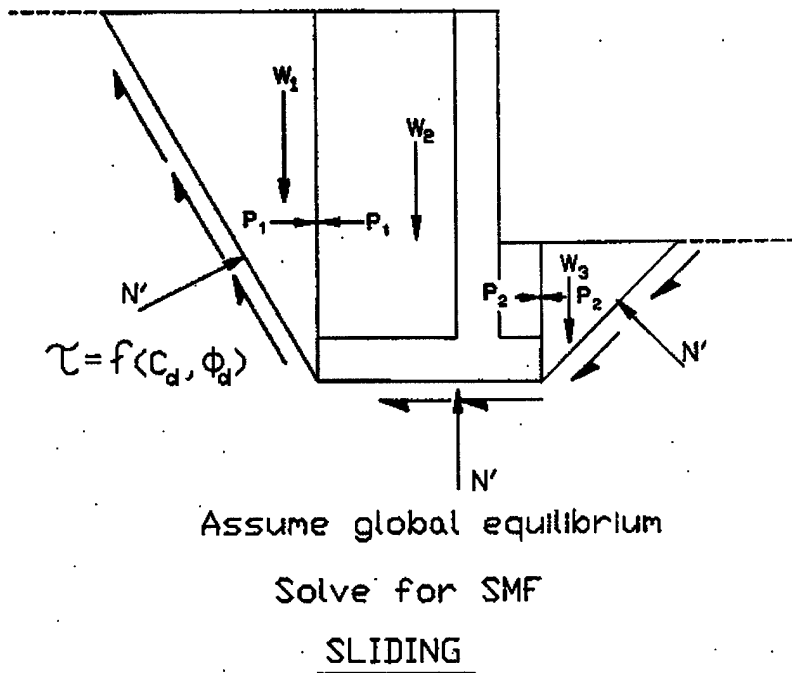
Figure 3-7. Application of the strength mobilization factor
