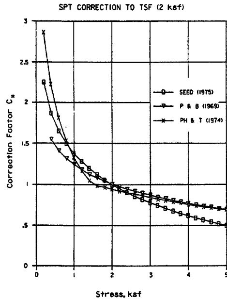
Figure 2-5. SPT correction to 1 tsf (2 ksf)
