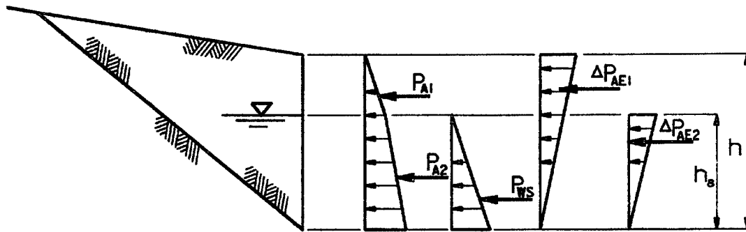
a. Driving wedge
