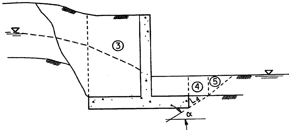
a. Estimation of forces using slices
