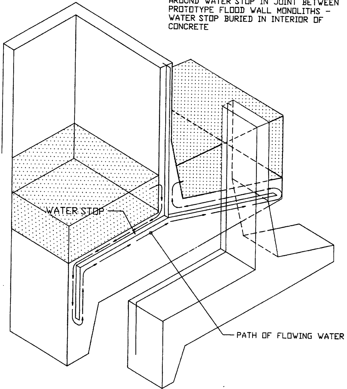
Figure 7-1. Flow around interior embedded water stop in the base
