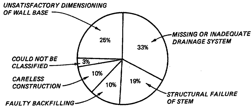
a. Causes of failure of rigid concrete retaining walls (Techeng and Iseux 1972)
