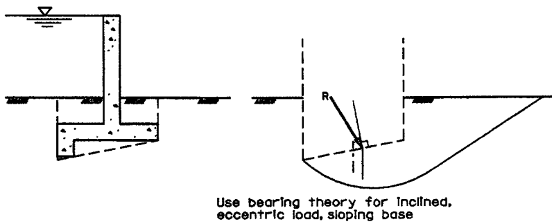
c. Bearing
