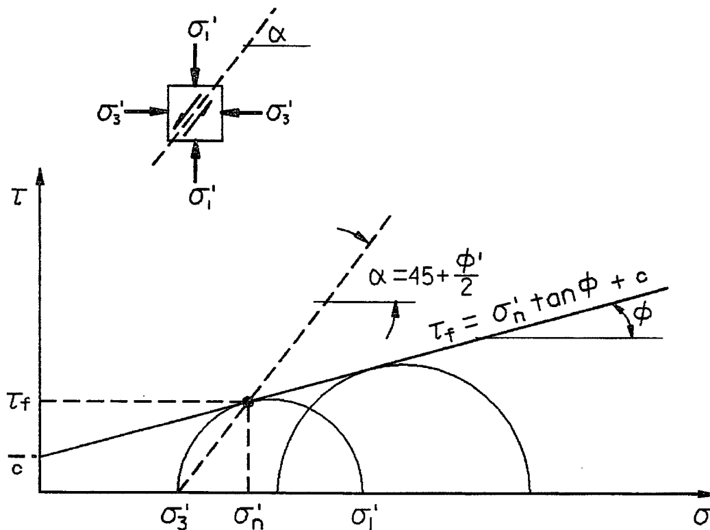
Figure 3-8. Mohr-Coulomb failure criterion
