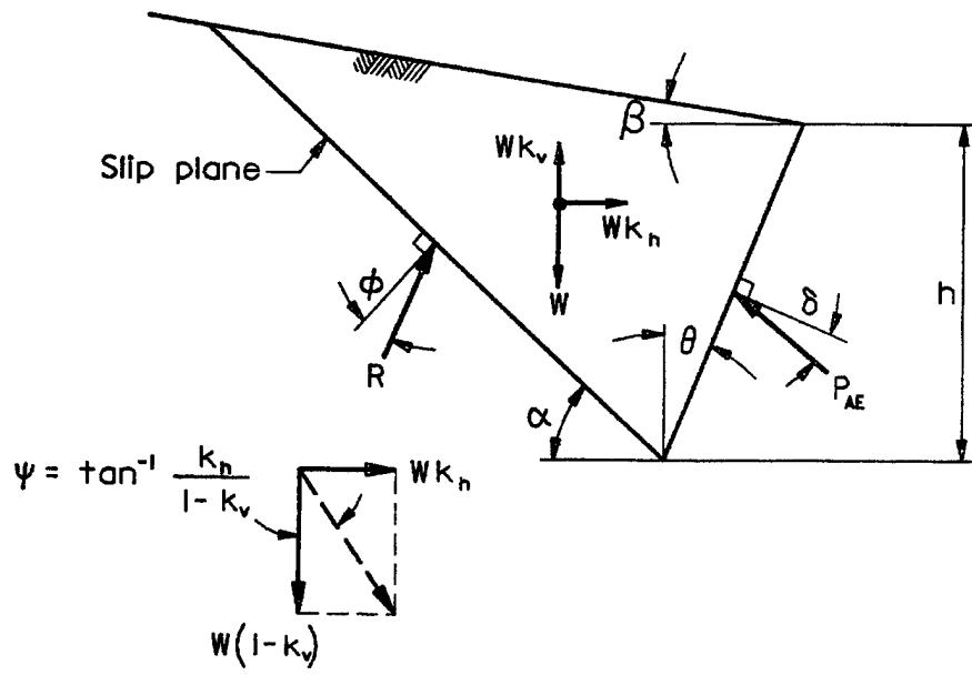
a. Mononobe-Okabe (active) wedge
