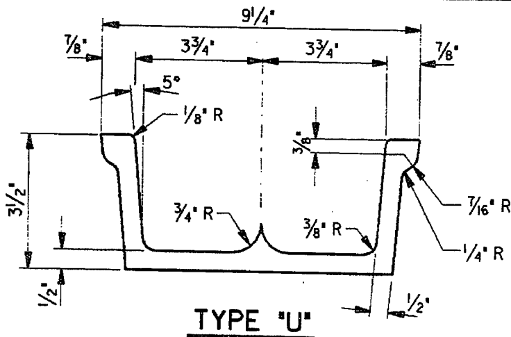
c. Water stop details
