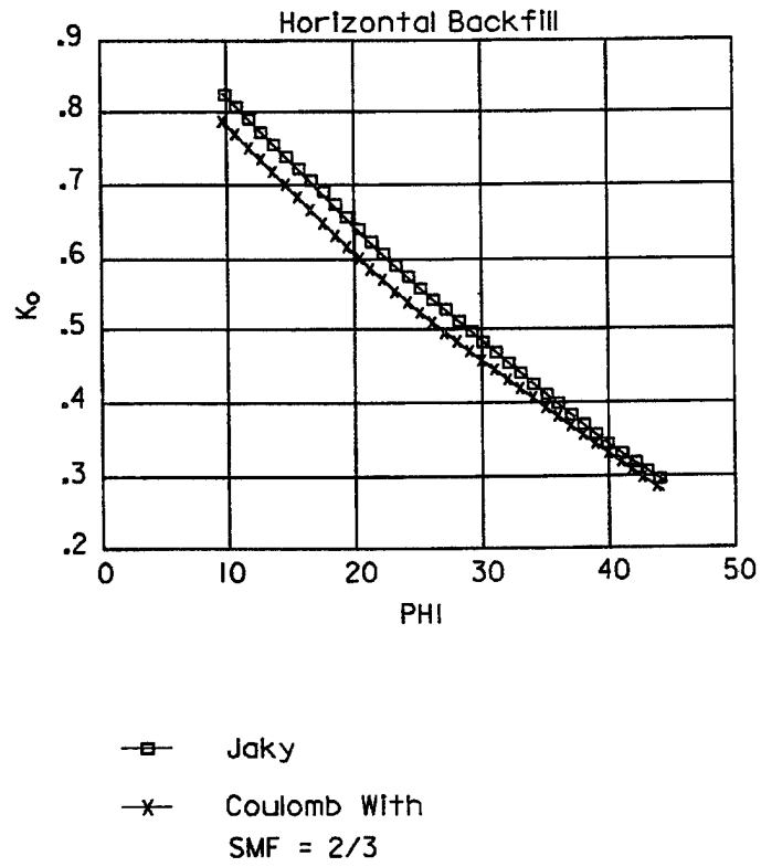
Figure 3-6. At-rest earth pressure coefficients
