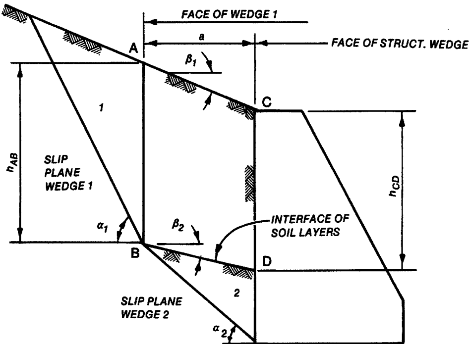
Figure K-1. General condition where shear force is required
