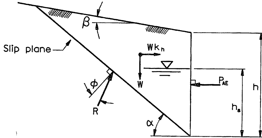
a. Driving wedge
