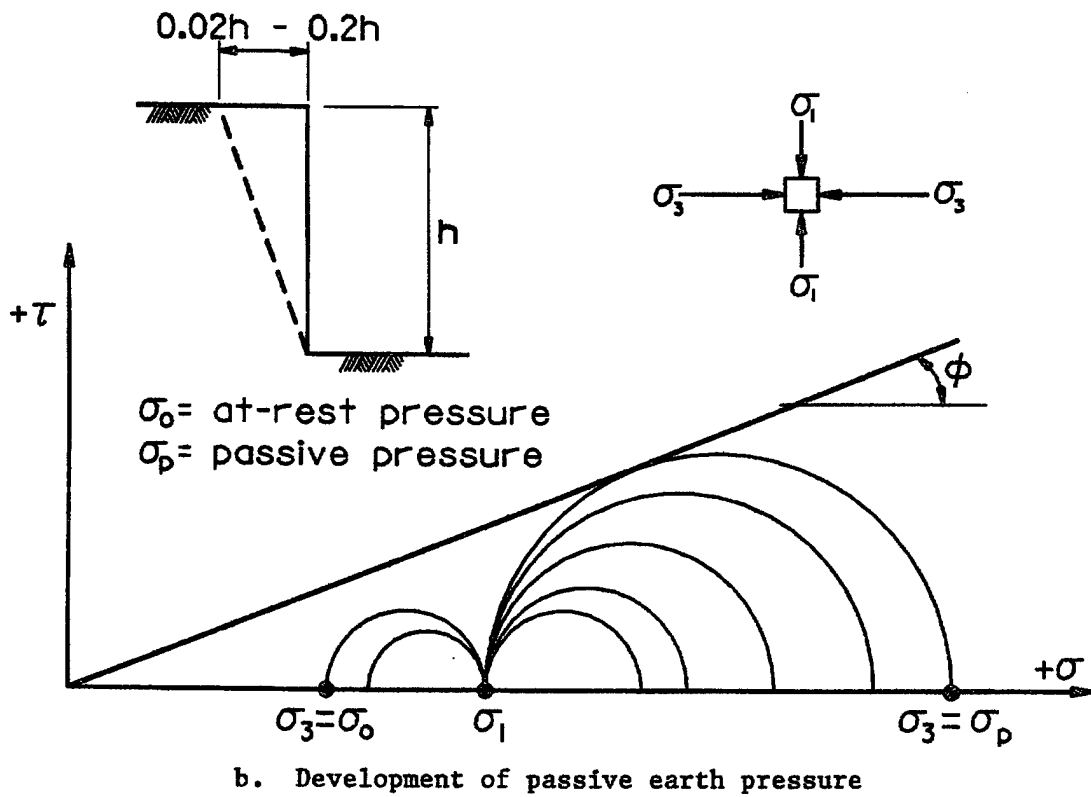
Figure 3-1. Development of earth pressures for a cohesionless material
