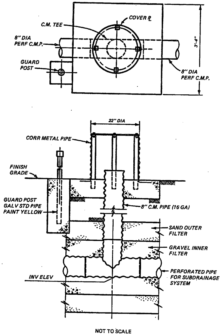
Figure 6-7. Inspection hole for longitudinal drain
