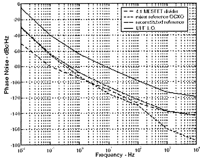
Figure 2. Estimated phase noise for the UHF measurement carrier.
