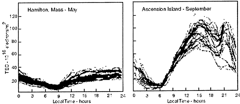
Figure 4. Range of TEC patterns that TechSat21 is likely to encounter.
