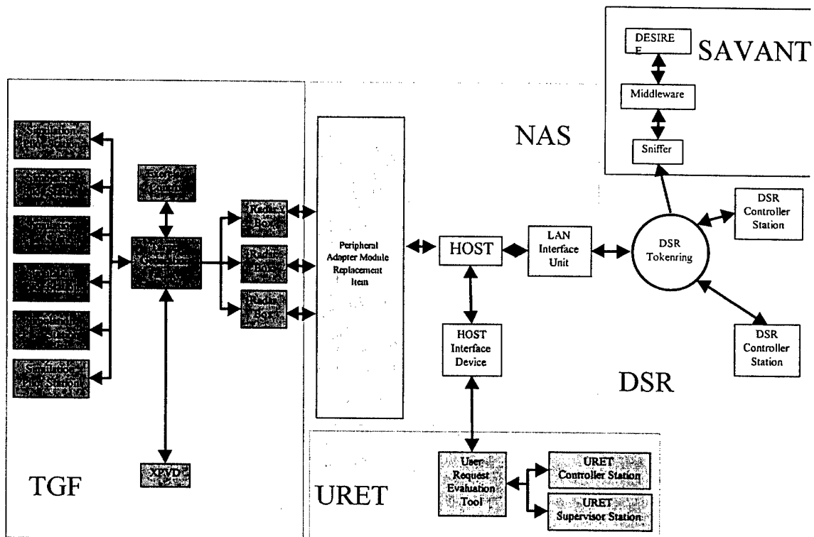
Figure E-2. Schematic layout of DSAR1 hardware and software.
