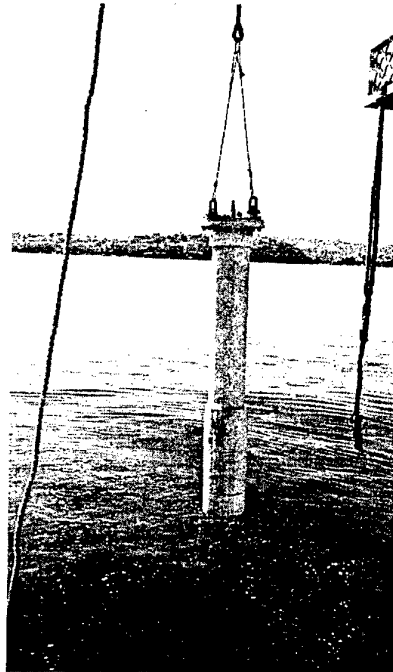
Figure 8. AUSSI probe ready to be launched.
