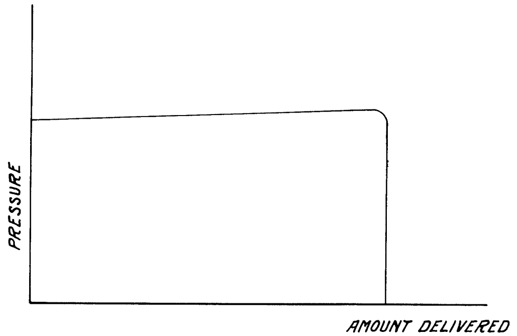
Fig. 15 - Pump-Performance Curve at Constant Speed
