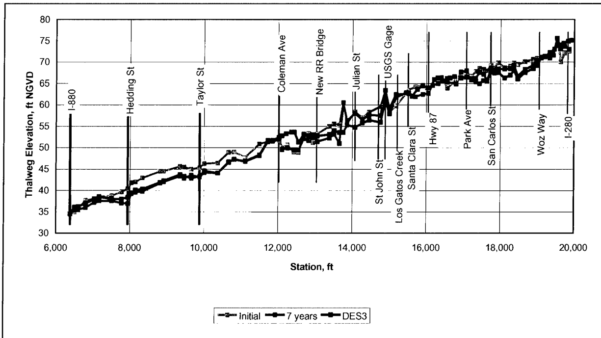
Figure 38. Calculated thalweg elevations after 7-year hydrograph (1992-1999) for existing and project (DES3) conditions
