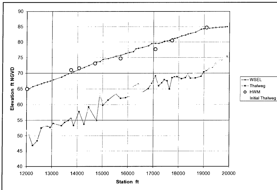
Figure 7. Water-surface elevations calculated with adjusted roughness coefficients. Water-surface elevations estimated 10 January 1995
