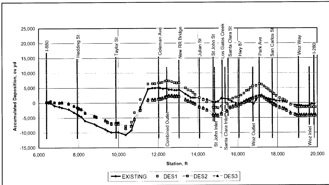
Figure 39. Calculated deposition accumulated from downstream station from 7-year hydrograph (1992-1999)
