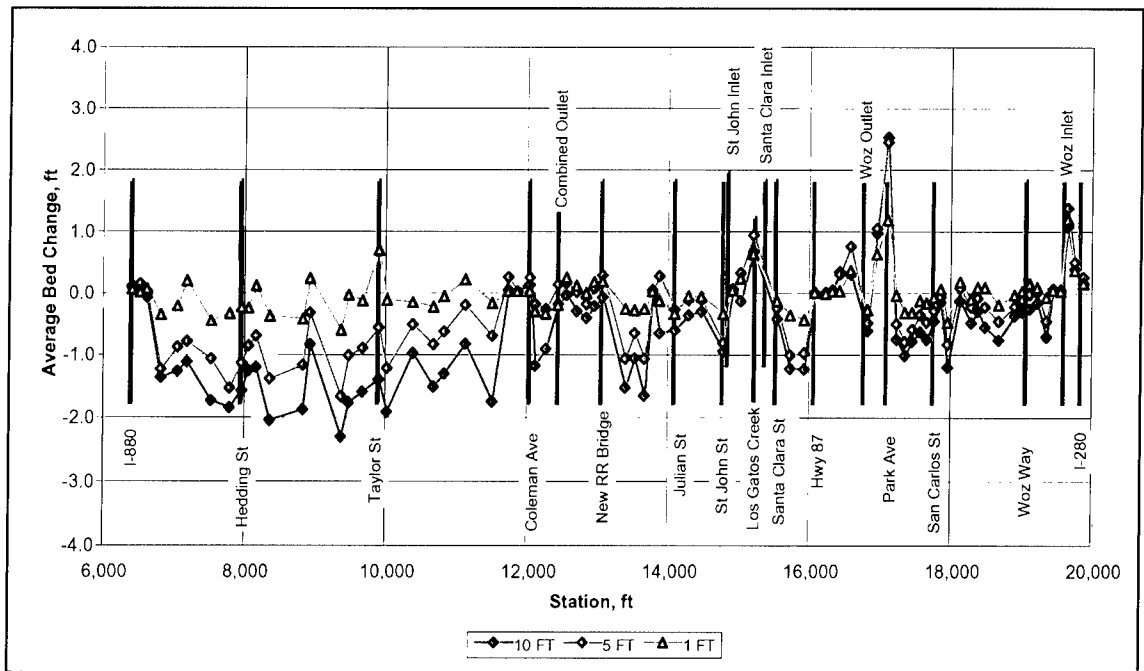
Figure 32. Sensitivity of average bed change to bed-sediment reservoir depth during 7-year hydrograph. Bed-sediment reservoir depths of 10, 5, and 1 ft were evaluated
