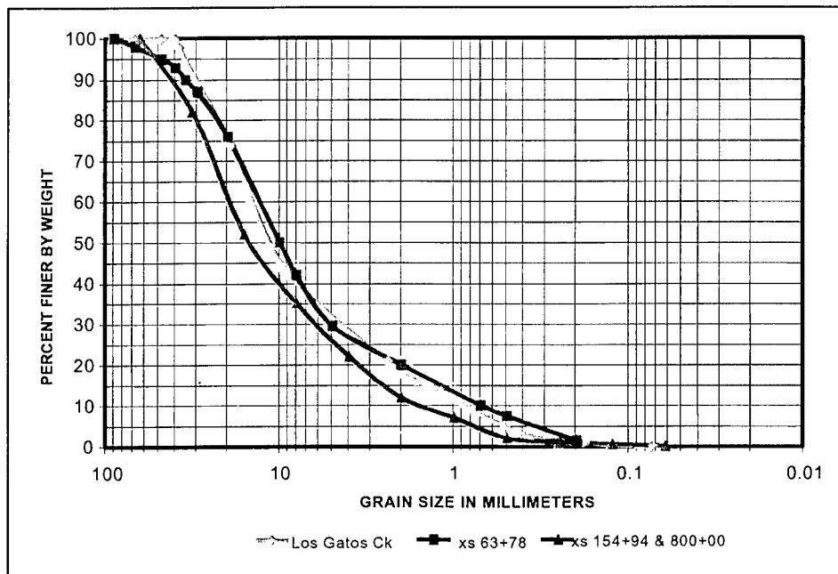
Figure 11. Bed-material gradations used in numerical model study. From 2000 SPK HEC-6 model and WET samples collected in 1987 and 1988
