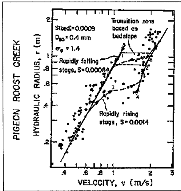
Figure 5-4. Velocity versus hydraulic radius in a mobile bed stream (courtesy of W. M. Keck Laboratories of Hydraulics and Water Resources (Brownlie 1981))
