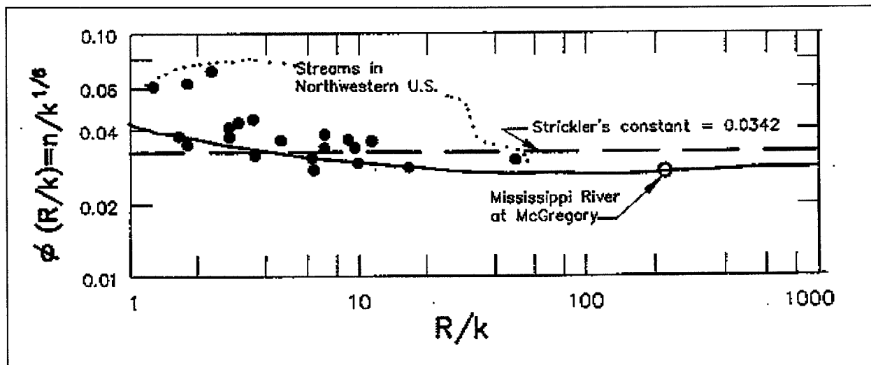
Figure 5-2. The Strickler function (Chow 1959) (courtesy of McGraw-Hill Book Company, Inc.)
