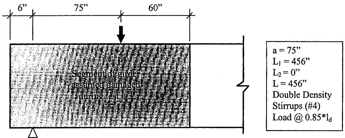
Figure 8.4 Test Configuration 3
