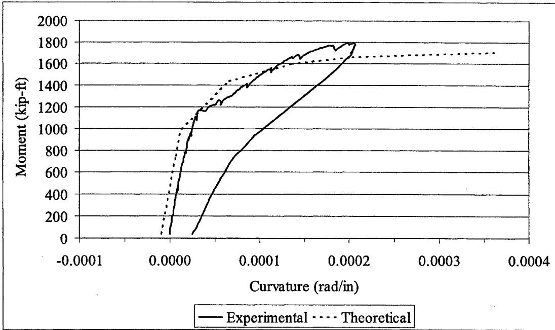
Figure L.18 G1C-East Moment vs. Curvature Plot
