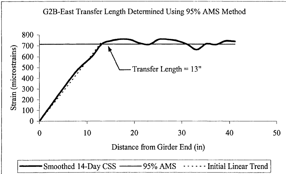
Figure I.18 14-Day Transfer Length Determined for G2B-East
