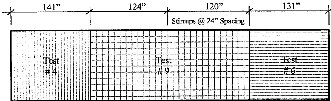
Figure 8.13 Girder Layout C
