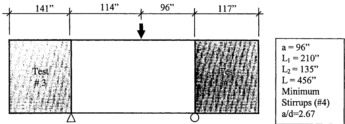
Figure 8.9 Test Configuration 8
