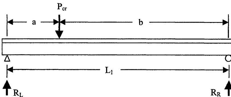
Figure L.2 Diagram Showing Variables for Elastic Deflection Calculations
