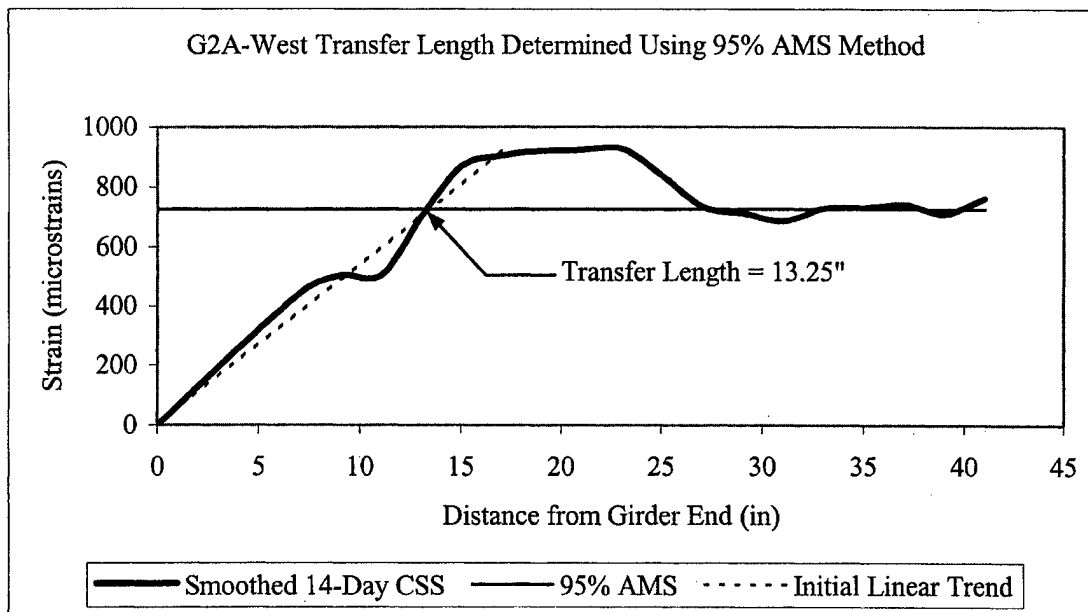
Figure I.16 14-Day Transfer Length Determined for G2A-West
