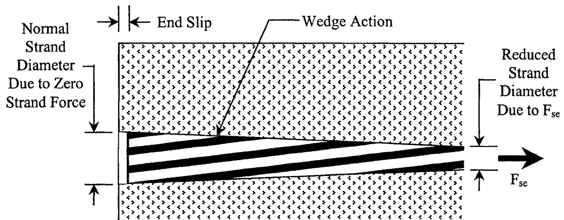
Figure 2.1 Wedge Action Resulting from Hoyer's Effect
