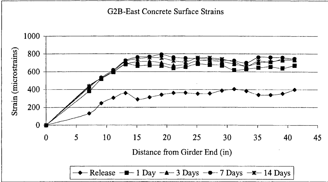
Figure I.17 Concrete Surface Strains for G2B-East
