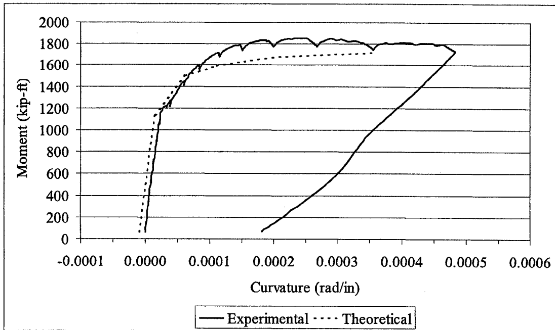
Figure L.26 G2A-West Moment vs. Curvature Plot
