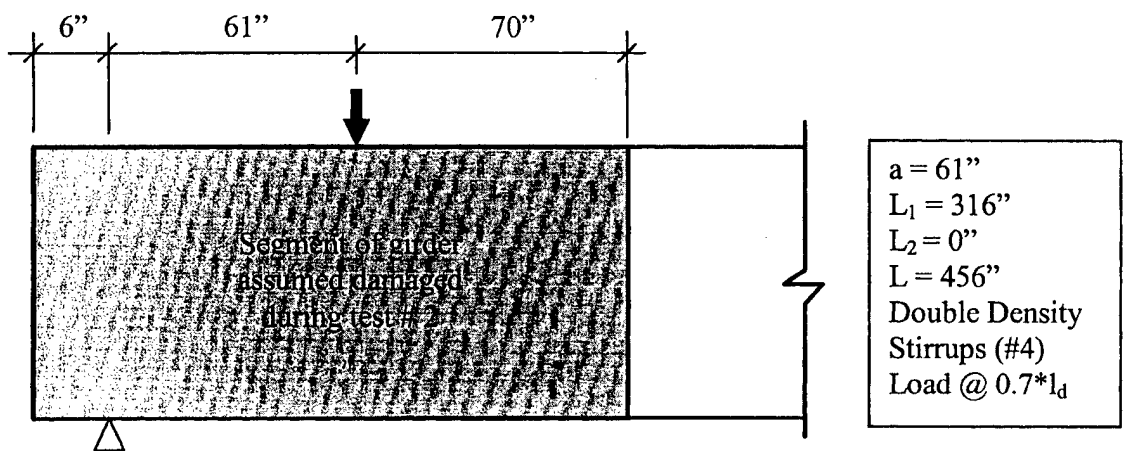
Figure 8.3 Test Configuration 2
