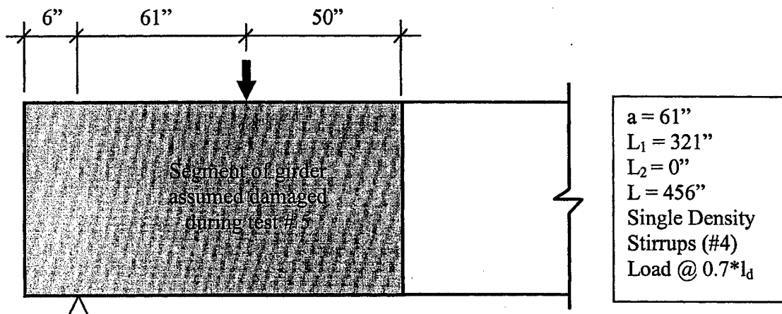
Figure 8.6 Test Configuration 5
