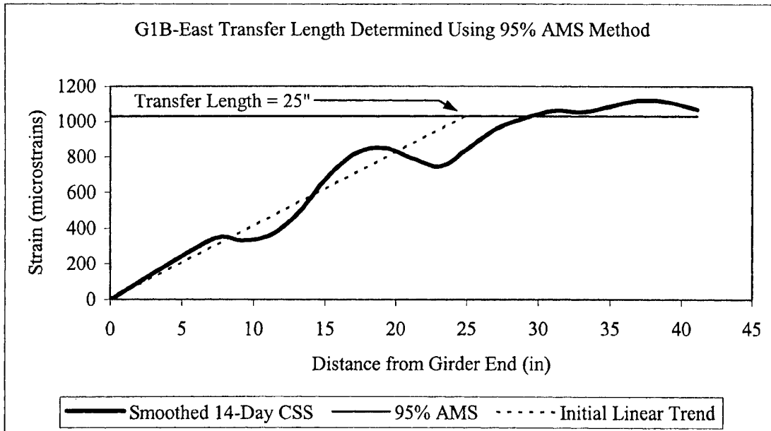
Figure I.6 14-Day Transfer Length Determined for G1B-East
