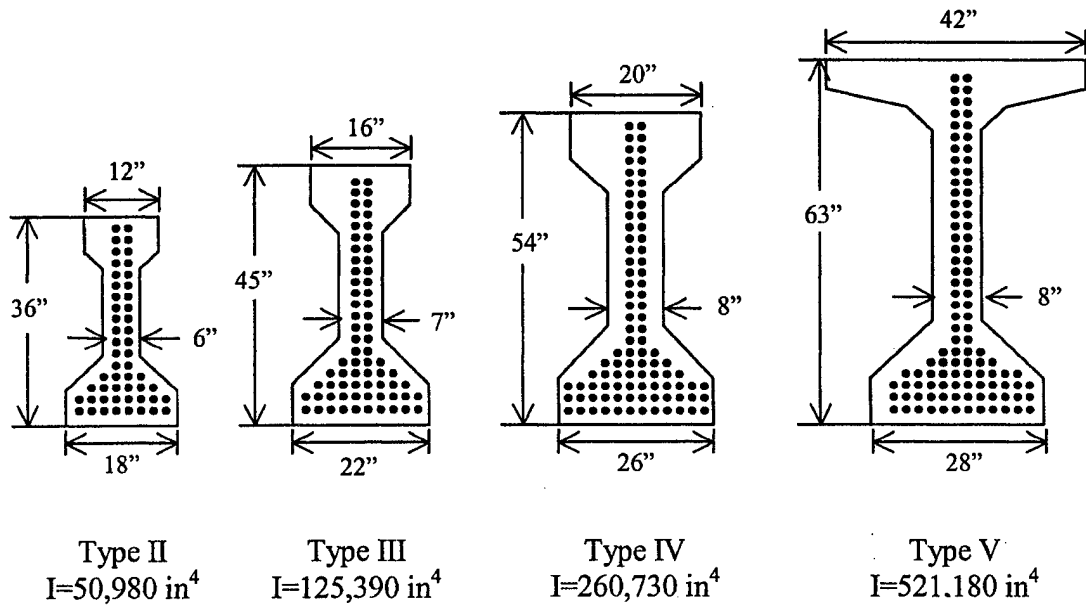
Figure 3.1 AASHTO Type II – V Sections
