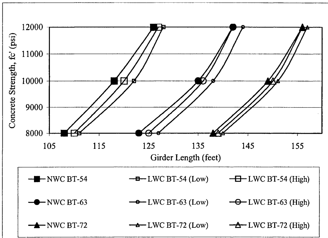
Figure 3.7 Concrete Strength vs. Maximum Length for Bulb-Tee Girders
