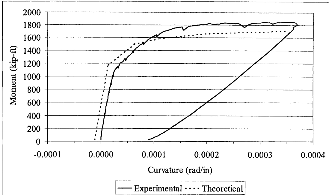
Figure L.24 G2A-East Moment vs. Curvature Plot
