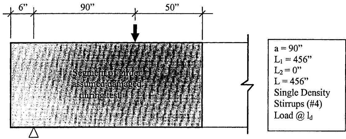
Figure 8.2 Test Configuration 1
