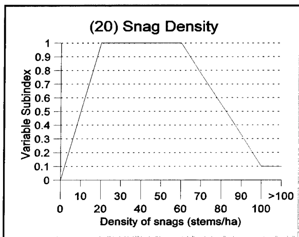
Figure 47. Function 8: Relationship between snag density and functional capacity
