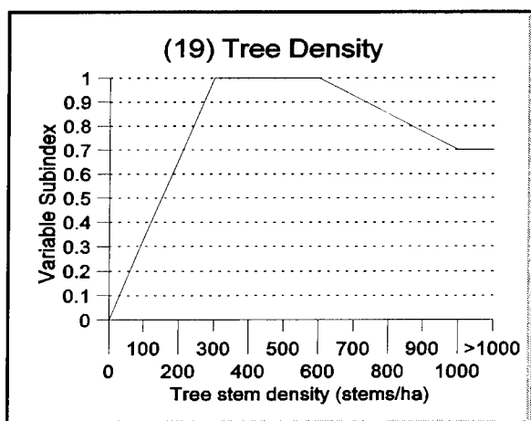
Figure 36. Function 7: Relationship between tree density and functional capacity
