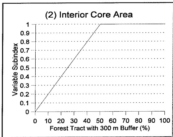
Figure 52. Function 8: Relationship between interior core area and functional capacity
