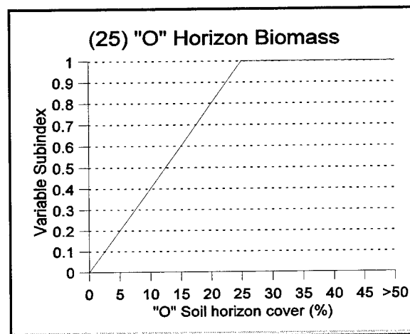
Figure 48. Function 8: Relationship between “O” soil horizon and functional capacity
