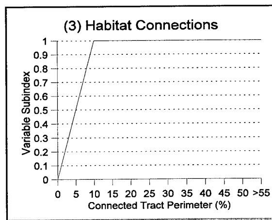
Figure 54. Function 8: Relationship between tract perimeter connections and functional capacity
