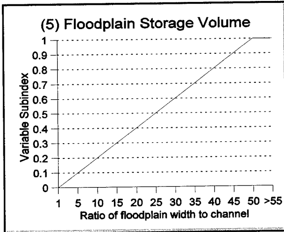
Figure 5. Function 1: Relationship between the ratio of floodplain width to channel width and functional capacity
