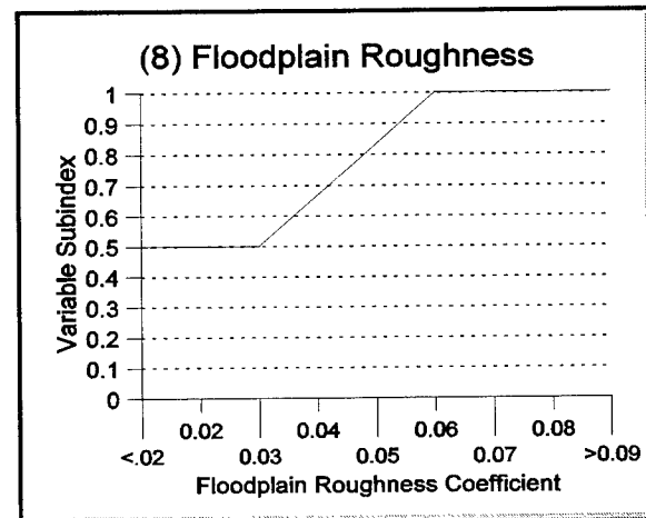
Figure 30. Function 5: Relationship between floodplain roughness and functional capacity
