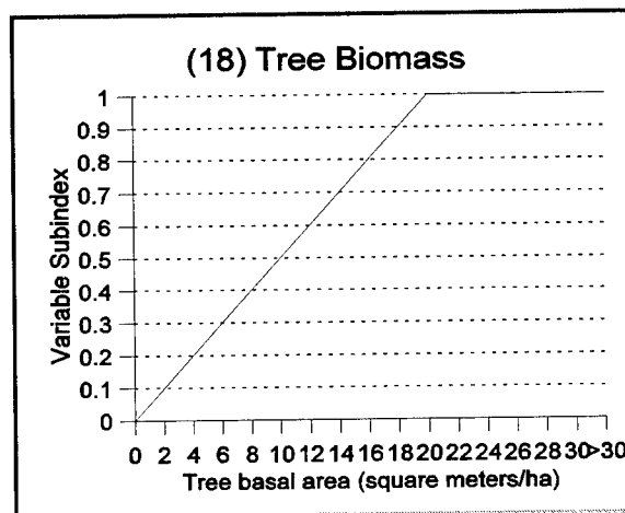
Figure 35. Function 7: Relationship between tree basal area and functional capacity
