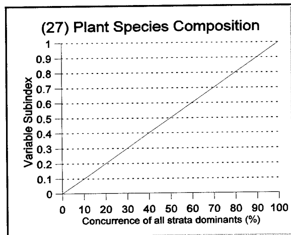
Figure 43. Function 8: Relationship between percent concurrence of strata dominants and functional capacity
