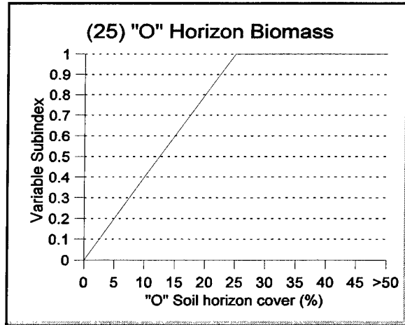
Figure 33. Function 6: Relationship between “O” soil horizon and functional capacity
