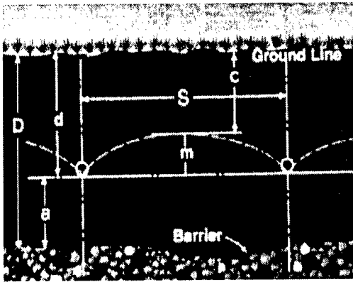
Example tile drainage system
