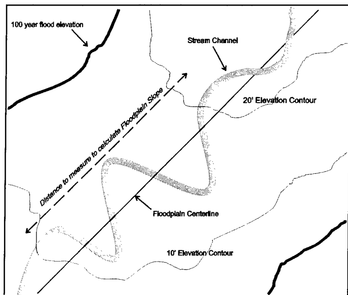
Figure 6. Measuring floodplain slope
