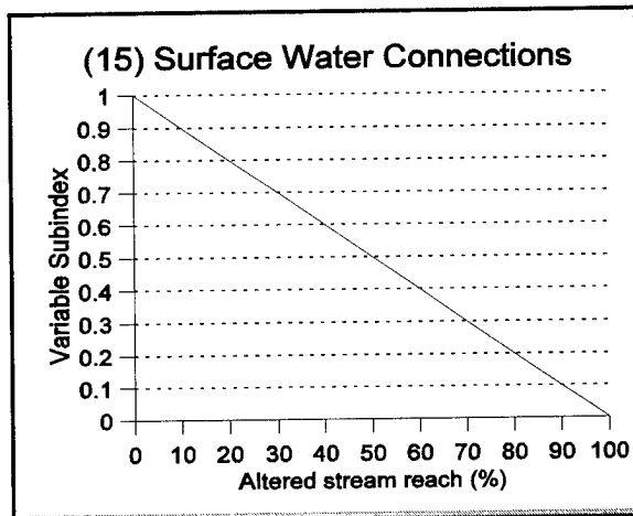
Figure 32. Function 6: Relationship between altered stream reach and functional capacity
