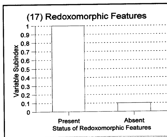
Figure 24. Function 4: Relationship between status of redoximorphic features and functional capacity
