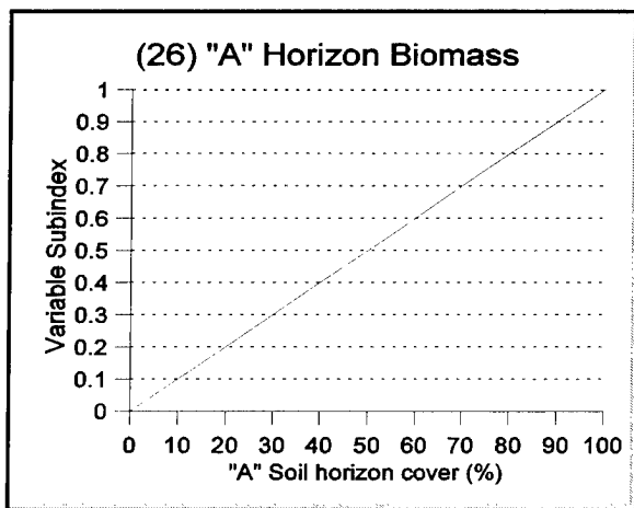
Figure 26. Function 4: Relationship between “A” soil horizon and functional capacity
