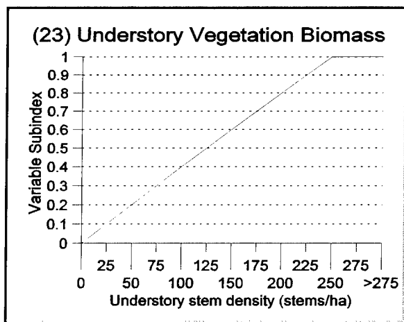
Figure 16. Function 3: Relationship between understory vegetation stem density and functional capacity
