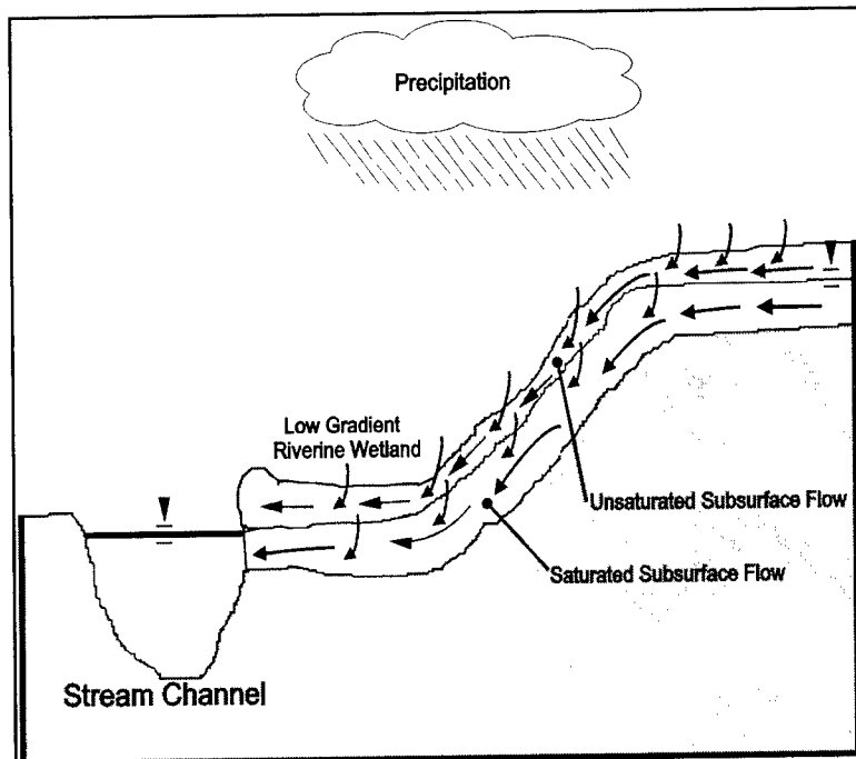
Figure 9. Movement of water down the hydraulic gradient from uplands, through wetlands, and into adjacent stream channels
