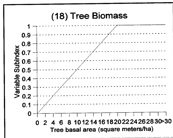
Figure 15. Function 3: Relationship between tree basal area and functional capacity
