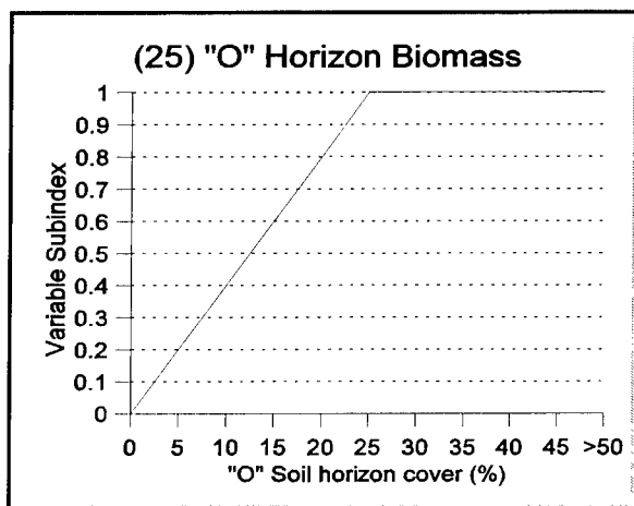
Figure 18. Function 3: Relationship between “O” soil horizon and functional capacity
