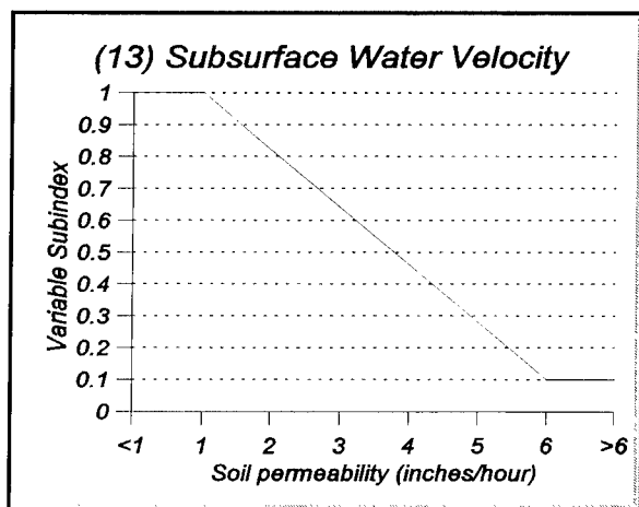
Figure 10. Function 2: Relationship between soil permeability and functional capacity
