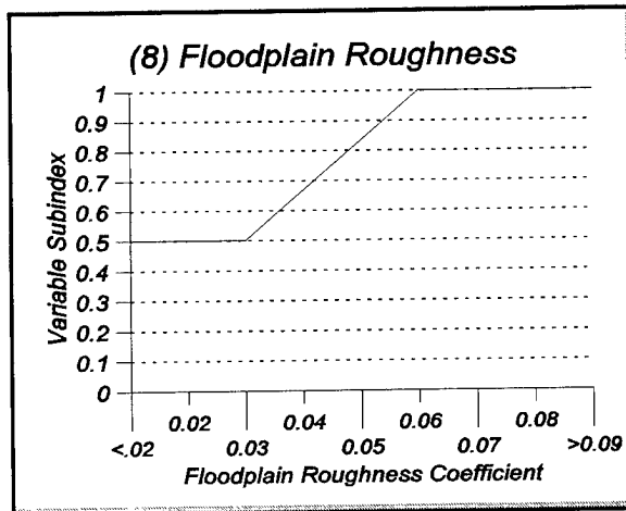
Figure 8. Function 1: Relationship between floodplain roughness and functional capacity
