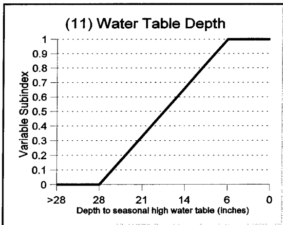
Figure 39. Function 7: Relationship between depth to seasonal high water table and functional capacity
