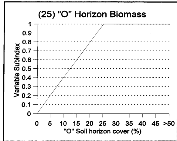
Figure 25. Function 4: Relationship between “O” soil horizon and functional capacity
