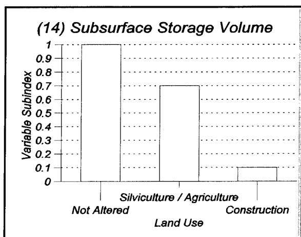
Figure 13. Function 2: Relationship between land use activities and functional capacity
