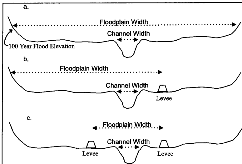
Figure 4. Determining floodplain width and channel width
