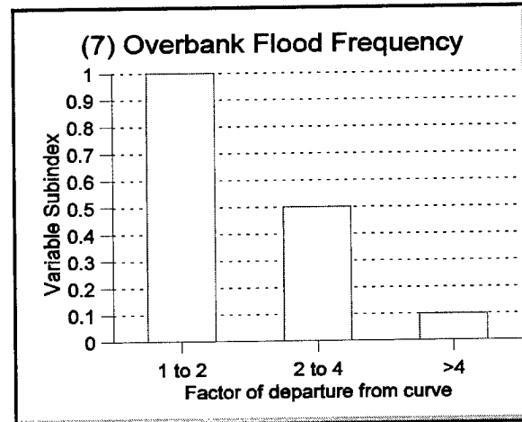
Figure 21. Function 4: Relationship between channel cross-sectional area and functional capacity
