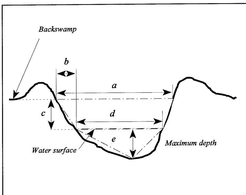
Figure C6. Five measurements on cross-sectional area
