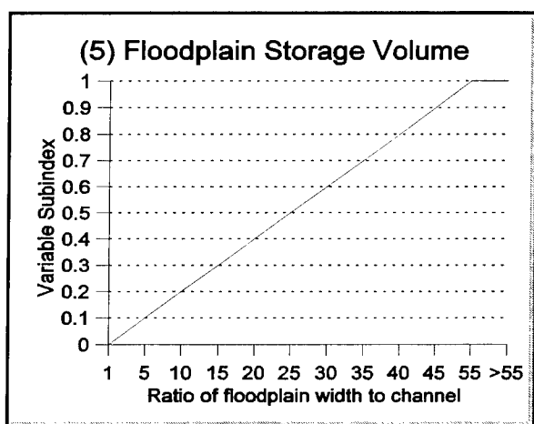
Figure 28. Function 5: Relationship between the ratio of floodplain width to channel width and functional capacity
