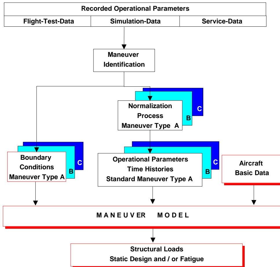
Fig. 1: Procedure Overview
