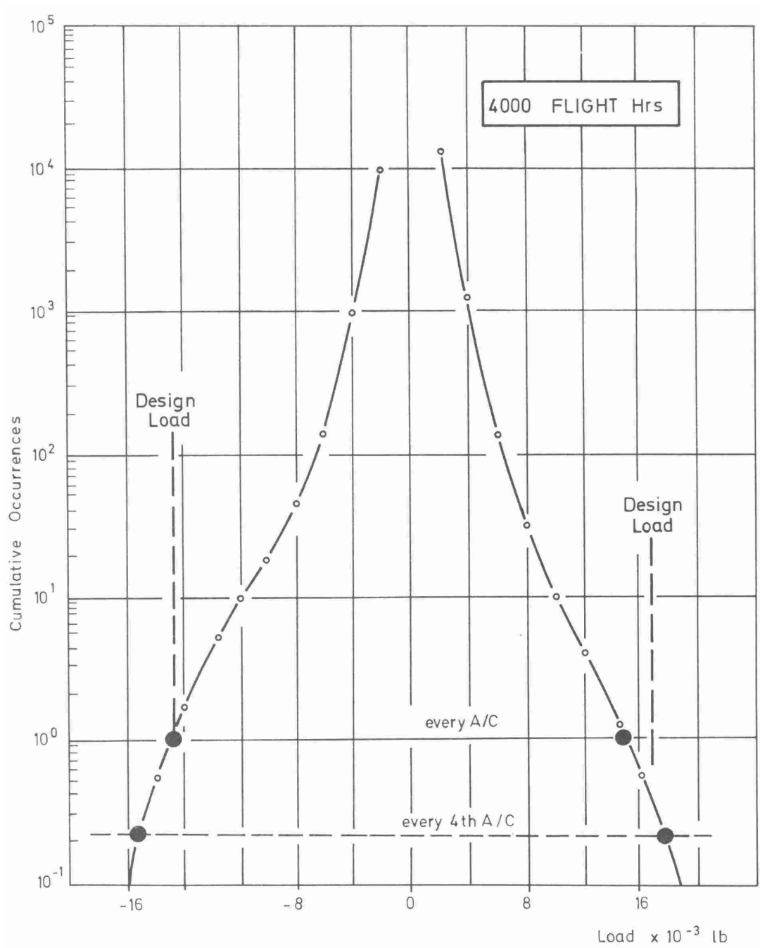
FIG. 2 CUMULATIVE OCCURANCES OF VERTICAL STABILIZER LOADS
