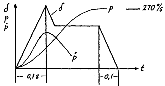
Fig. 4 Stick Input of rolling cases of 8861 A
