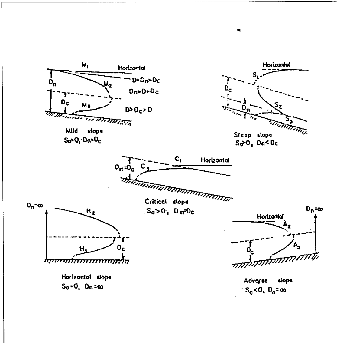
Figure 2-5. Classification of steady flow profiles
