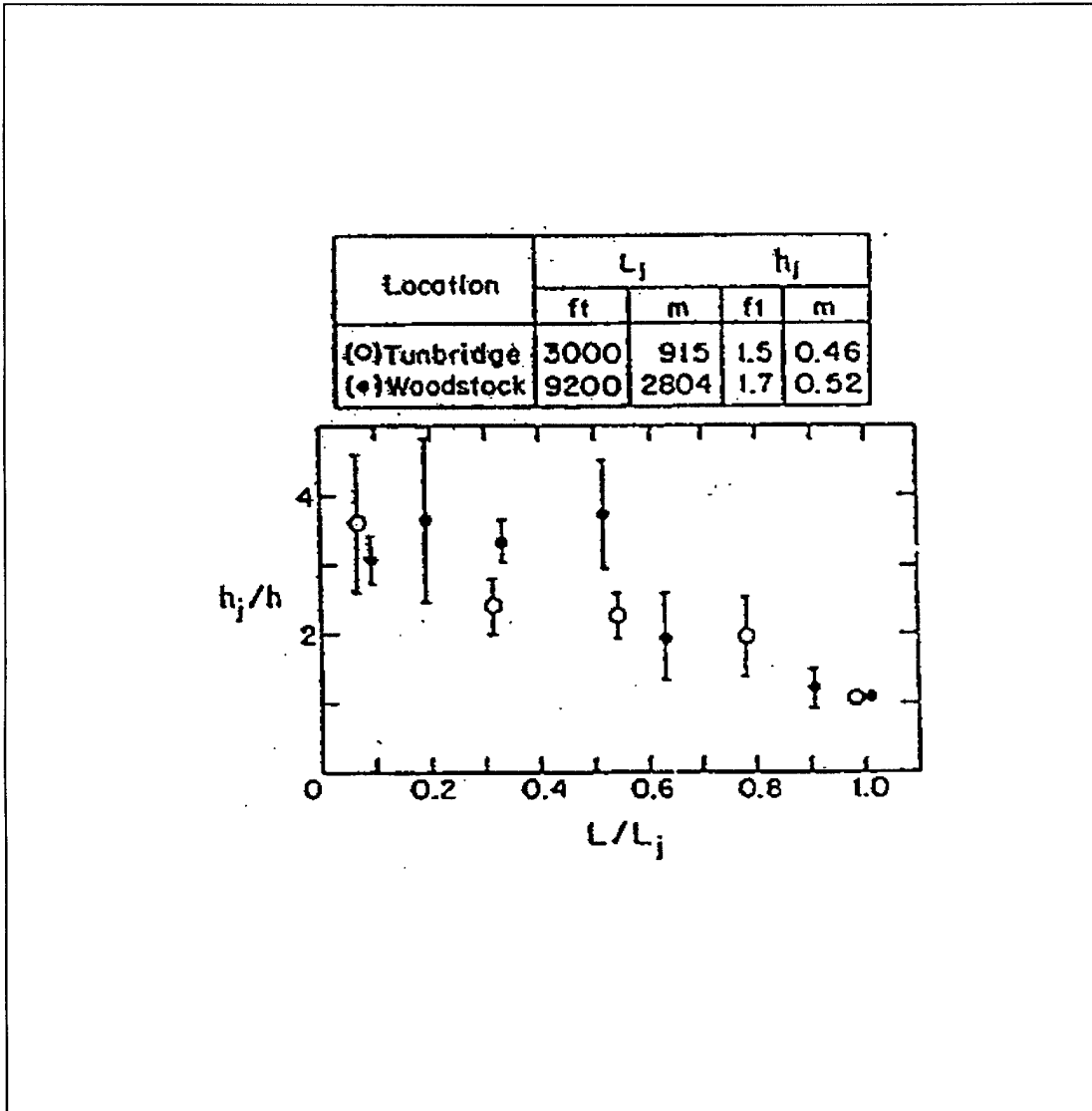
Figure 6-13. Nondimensional ice jam thickness versus its relative length (narrow, steep rivers)
