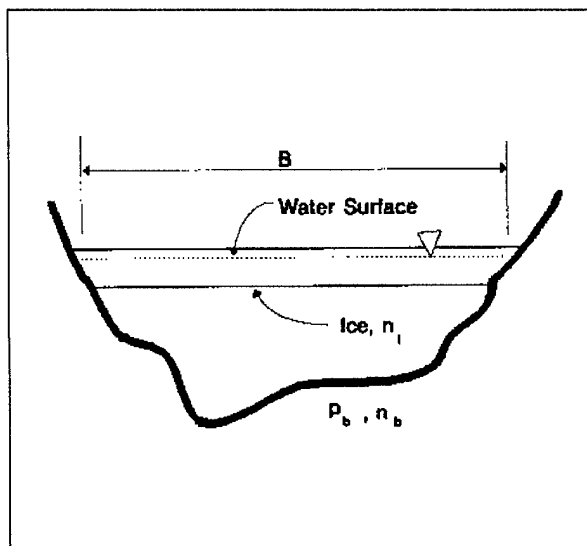
Figure 6-12. Hydraulic parameters of an ice-covered stream
