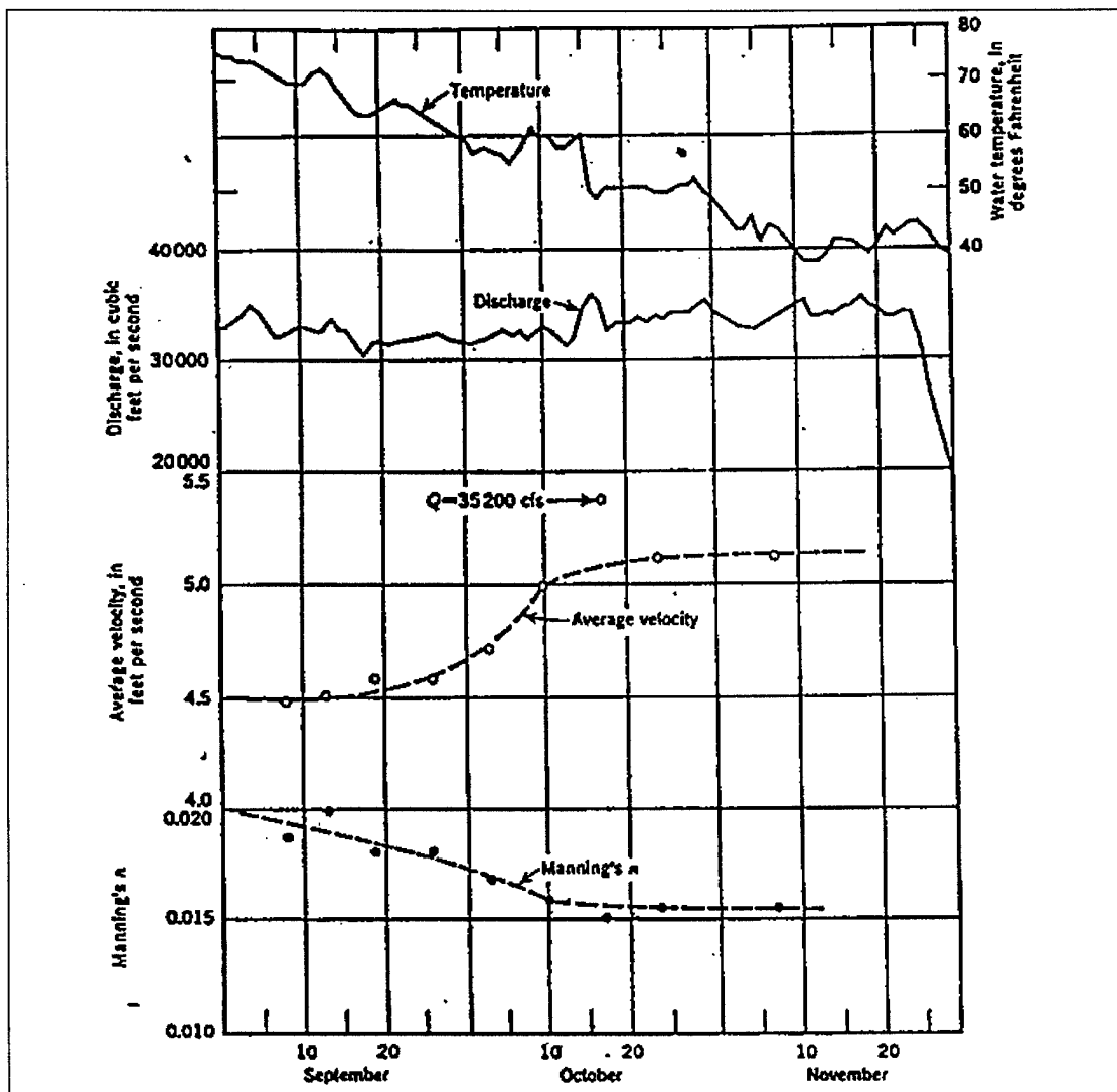
Figure D-17. Variation of water temperature, discharge, average velocity, and Manning's n for Missouri River at Omaha, Neb., during fall of 1966 (U.S. Army Corps of Engineers 1969)
