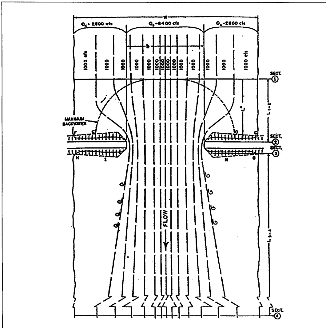
Figure 6-5. Flow lines for typical normal bridge crossing
