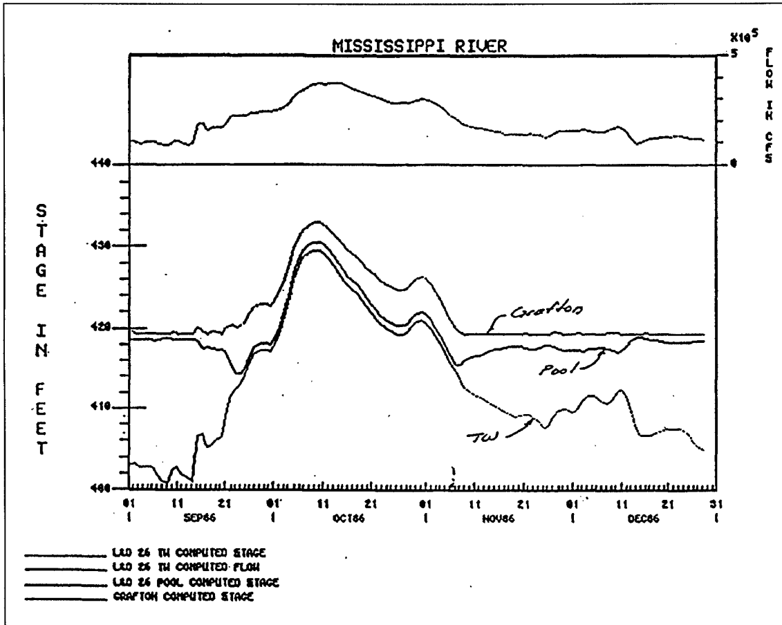
Figure D-6. Pool, tailwater, and control point hydrographs at Lock and Dam 26
