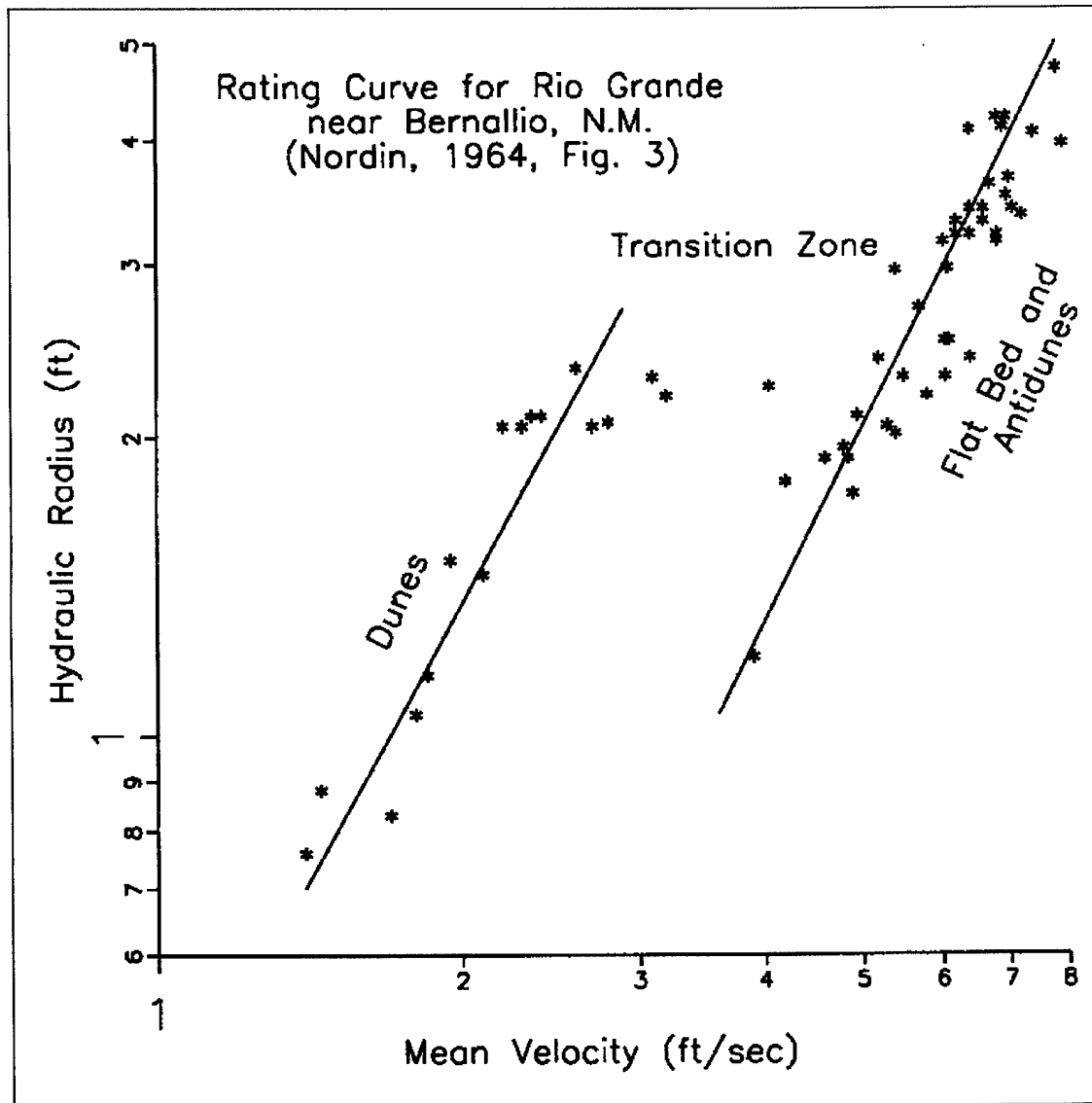
Figure 3-1. Discontinuous rating curve
