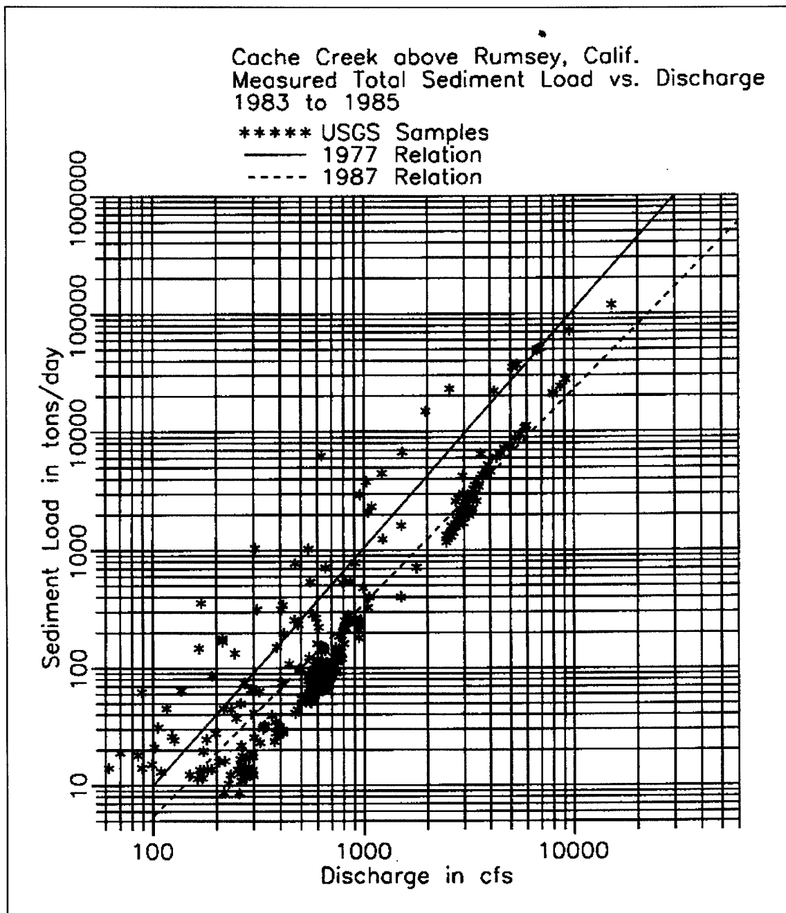
Figure 7-8. Sediment-discharge rating curve
