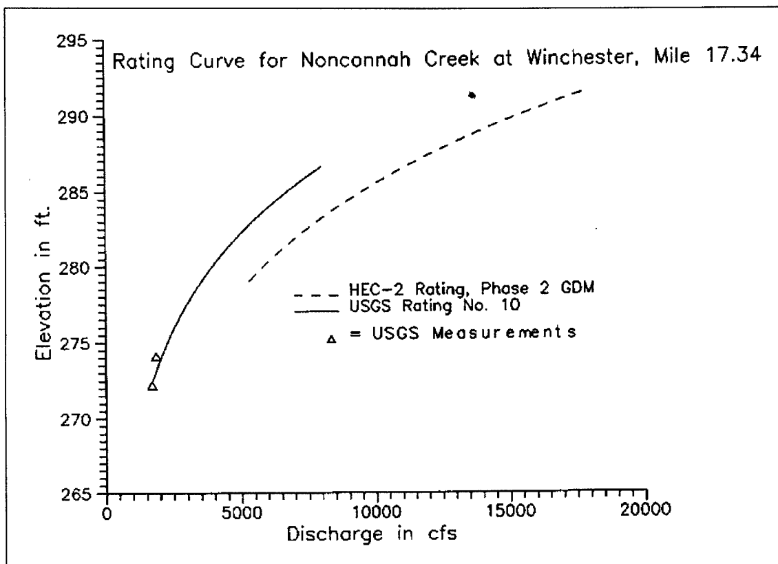
Figure 7-3. Rating curve at a gage
