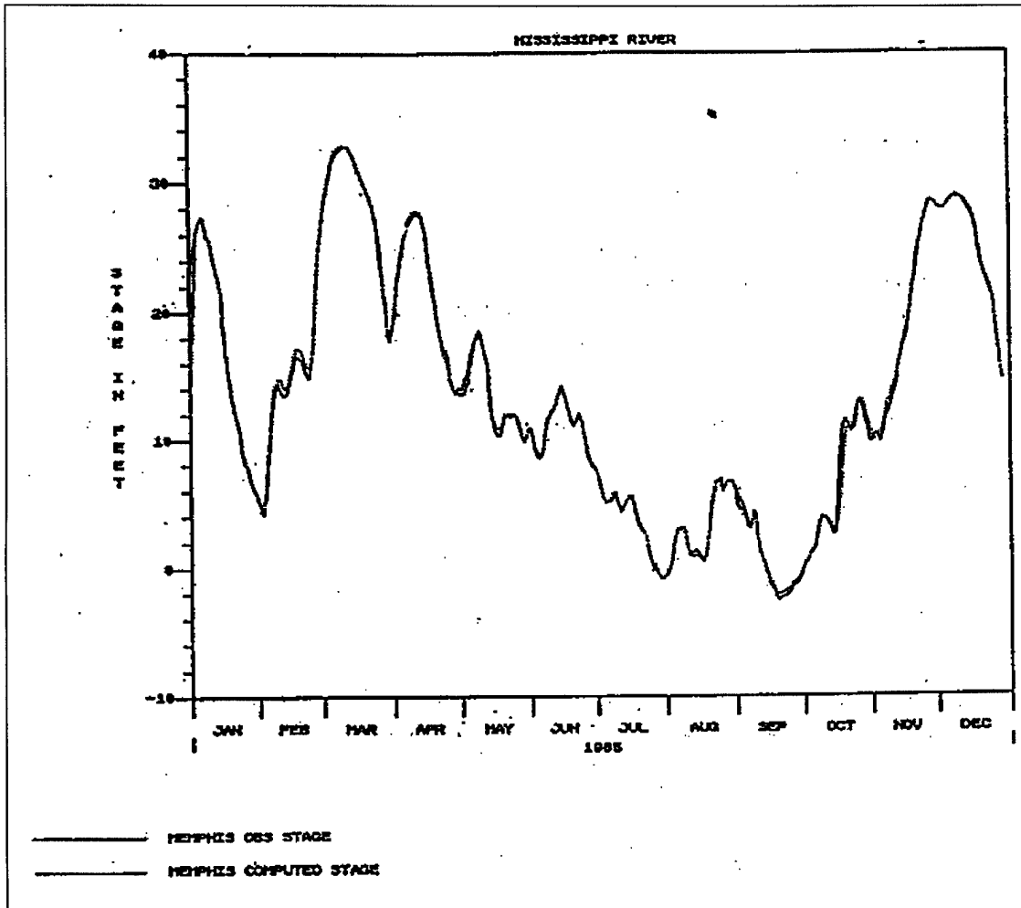
Figure 5-5. Reproduction of Stage at Memphis from Stages Routed from Cairo, 220 Miles Upstream
