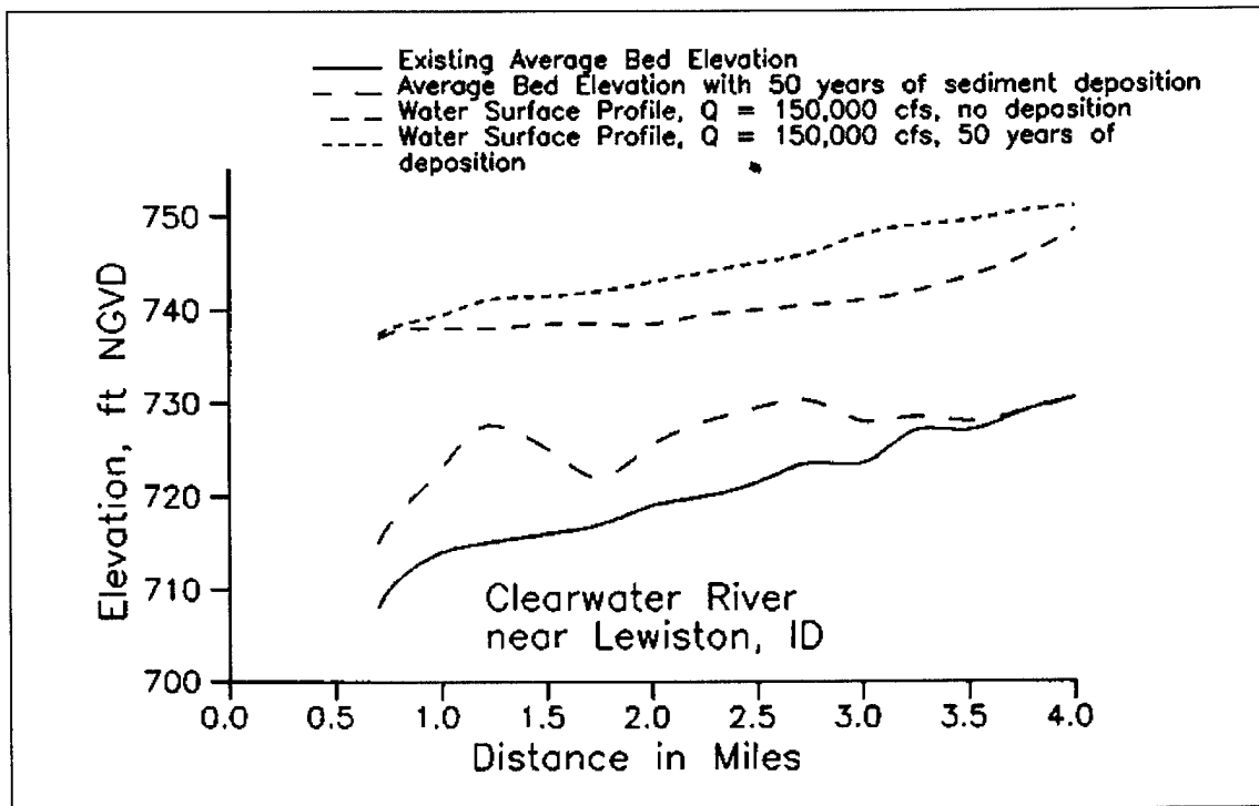
Figure 7-13. Water surface and bed surface profiles
