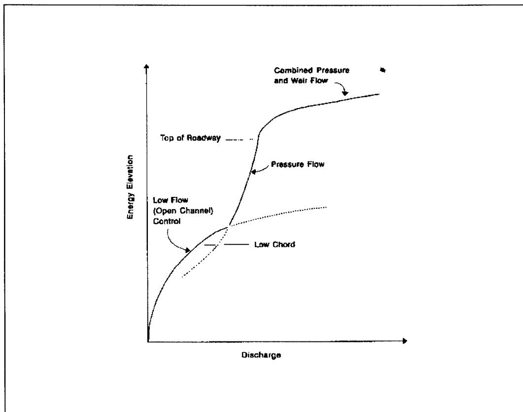
Figure 6-7. Typical discharge rating curve for bridge culvert
