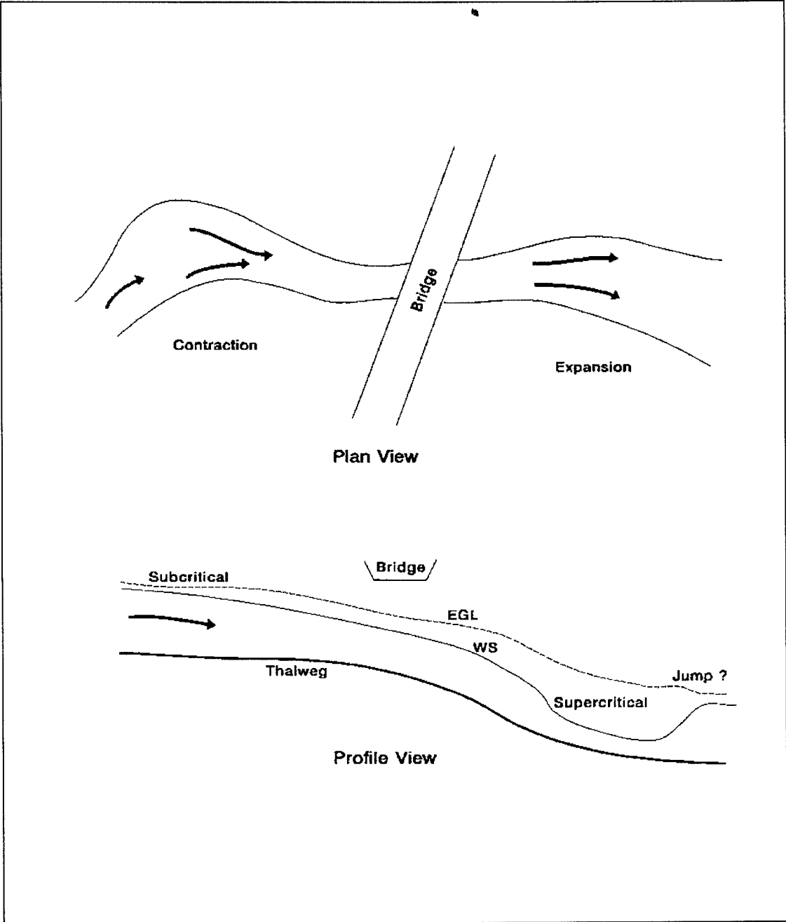
Figure 2-7. Varying flow classification along a channel
