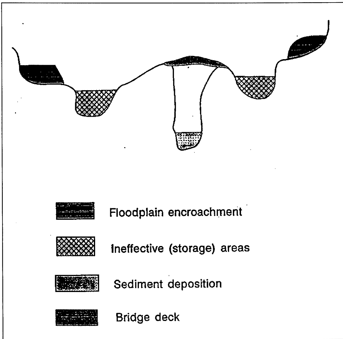
Figure 6-9. Types of effective flow options
