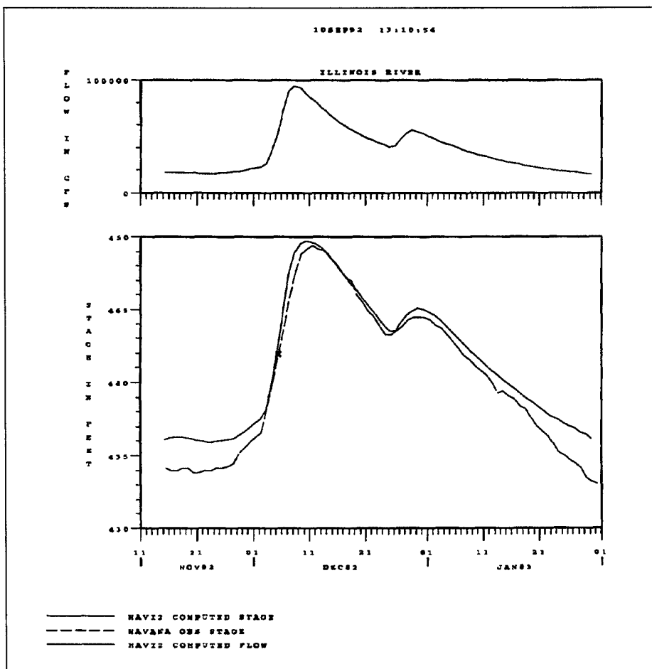
Figure 5-12. Hydrographs for the Illinois River at Havana after initial calibration
