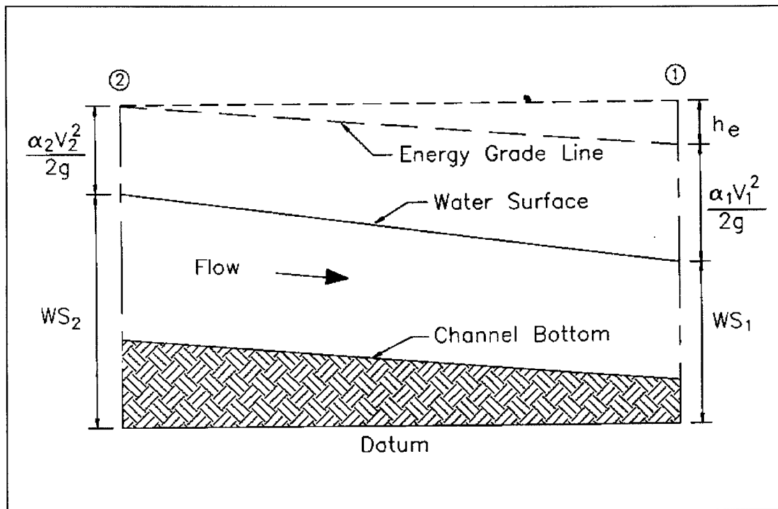
Figure 6-1. Open channel energy relationships
