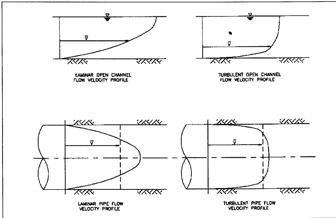
Figure 2-2. Laminar and turbulent velocity profiles
