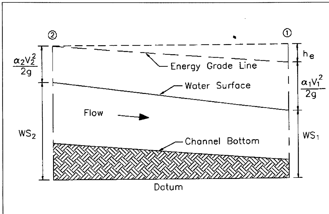
Figure 2-6. Open channel energy relationships
