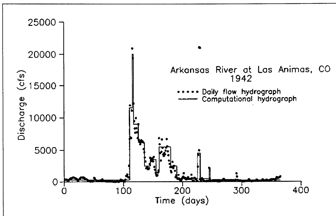
Figure 7-7. Water discharge histogram
