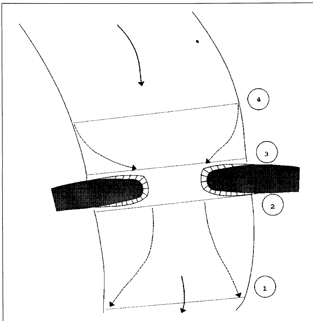
Figure 6-8. Cross section locations in the vicinity of bridges
