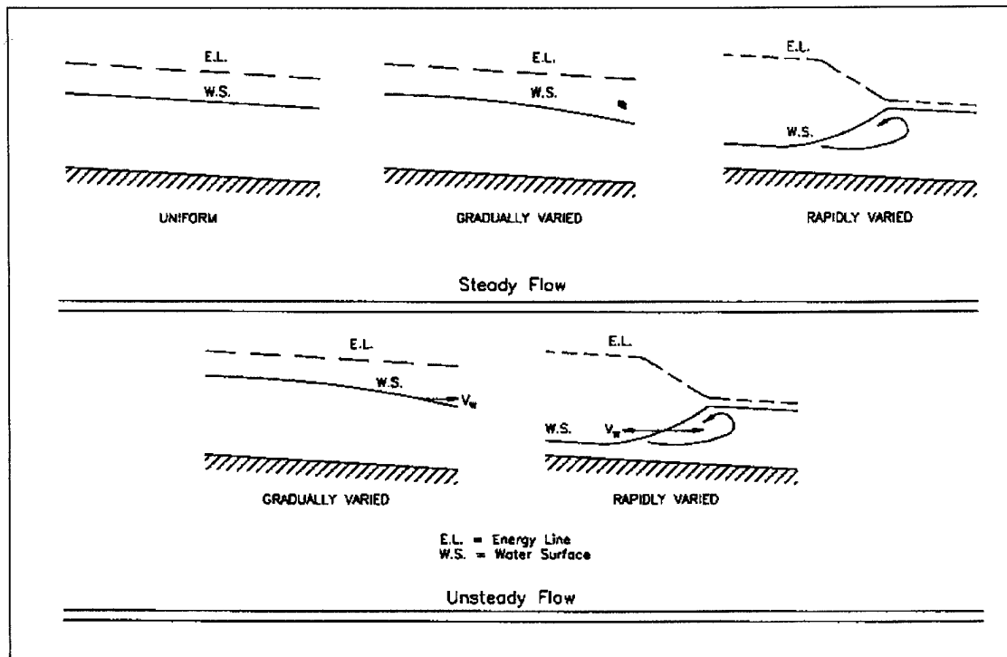
Figure 2-4. Some types of open-channel flow
