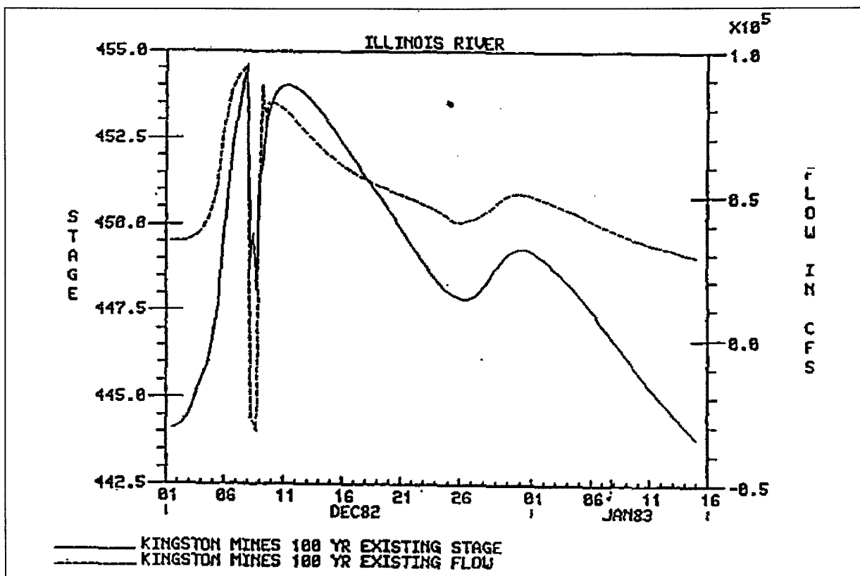
Figure D-13. Flow hydrographs for the Illinois River at Kingston Mines
