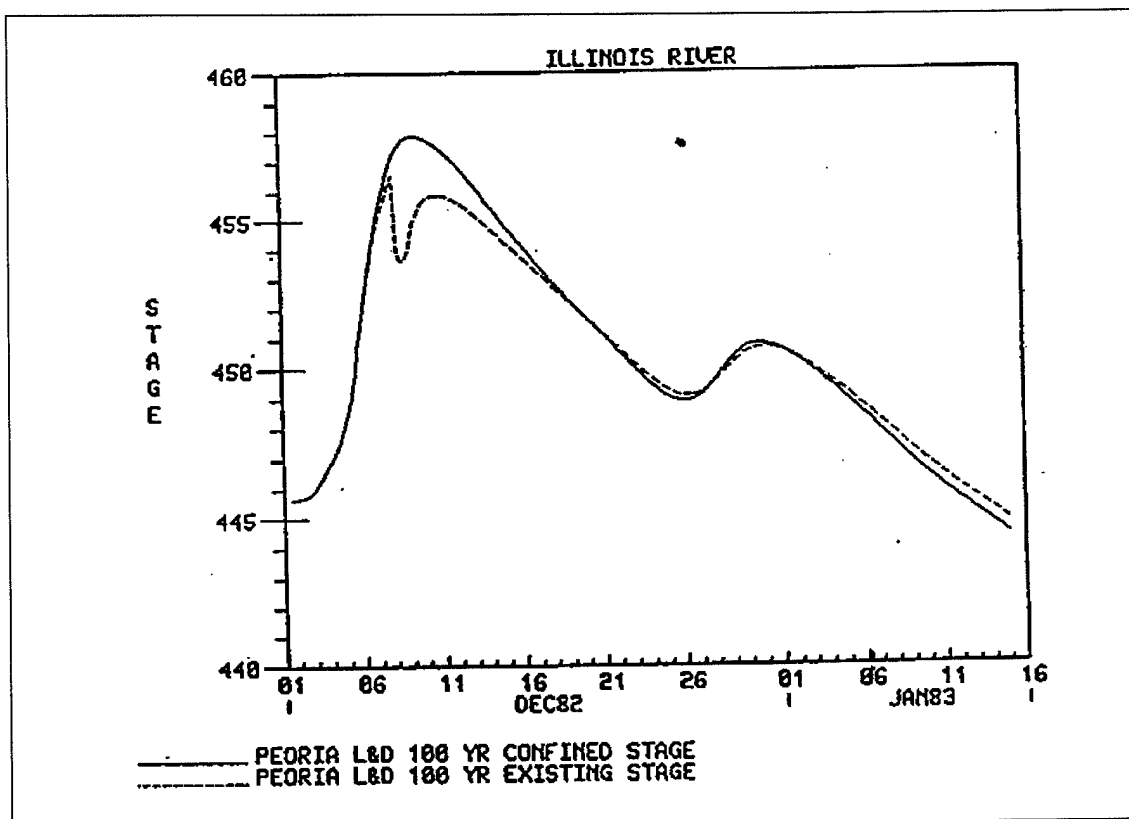
Figure D-9. Stage hydrographs for the Illinois River at Peoria with and without failures
