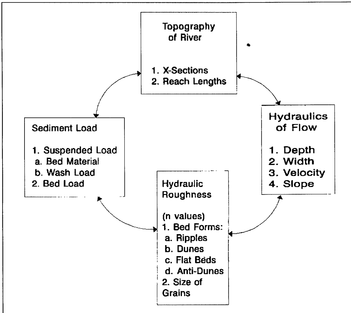
Figure 7-2. Movable bed model
