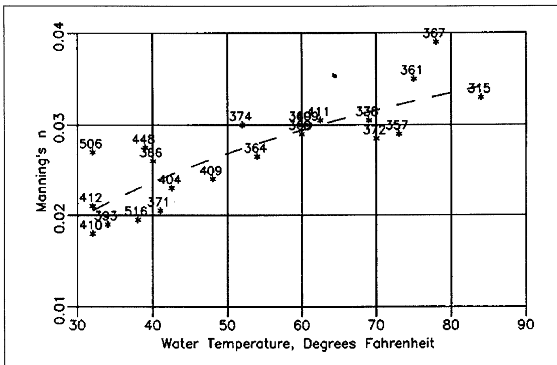
Figure D-15. Plot of Manning's friction factor n against water temperature for Middle Loup River at Dunning, Neb. (Colby and Scott 1965)
