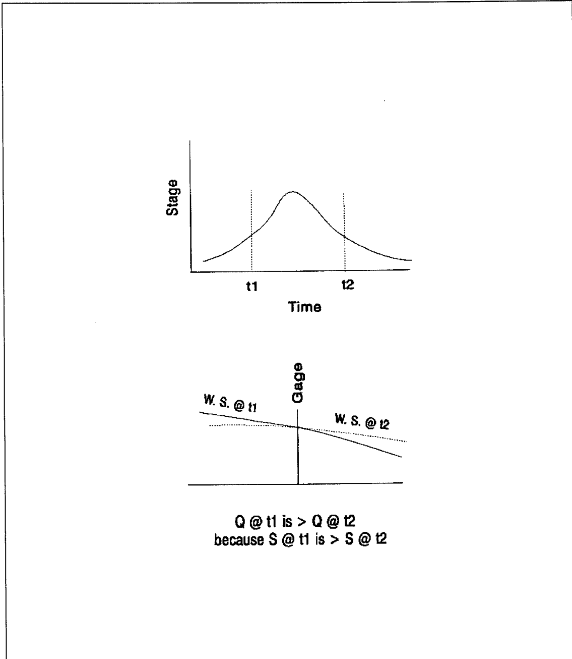
Figure 5-20. Explanation for looped rating curve effect
