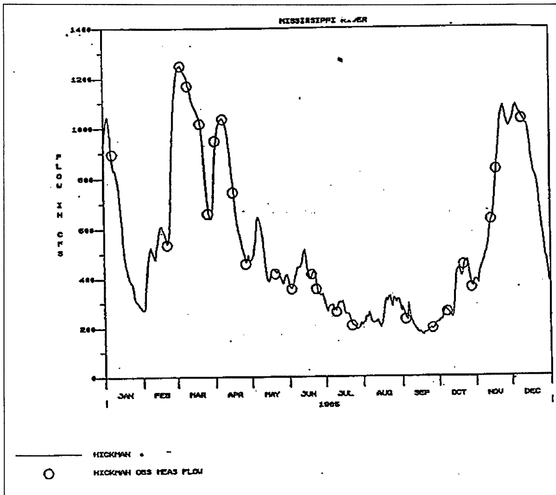
Figure 5-4. Computed versus observed flow at Hickman
