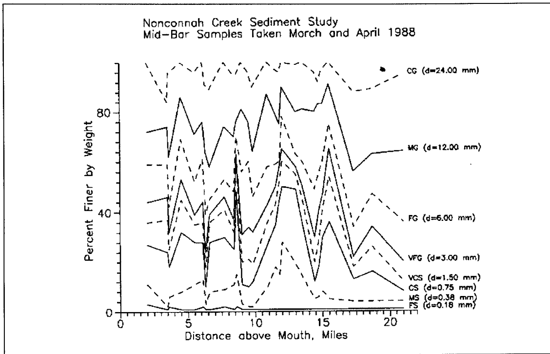
Figure 7-6. Bed surface gradation based on midbar samples
