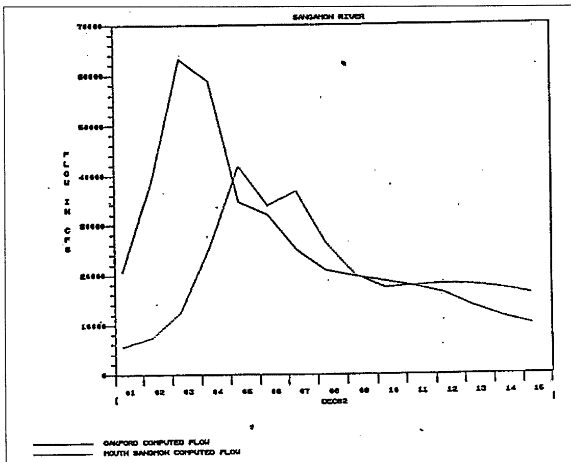
Figure 5-2. Discharge hydrograph at the oakford gage at the mouth of the Sangmon River
