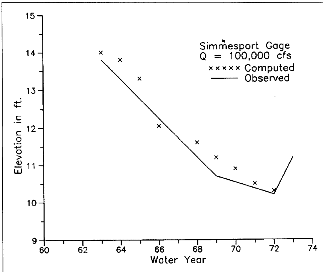
Figure 7-14. Water surface trend plot (specific gage plot)
