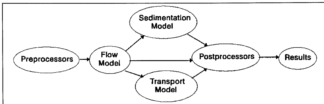
Figure 7-15. TABS-2 schematic
