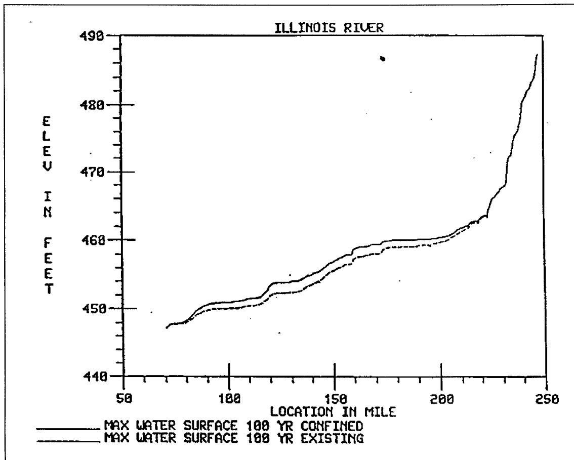
Figure D-10. The 100-yr maximum water surface along the Illinois River with and without levee failure
