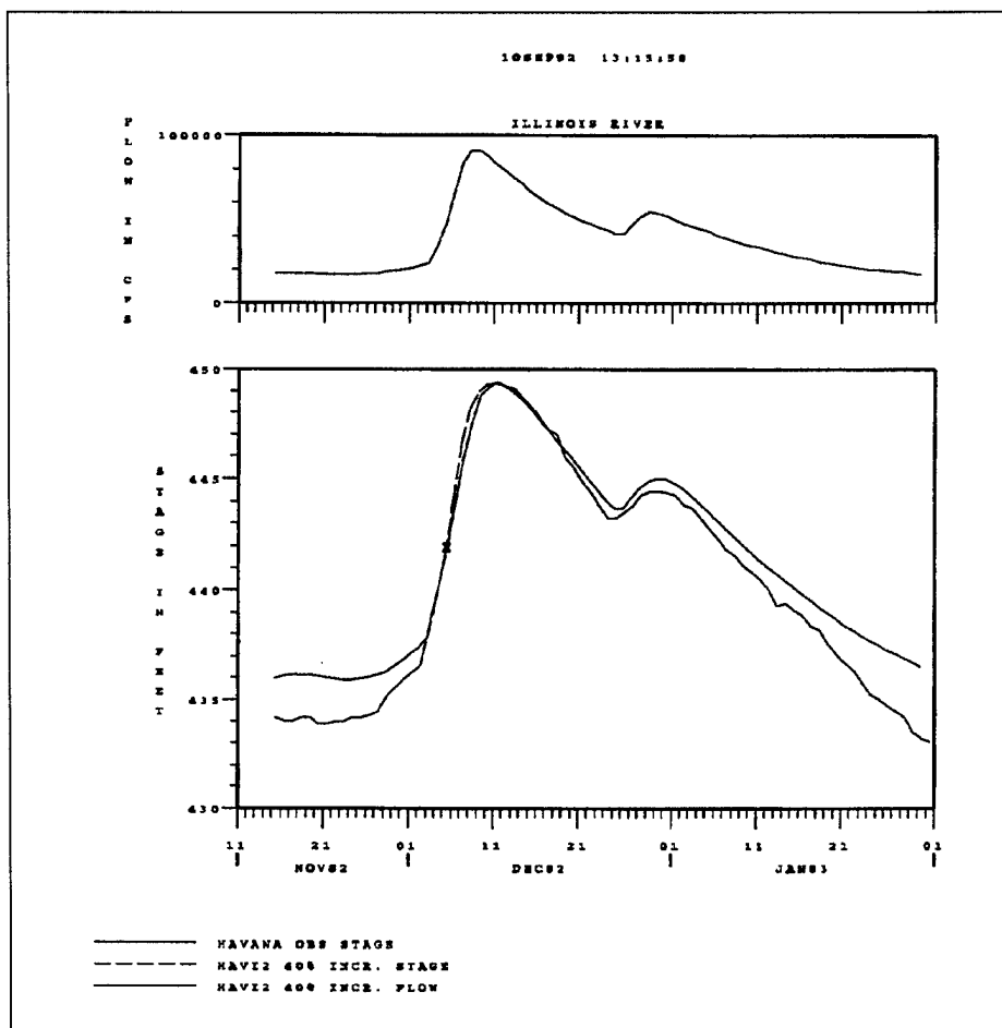
Figure 5-14. Hydrographs for the Illinois River at Havana with overbank storage increased by 40 percent
