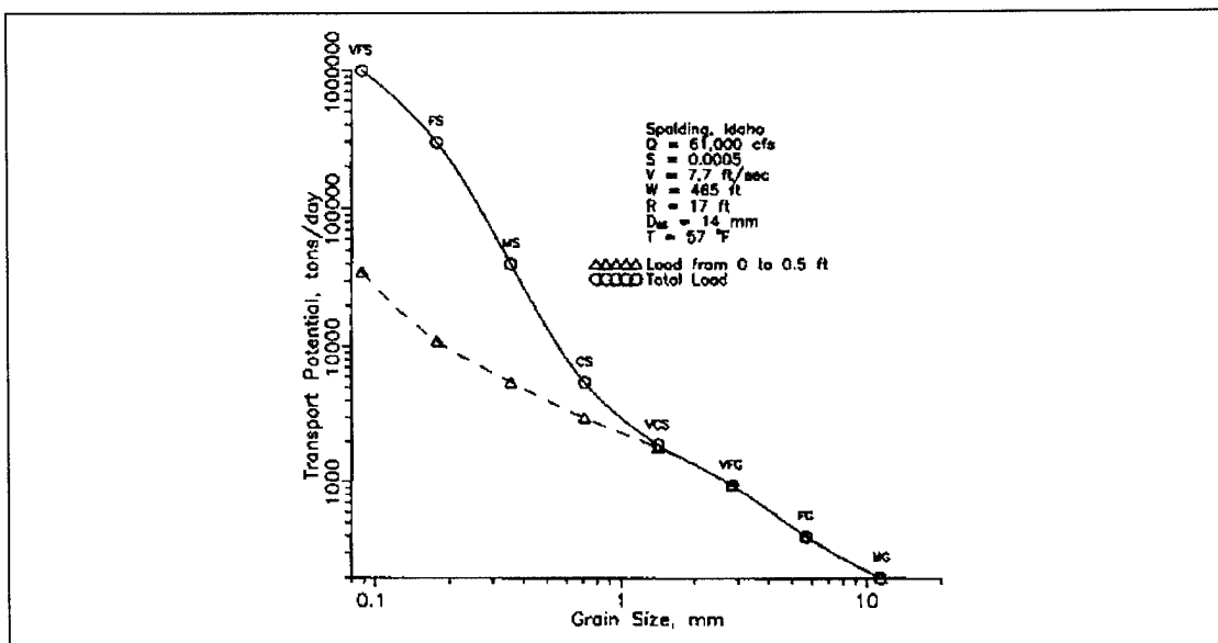
Figure 7-11. Variation of sediment transport with grain size
