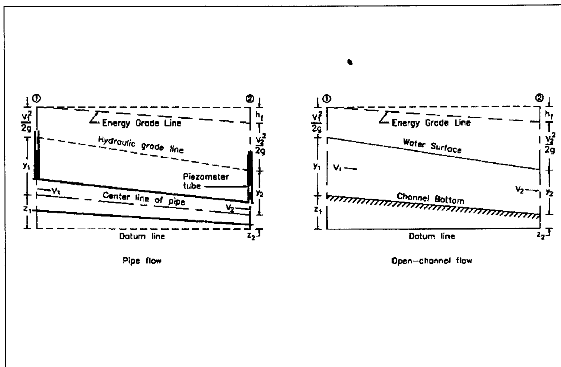
Figure 2-1. Comparison between pipe flow and open-channel flow
