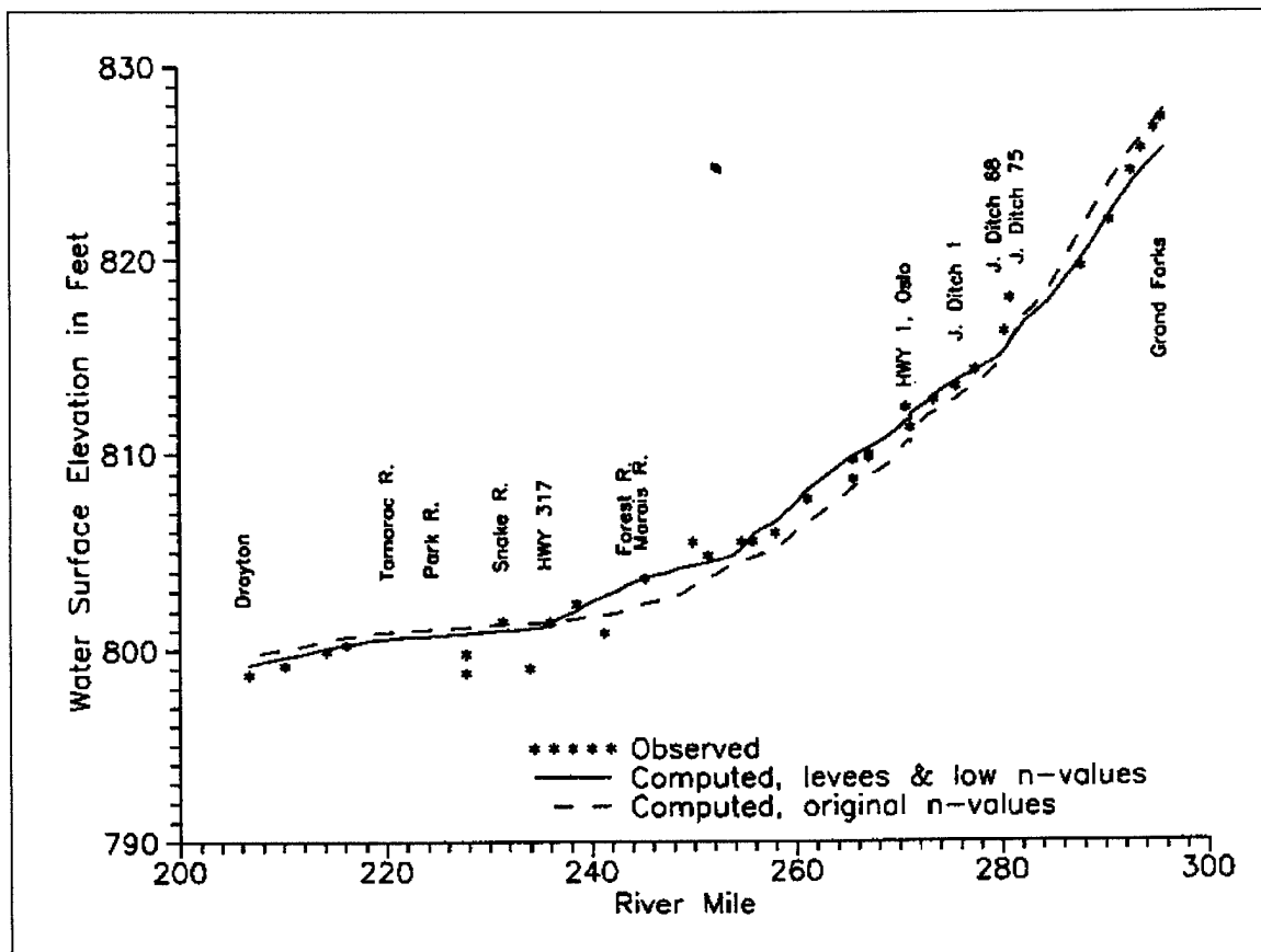
Figure 3-3. Profile calibration to high water marks
