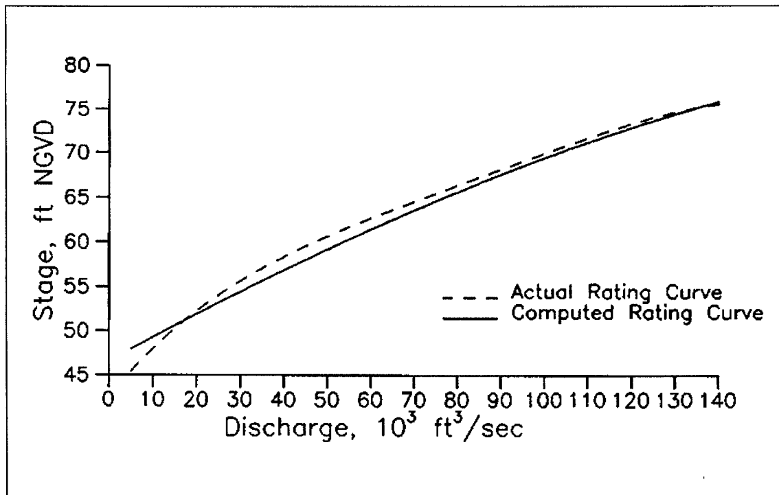
Figure 7-12. Reconstituting the stage-discharge rating curve
