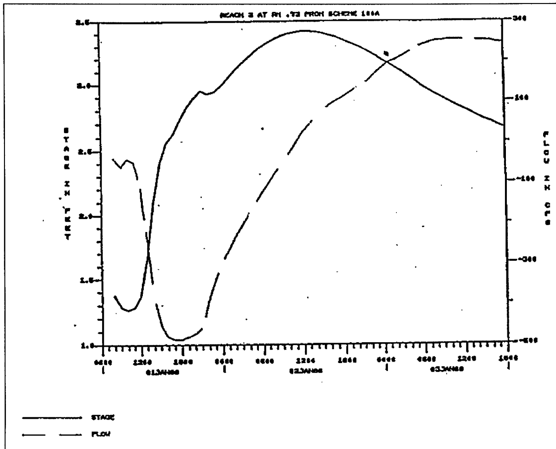
Figure 5-1. Looped rating curve induced by backwater
