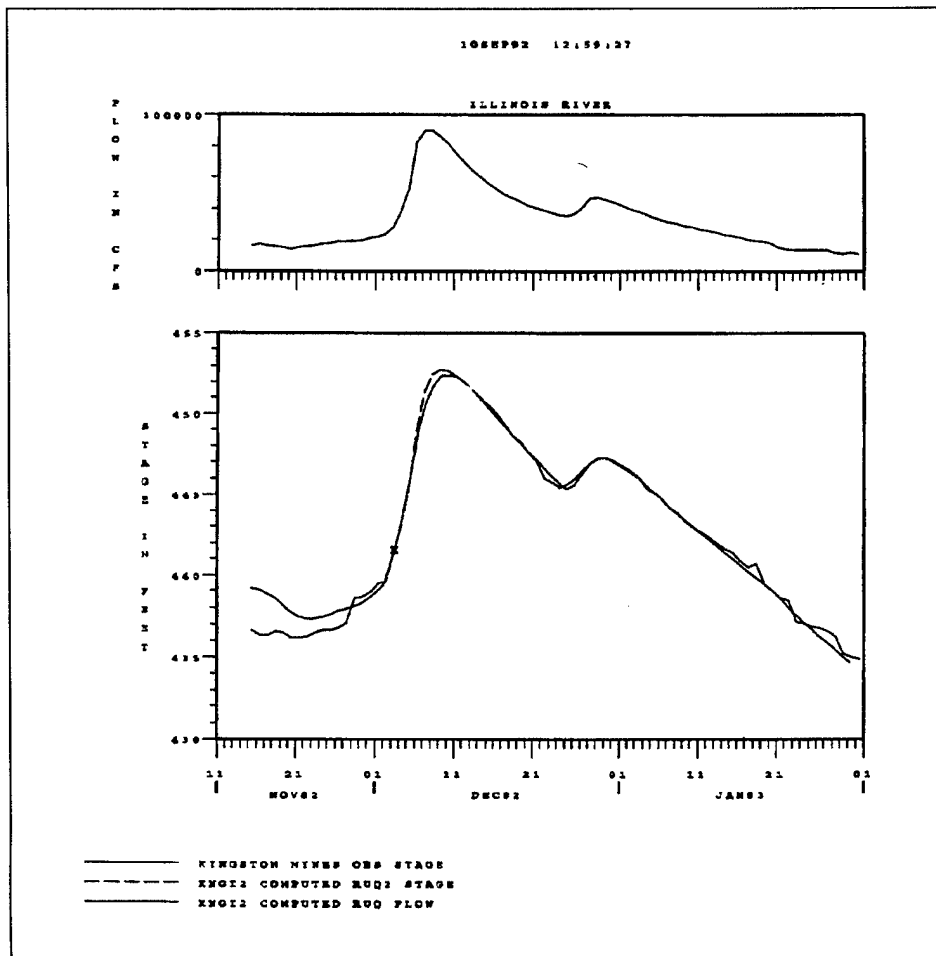
Figure 5-7. Simulation of the Illinois River at Kingston Mines including 2,579 square miles of unged drainage
