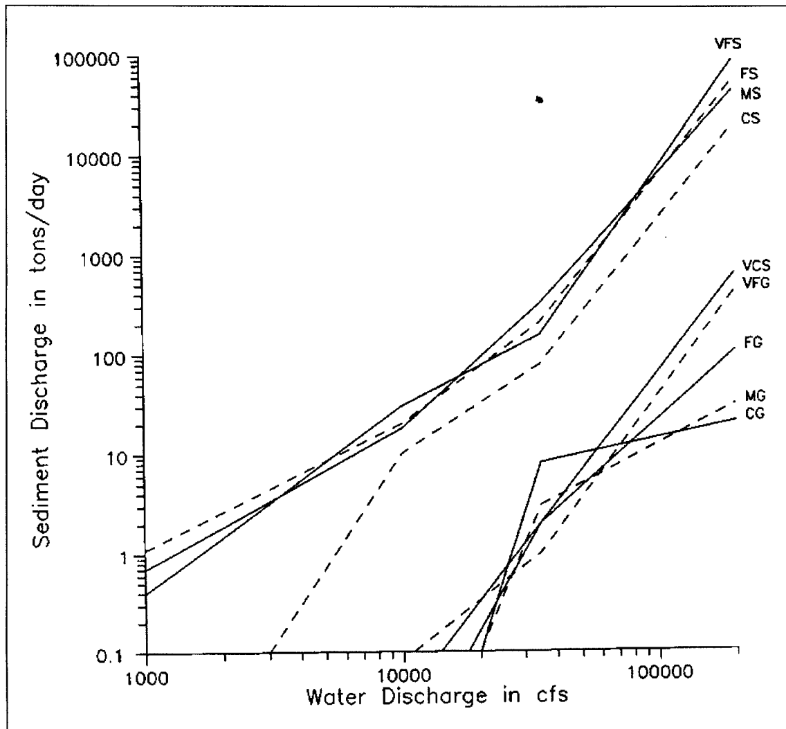
Figure 7-9. Sediment load curves
