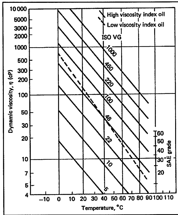
Figure 10-2. Typical viscosity/temperature characteristics of mineral oils (Reference: Neale, M. J., Lubrication: A Tribology Handbook. Butterworth-Heinemann Ltd, Oxford, England)
