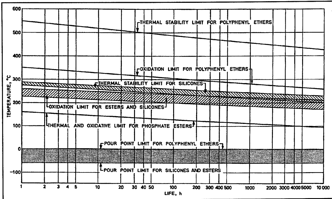
Figure 12-2. Temperature limits for some synthetic oils (Reference: Neale, M.J., Lubrication: A Tribology Handbook. Butterworth-Heinemann Ltd., Oxford, England)
