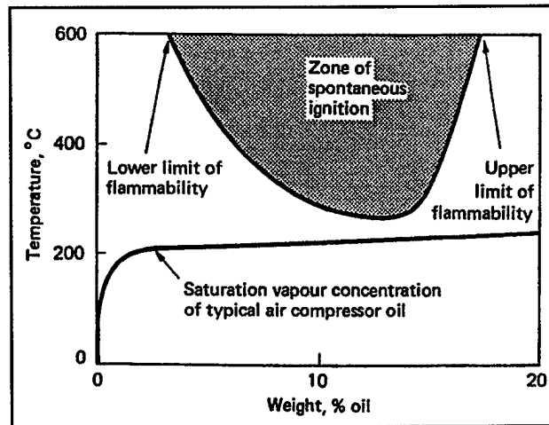
Figure 12-6. Spontaneous ignition limits for mineral oil vapor air mixtures at atmospheric pressure (Reference: Neale, M. J., Lubrication: A Tribology Handbook . Butterworth-Heinemann Ltd., Oxford, England)
