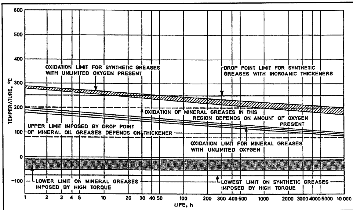
Figure 12-3. Temperature limits for greases (Reference: Neale, M.J., Lubrication: A Tribology Handbook. Butterworth-Heinemann Ltd., Oxford, England)
