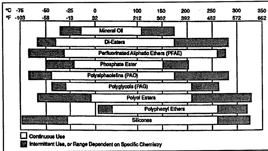
12-4. Base oil temperature limits (Reference: Booser, R.E., Reprinted with permission from CRC Handbook of Lubrication (Theory and Practice of Tribology); Volume II Theory and Design, Copyright CRC Press, Boca Raton, Florida)
