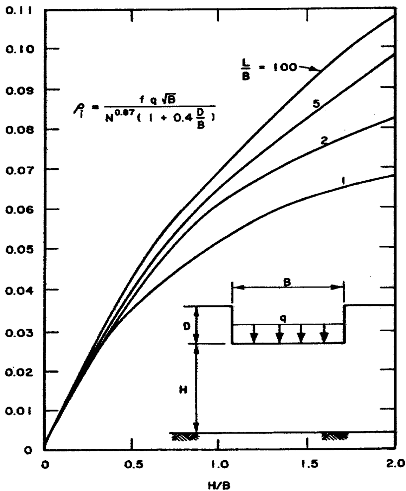
Figure 3-2. Settlement from the standard penetration test (Data from item 60)
