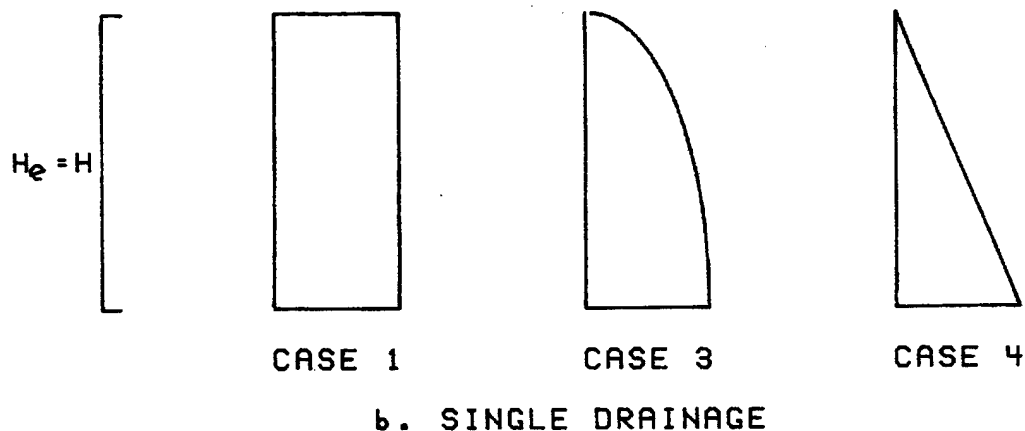
Figure 3-16. Example distributions of excess pore water pressure for double and single drainage. H is the actual stratum thickness and H_e is the equivalent height.
