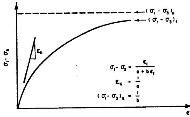
a. HYPERBOLIC RELATIONSHIP
