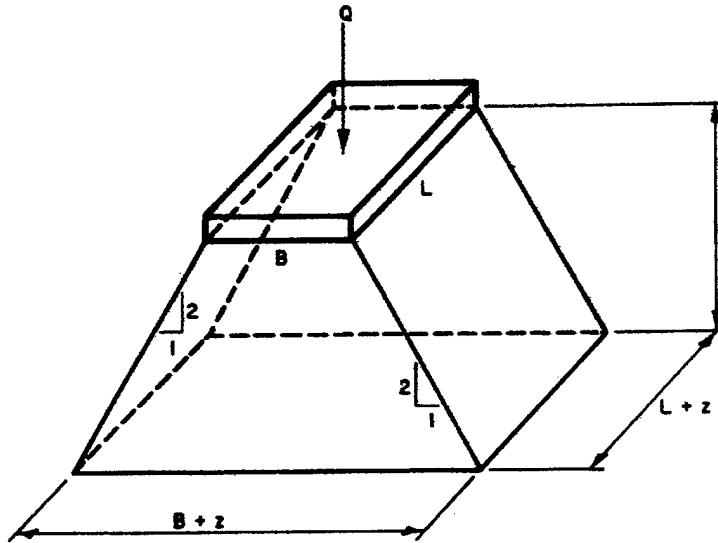
Figure C-1. Approximate stress distribution by the 2:1 method
