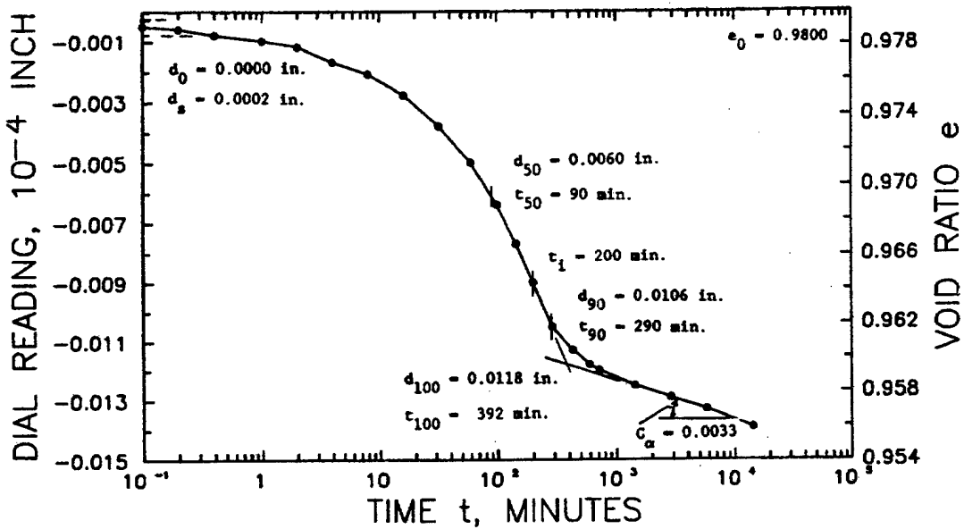
a. VOID RATIO-LOGARITHM TIME
