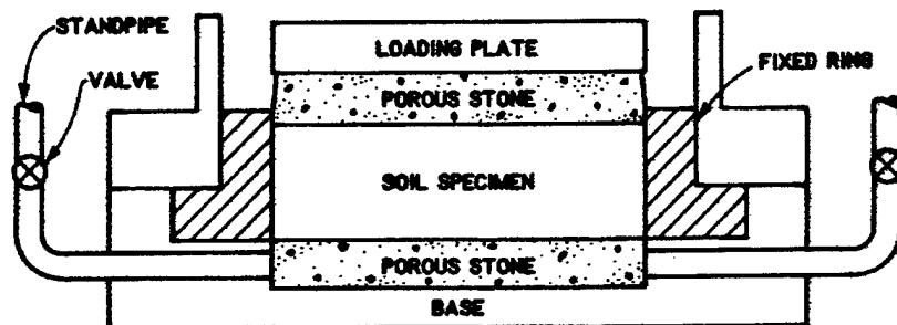
a. FIXED-RING CONSOLIDOMETER
