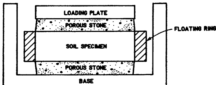
b. FLOATING-RING CONSOLIDOMETER
