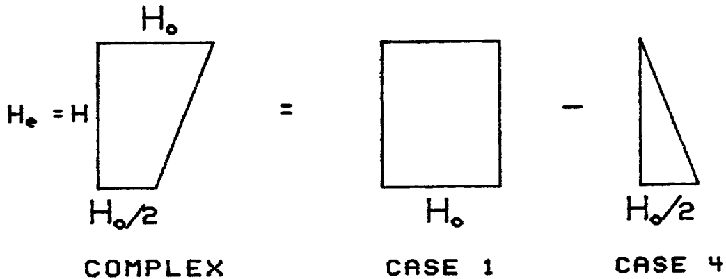
Figure 3-19. Example complex excess pore water pressure distributions
