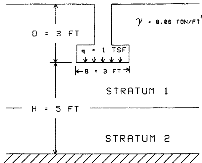
Figure 5-6. Illustration of footing for calculating settlement on collapsible soil
