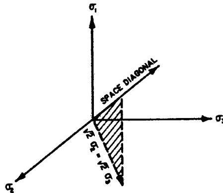
a. THE TRIAXIAL PLANE
