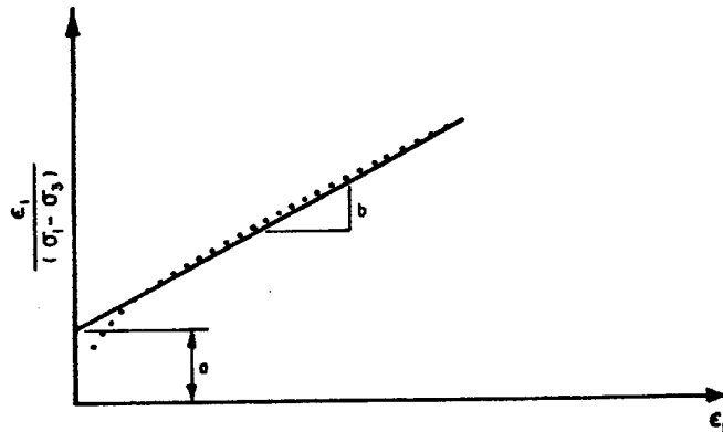
b. EVALUATION OF HYPERBOLIC PARAMETERS a, b
