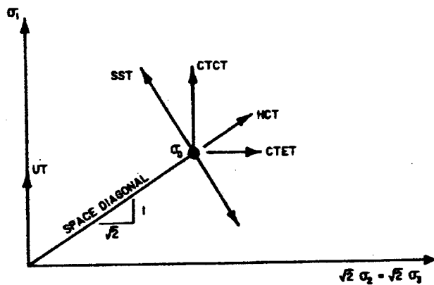
b. STRESS PATHS
