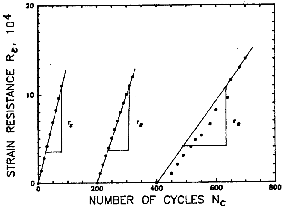
b. STRAIN RESISTANCE VERSUS NUMBER OF CYCLES
