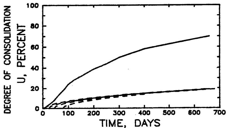
b. DEGREE OF CONSOLIDATION
