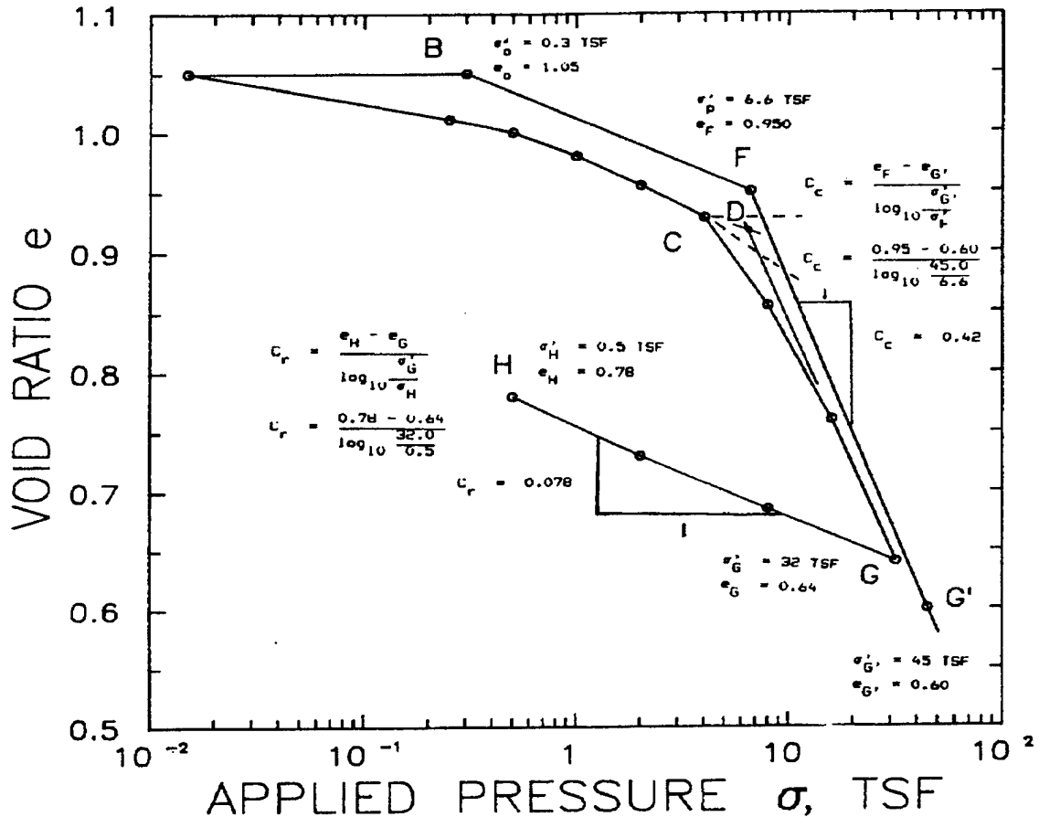
Figure 3-13. Example void ratio - logarithm pressure relationship.
