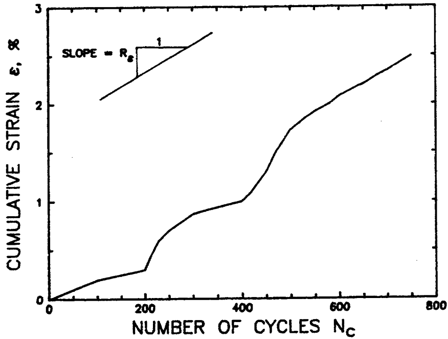
a. CUMULATIVE STRAIN VERSUS NUMBER OF CYCLES
