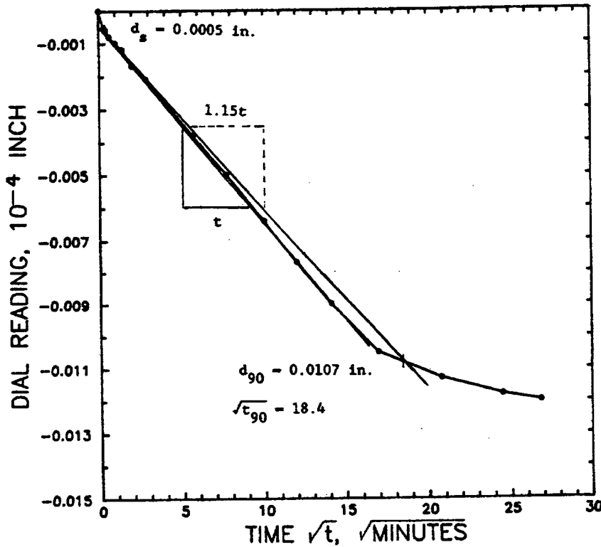
b. DISPLACEMENT-SQUARE ROOT TIME
