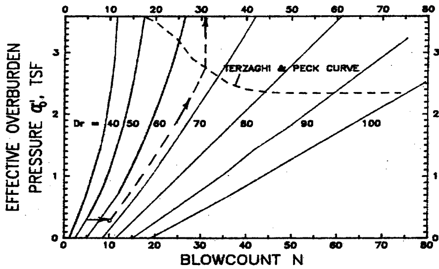
a. ADJUSTED BLOWCOUNT FROM N AND \sigma'_0
