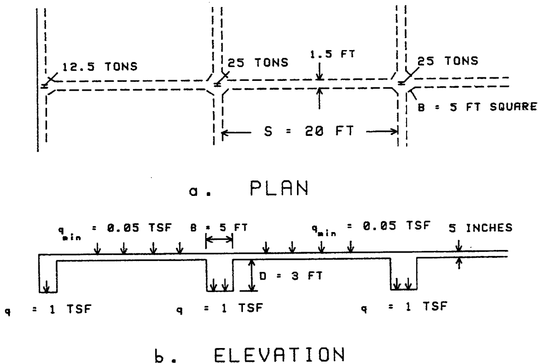
Figure 5-2. Plan and elevation of stiffened mat in expansive soil
