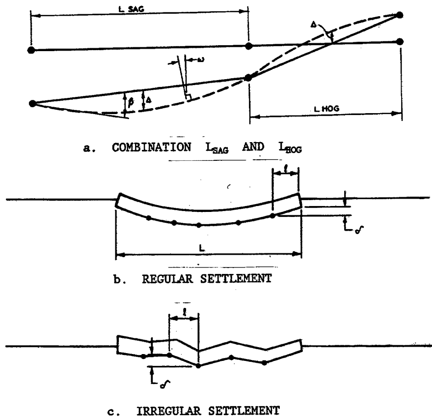
Figure 2-1. Schematic illustration of angular distortion \beta = \delta/l and deflection ratio \Delta/L for settling (sagging) and heaving (hogging) profiles
