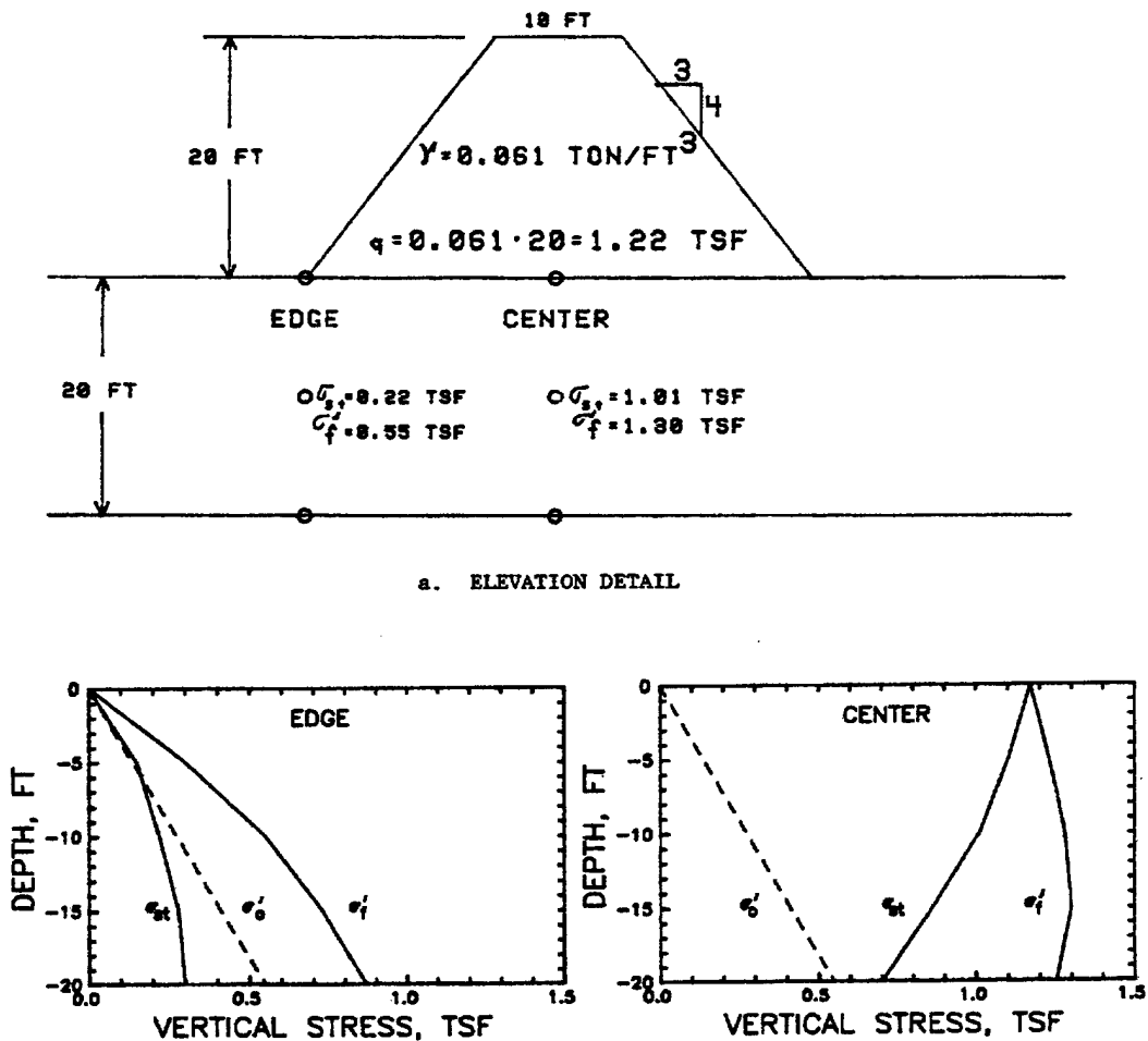
b. VERTICAL STRESS DISTRIBUTION
