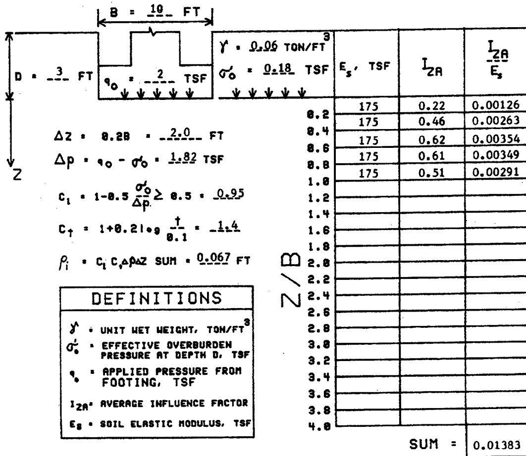
Figure 3-6. Estimation of immediate settlement by Schmertmann's method
