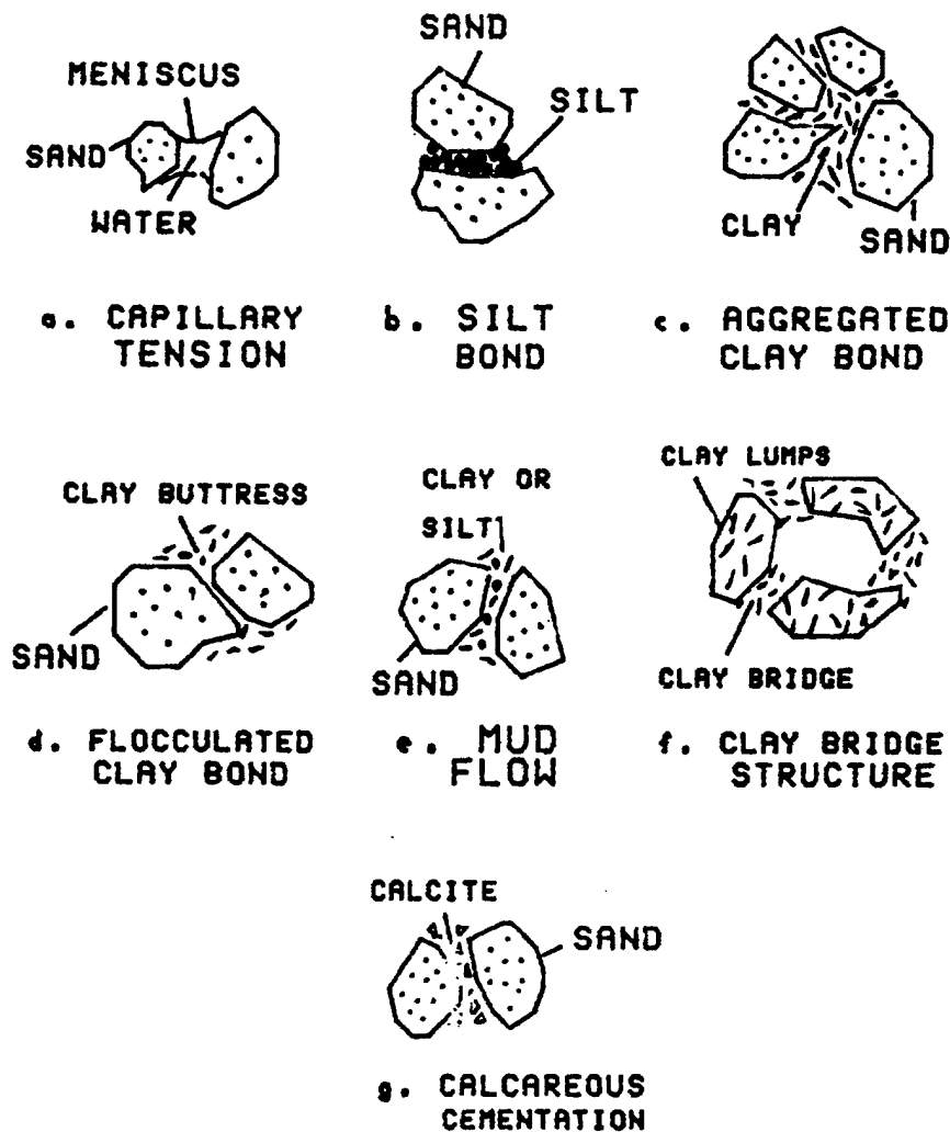
Figure 5-4. Mechanisms for collapse of loose, bulky grains
