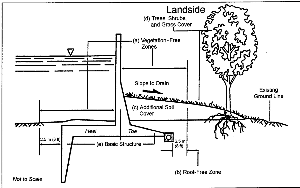
Figure 3-1. Inverted T-type floodwall showing (a) vegetation-free zone, (b) root-free zone (vertical joint occurring at section), (c) additional soil cover, (d) landscape planting of trees, shrubs, and grass, and (e) basic structure
