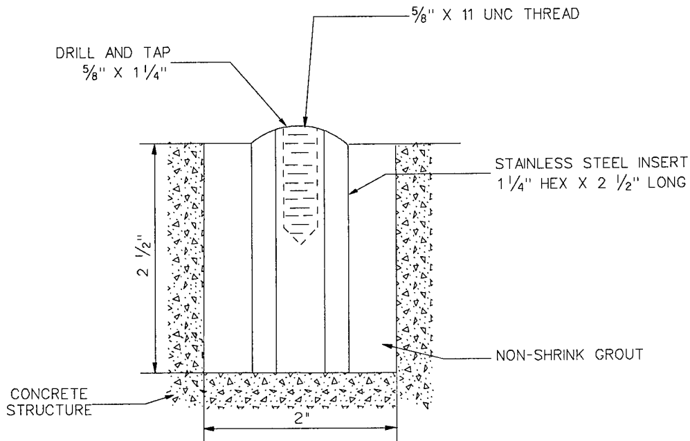
Figure 4-4. Structure insert
