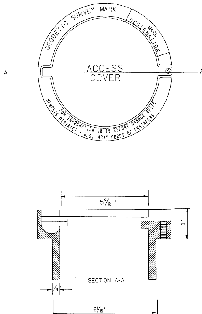
Figure 3-9. Standard access cover
