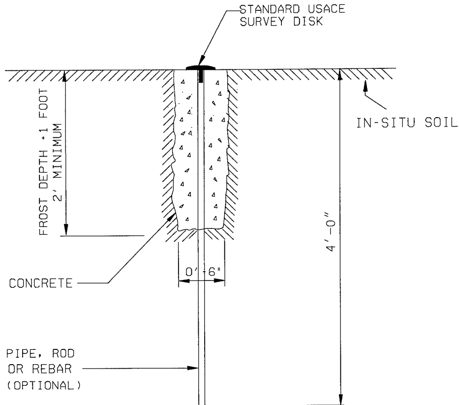
Figure 3-8. Type G monument - disk in cast-in-place concrete
