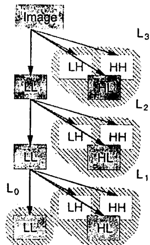
Figure A1. Mallat Decomposition. (After Taubman [2])
