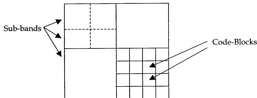
Figure A3. Sub-band code-blocks.
