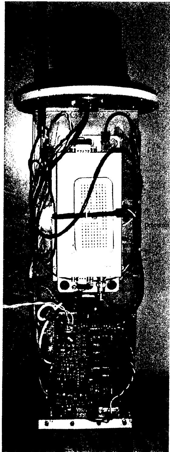
Figure 1.17: Surface electronics chassis: SIM, accelerometer, and Orbcomm unit.
