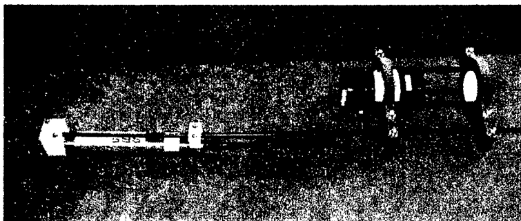
Figure 1.11: a-Beta and SBE-44 clamped on mooring wire.
