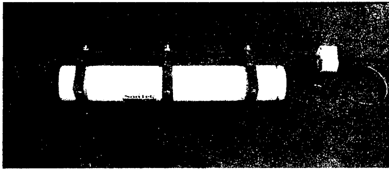
Figure 1.12: Argonaut-MD with inductive cable coupler clamped on mooring wire.
