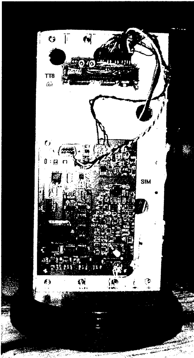
Figure 1.19: Subsurface electronics chassis: TT8V2 controller and SIM.
