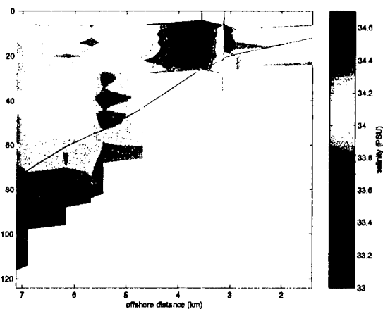
Figure 2.7: Contours of salinity along the same section as in figure 2.6.
