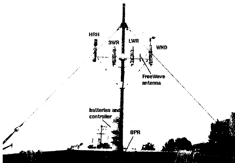
Figure 1.14: Bow mast of RV New Horizon instrumented with ASIMET modules.
