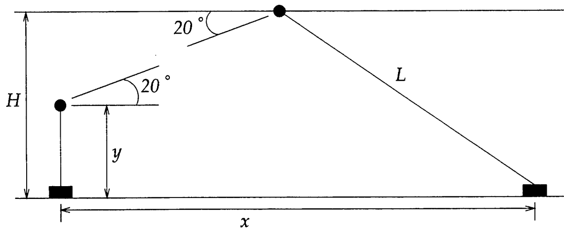
Figure 1.15: Mooring geometry dictated by the UAM transducer beam pattern.
