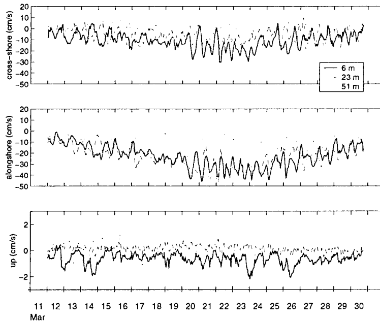
Figure 2.24: Hourly averaged cross-shore, alongshore, and up currents at 6 m, 23 m, and 51 m depths. Alongshore currents are positive upcoast, cross-shore currents are positive oncoast.
