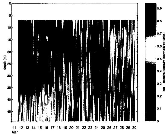
Figure 2.13: Integrated spectral energy above 48 CPD in the salinity data from the mooring line SBE-37s.
