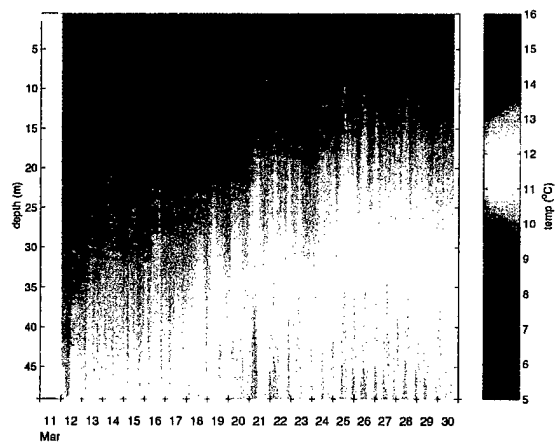
Figure 2.4: Contours of temperature from the ASIMET SBE-37, seven mooring line SBE-37s, and thirteen SBE-39 instruments.
