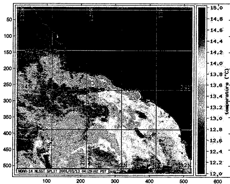
Figure 2.15: AVHRR sea surface temperature acquired at the CoastWatch West Regional Node on 13 March 2001 at 04:29 local.
