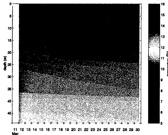
Figure 2.23: PWP modeled temperature contours.
