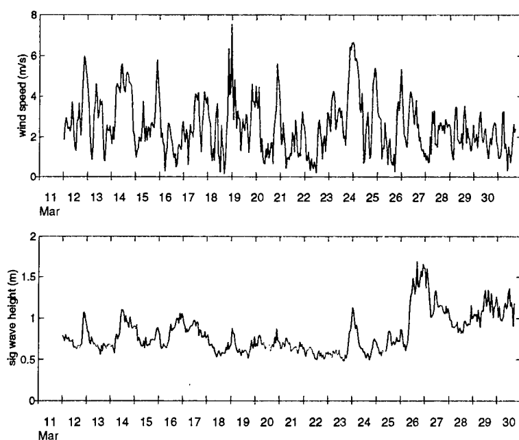
Figure 2.20: Hourly averaged wind speed (from the ASIMET system) and significant wave height from the tri-axial accelerometer on the surface buoy.
