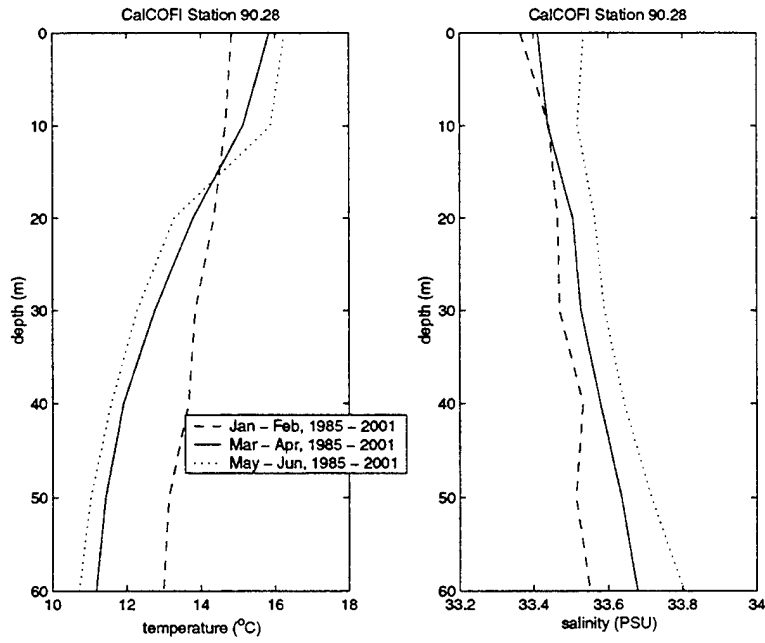
Figure 2.1: January–February, March–April, and May–June temperature and salinity profiles at CalCOFI station 90.28 (33.48°N, 117.77°W averaged over 1985–2001).
