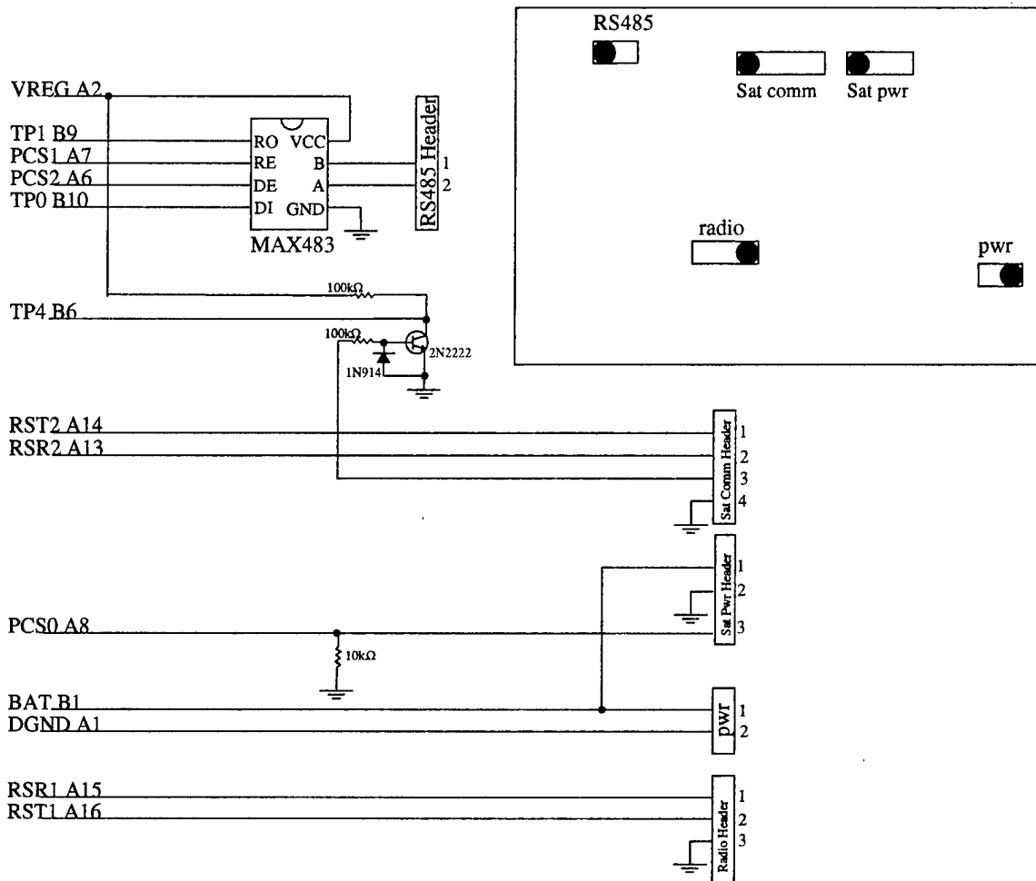
Figure 1.22: Electrical schematic and layout of the TT8 bow mast controller interface board.
