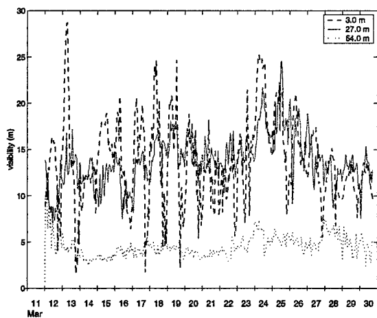
Figure 2.25: Visibility at the three a-Beta instruments using the 2/K formulation. Hourly K_L values were computed from the single ten second average raw transmission value returned via telemetry.
