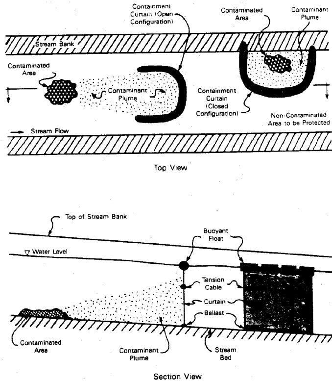
Figure I-1. Plume containment (U.S. EPA, 2000).
