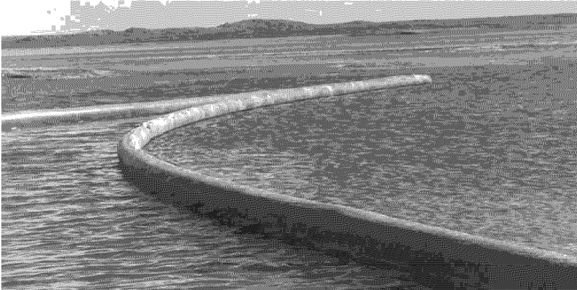
Figure 4-10. Chevron booming.
