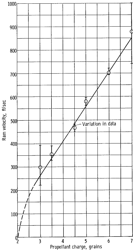
Figure 5. - Ram velocity as function of propellant charge. Ram weight, 22.5 grams; propellant, Bulseye powder.
