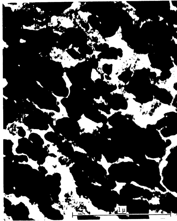
Figure 21. - Electron micrograph of nickel - 5 volume percent alumina wet blended in SMD colloid mill and hydrogen cleaned for 2 hours at 800° F. Blend specimen was vacuum infiltrated with resin and sliced in ultramicrotome. Original magnification, X58 000.
