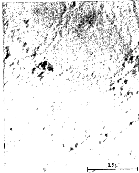
(b) Blend 8 (tungsten - 2 volume percent thoria) produced by arc-vaporization technique and compacted with sleeve-and-plunger method. Original magnification, X74 000.
