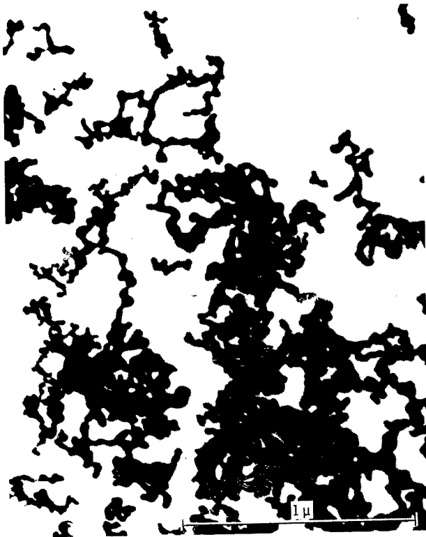
Figure 20. - Electron micrograph of blend specimen of tungsten - 5 volume percent thoria dispersed in plastic film. Original magnification, X58 000.
