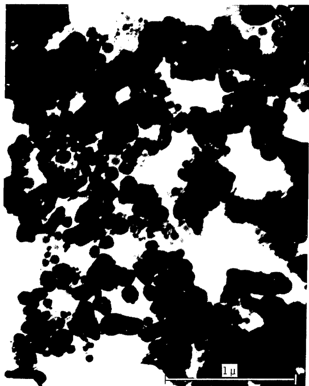
Figure 18. - Electron micrograph of preblend specimen of nickel - 8 volume percent alumina dispersed in plastic film. Original magnification, X46 000.
