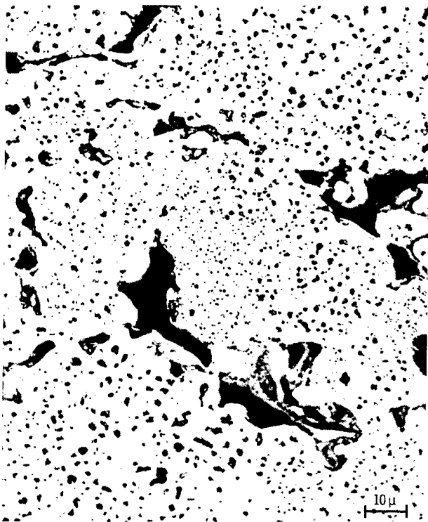
Figure 16. - Blend specimen of nickel - alumina pressed and sintered in hydrogen for 4 hours at 2000° F. Original magnification, X1000.
