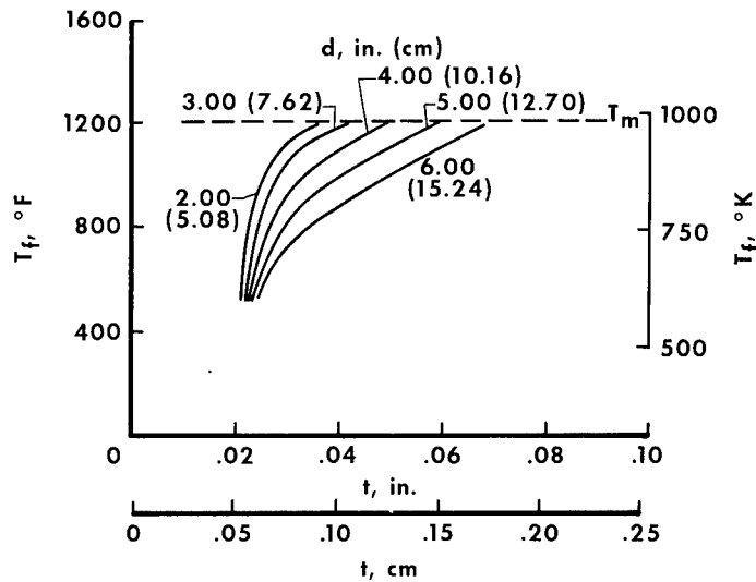
(b) SAE 4130 steel.
