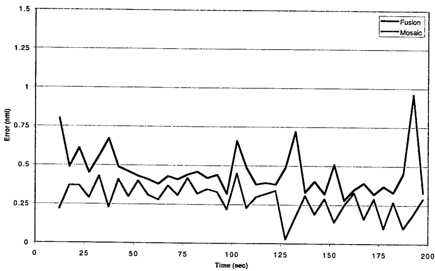
Figure 161. Outlier Test (Outlier at Time 100) - Position Error - CD2 Data - COTS C.
