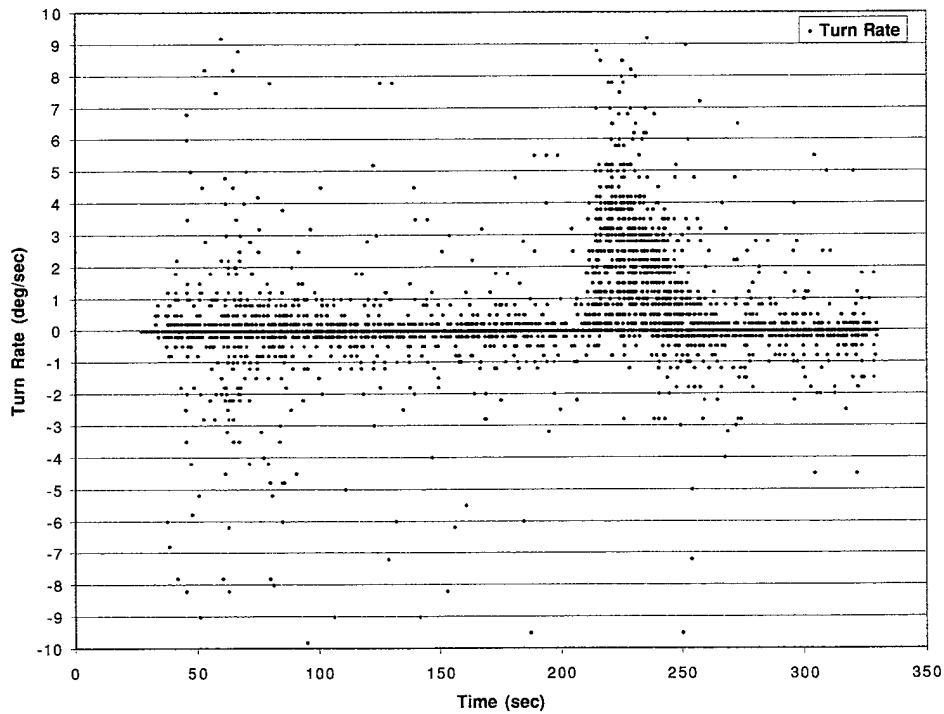
Figure 74. Computed Turn Rate Values - Turn 200-230 Seconds @ 3 Deg/Sec - Mode S Data - COTS D.
