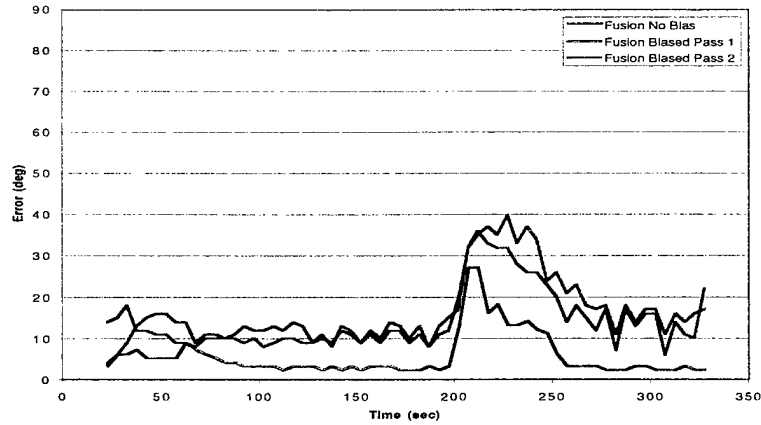
Figure 78. Bias Adaptation Test (1 Hour Adaptation Period) - Turn 200-230 Seconds - Track Angle Error - Mode S Data - COTS A.
