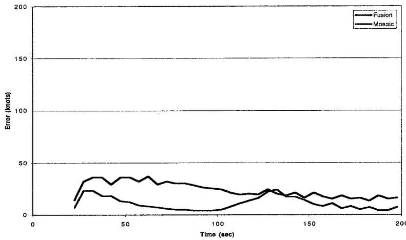
Figure 103. Sensor Hop Due to Biases Test - Sensor Change at 100 Seconds - Ground Speed Error - Mode S Data - COTS A.
