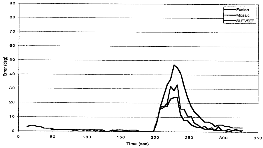
Figure 42. Turning Test (Turn 200-230 Seconds) - Track Angle Error - Mode S Data - COTS B.
