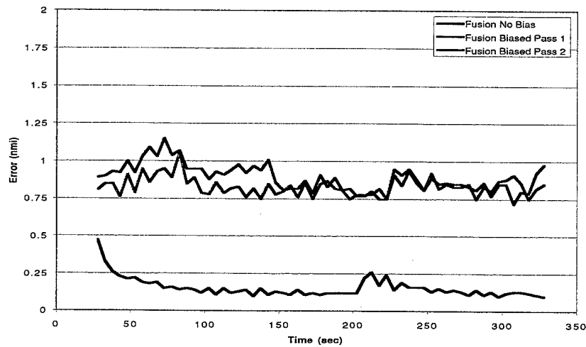
Figure 77. Bias Adaptation Test (1 Hour Adaptation Period) - Turn 200-230 Seconds - Position Error - CD2 Data - COTS A.
