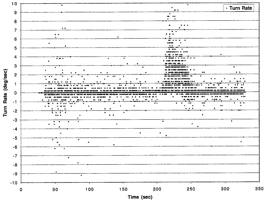
Figure 73. Computed Turn Rate Values - Turn 200-230 Seconds @ 3 Deg/Sec - CD2 Data - COTS D.
