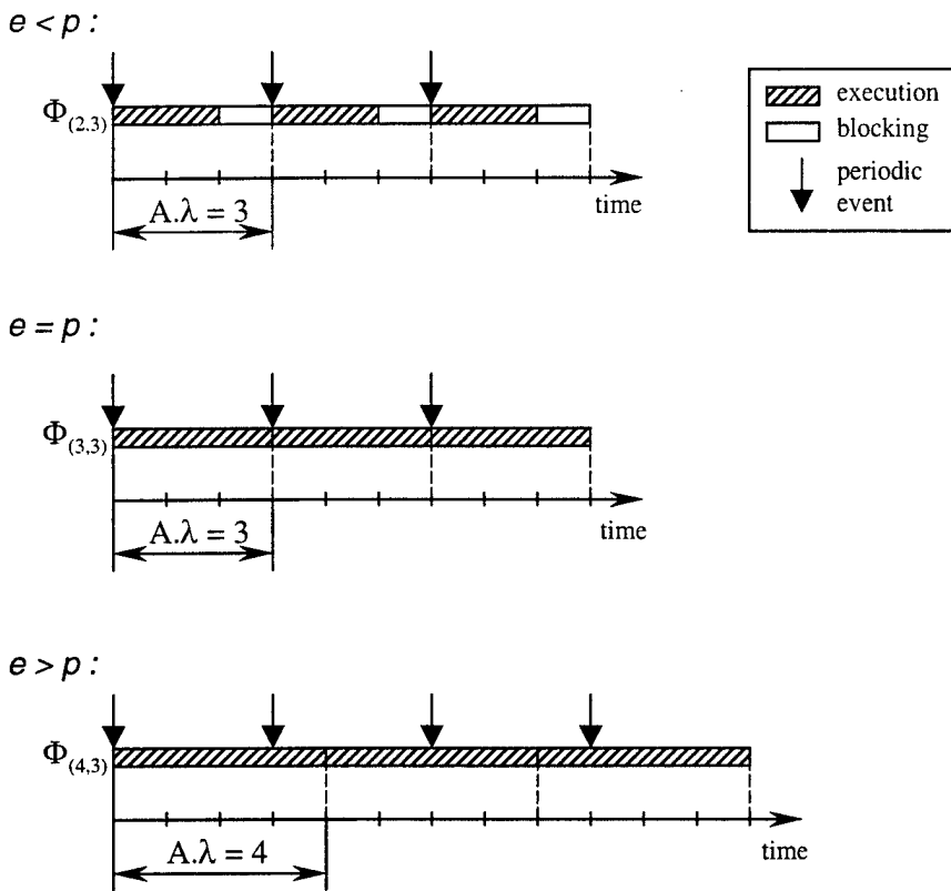
Figure 10: Timeline for \Phi Components with e < p , e = p , and e > p
