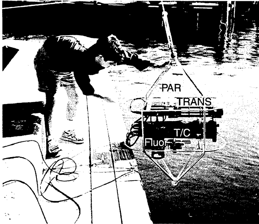
Figure 12: Photograph of WHOI Bio-Optical Unit
