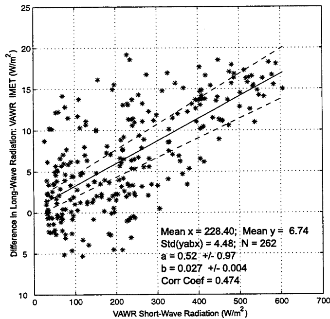
Figure 22: The difference between VAWR and IMET long-wave radiation measurements versus VAWR short-wave radiation during daytime ( SW > 25 \text{ W/m}^2 ). Only data from initial 28-day period before IMET failure occurred are shown.
