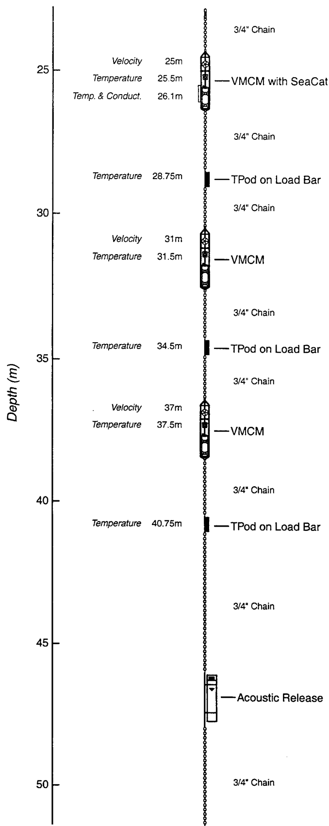
Figure 7B: Mid-section of surface mooring.
