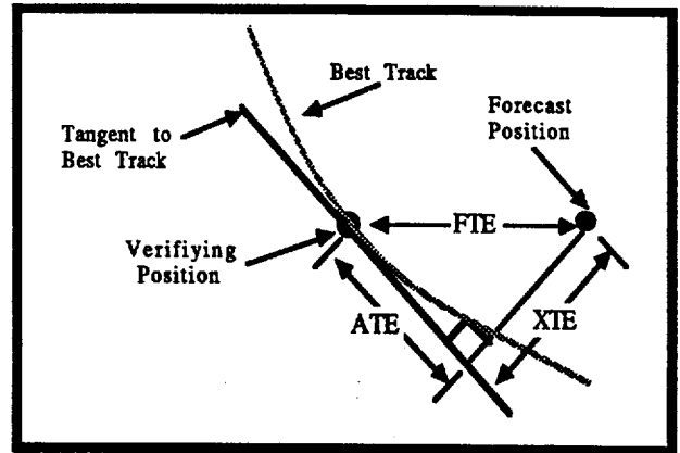
Figure 5-1. Definition of cross-track error (XTE), along-track error (ATE), and forecast track error (FTE). In this example, the XTE is positive (to the right of the Best Track) and the ATE is negative (behind or slower than the Best Track)..
