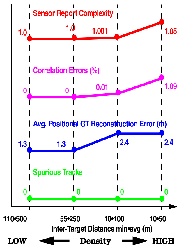
FIGURE 9. Ground Truth reconstruction performance and correlation errors are proportional to Sensor Report complexity. (Results from the Mountain Pass scenario)
