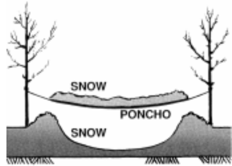
Figure 10. Design sketch of poncho and snow shelter.
