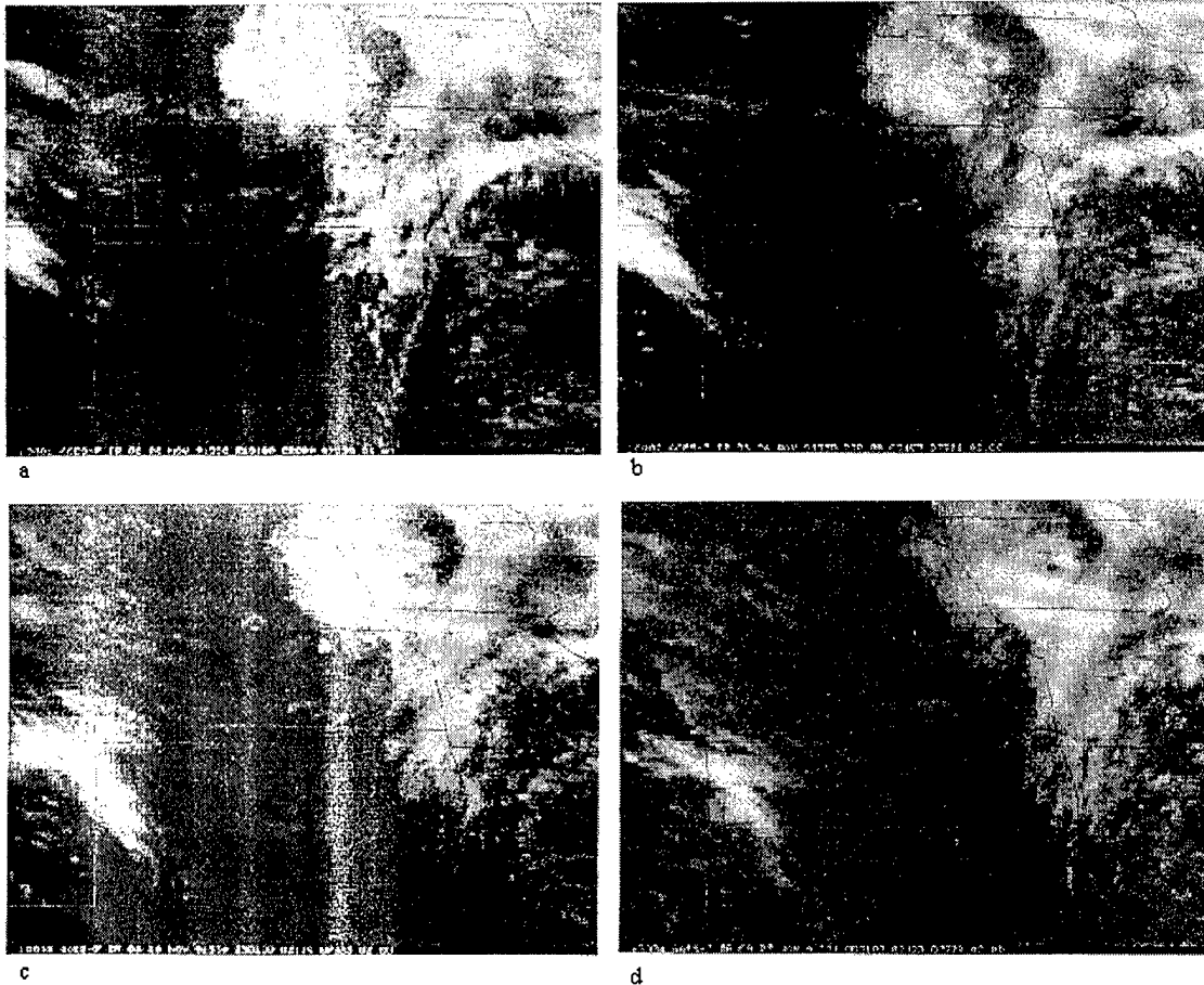
Figure 2.2: GOES-7 infrared imagery showing the progression of the 26 November 1991 cirrus event at (a) 2100 UTC 26 Nov 91; (b) 2200 UTC 26 Nov 91; (c) 2300 UTC 26 Nov 91; and (d) 0000 UTC 27 Nov 91.
