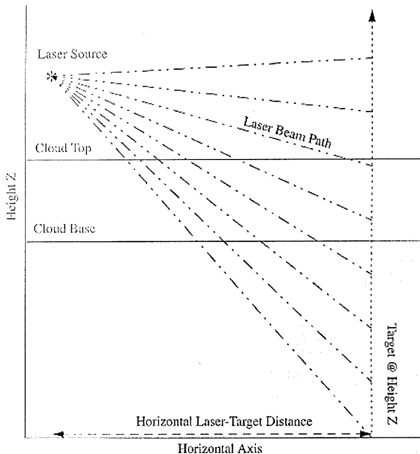
Figure 3.2: Description of a typical angle sweep laser-target geometry. Note that as the target increases in altitude below the cloud layer the path length of the beam within the cloud grows. This would be expected to cause a decrease in transmission as more cloud is in the way of the target.
