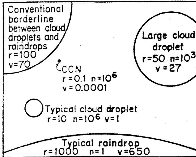
Figure B.1: Relative sizes of typical cloud and raindrops; r is the radius in micrometers, n is the number per liter of air, and v is the terminal fall speed in centimeters per second. (From McDonald, 1958)
