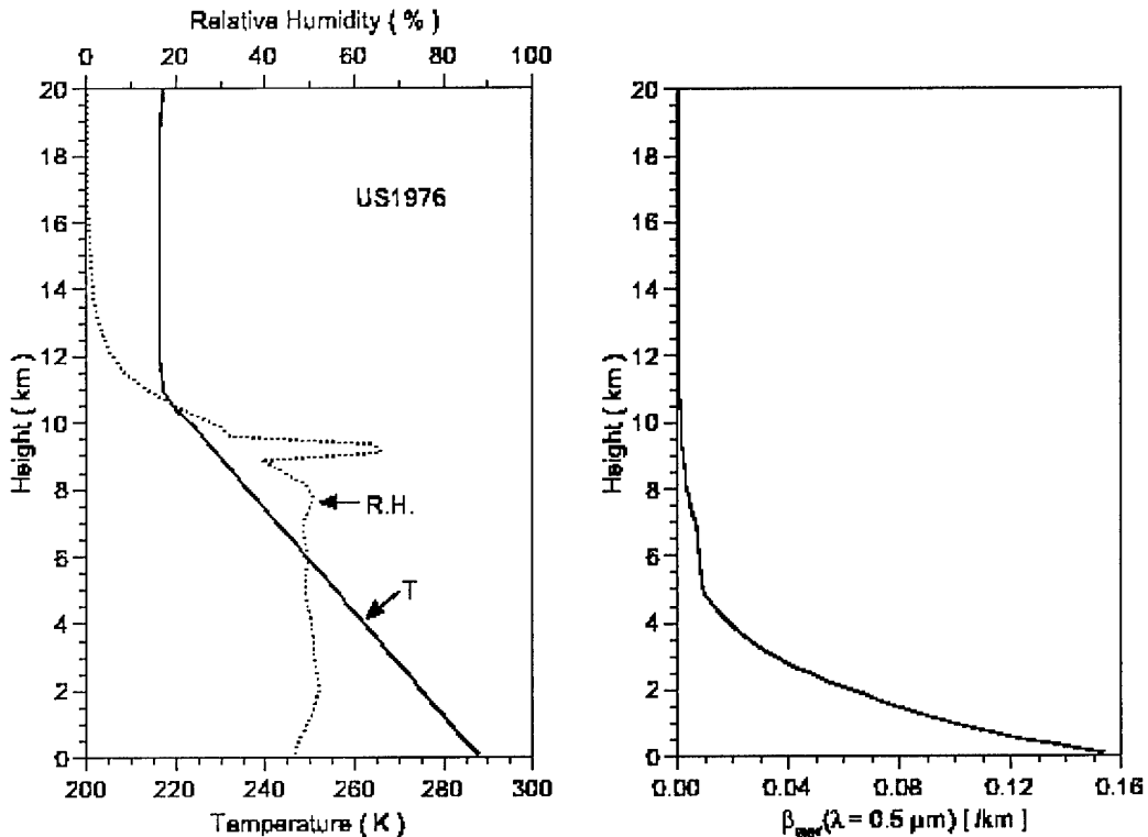
Figure 3.1: Atmospheric profile and extinction coefficient for aerosols assumed in the laser transmission computation, from Liou et al. 1999.
