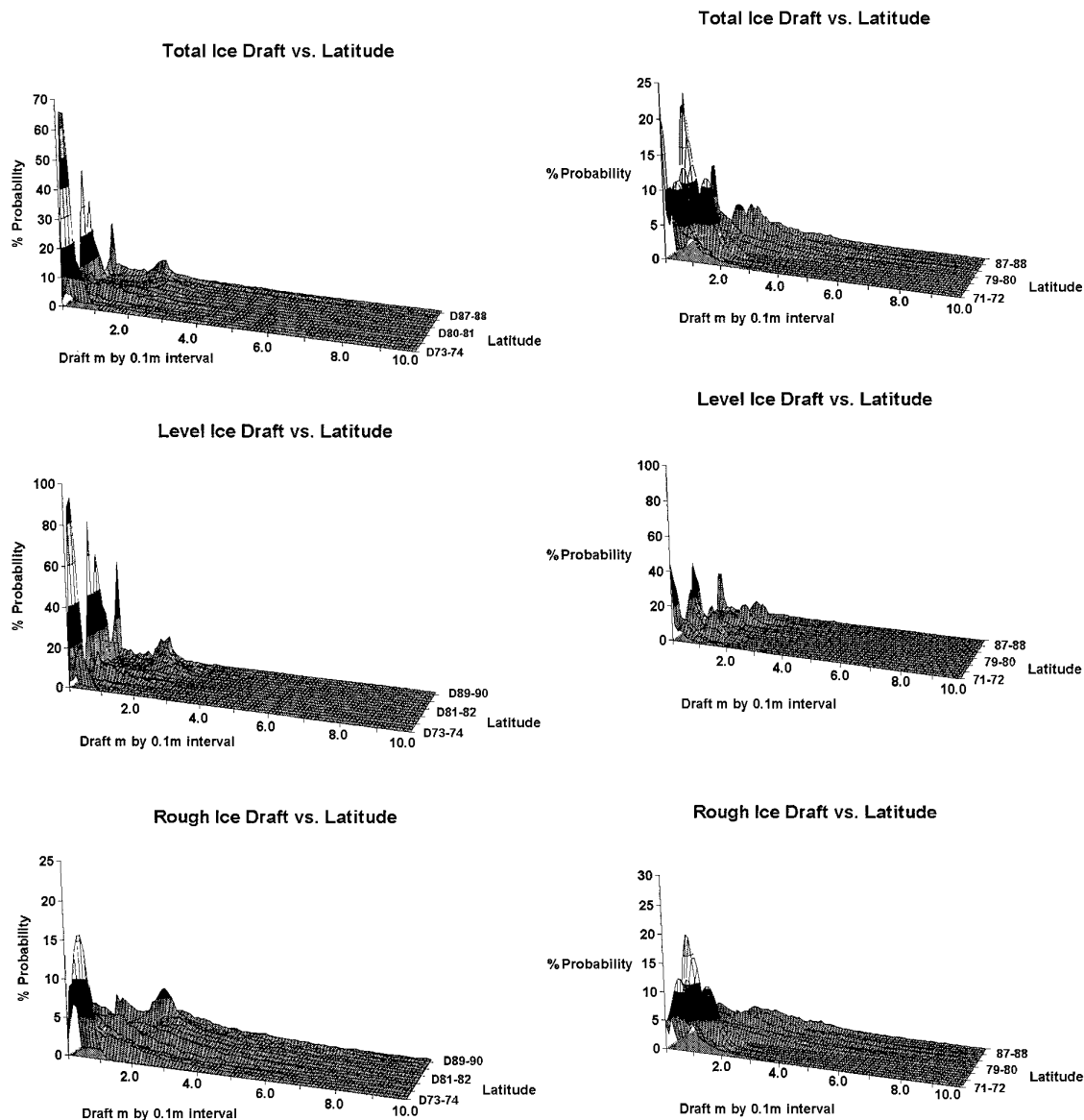
Fig. 3. Probability density functions of 1996 ice draft in 1^\circ bins plotted against latitude for westerly and easterly tracks. Top: all ice; middle: level ice only; bottom: rough ice only.
