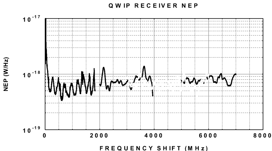
Figure 5 QWIP Heterodyne Performance Curves
