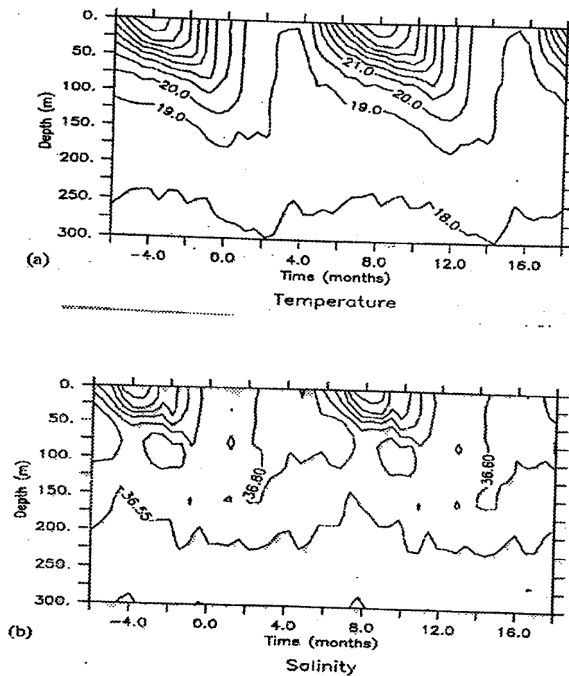
Figure 2-12: Climatological (1961-1970) seasonal cycles of (a) temperature ( ^{\circ}C ) and (b) salinity for Hydrostation S.
