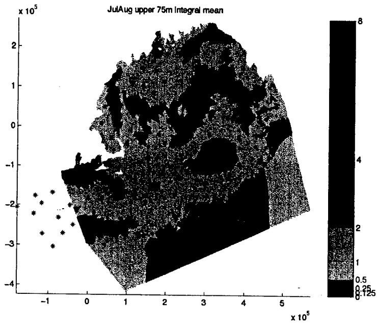
Figure 3-8: Jul-Aug map of Chl w of default case
