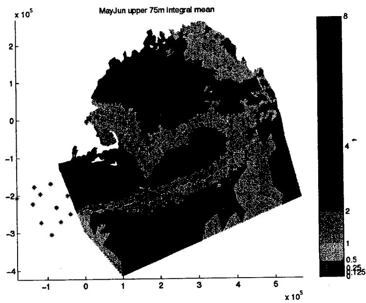
Figure 3-7: May-Jun map of Chl_w of default case
