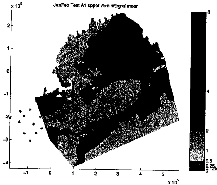
Figure 3-12: Jan-Feb map of Chl_w of case A1
