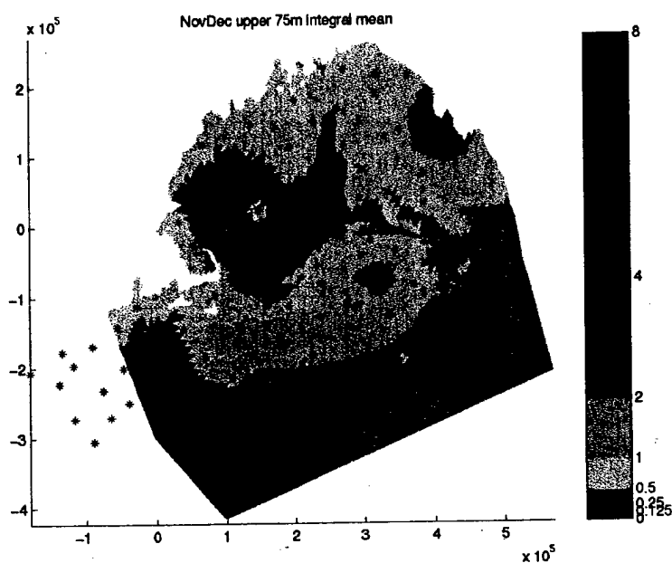
Figure 3-10: Nov-Dec map of Chl_w of default case
