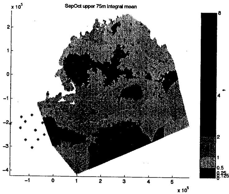
Figure 3-9: Sep-Oct map of Chl w of default case
