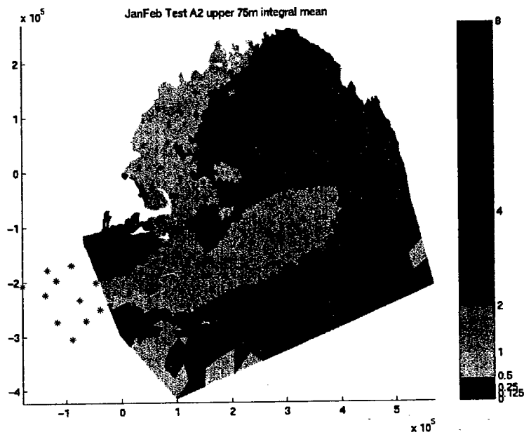
Figure 3-15: Jan-Feb map of Chl_w of case A2
