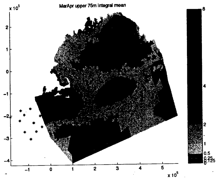
Figure 3-6: Mar-Apr map of Chl_w of default case
